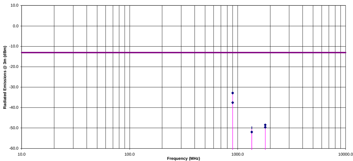
KAVAL TELECOM INC.50 50 dB Bi-Directional Amplifier, Model: BDA 1300 TX Frequency: 450 MHz Radiated Emissions Measurements at 3 Meter OFTS Ultratech Engineering Labs Inc.
