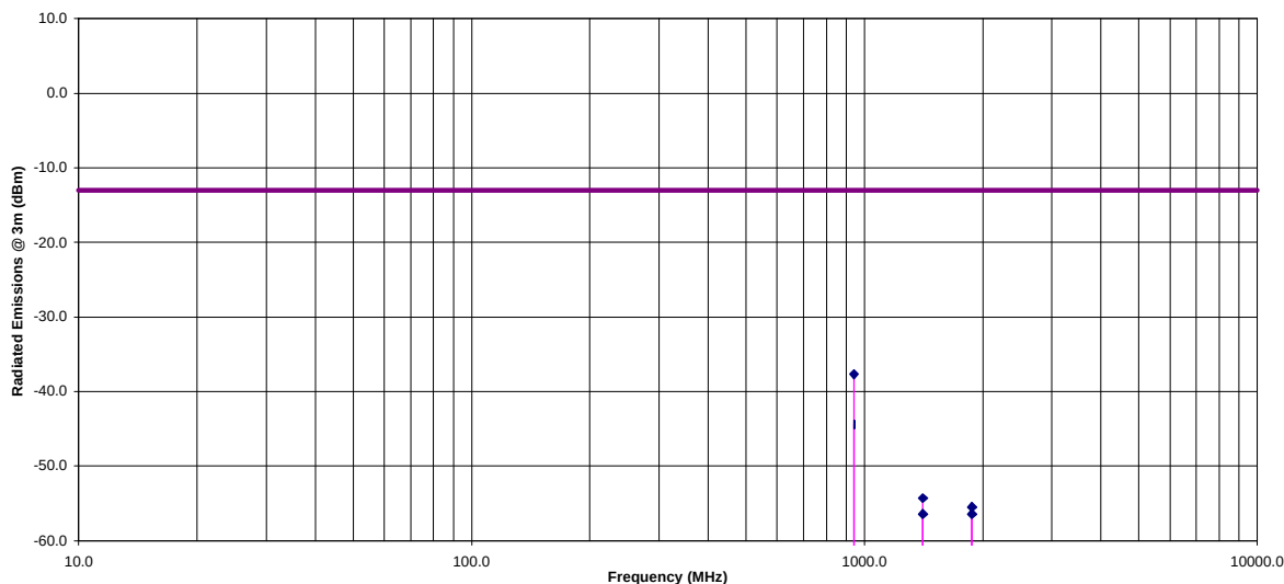
KAVAL TELECOM INC.50 50 dB Bi-Directional Amplifier, Model: BDA 1300 TX Frequency: 470 MHz Radiated Emissions Measurements at 3 Meter OFTS Ultratech Engineering Labs Inc.
