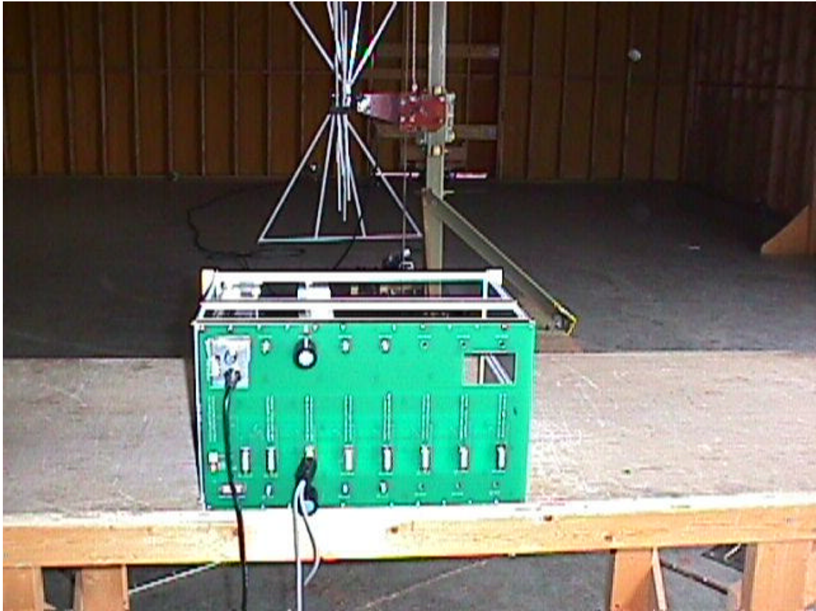
Exhibit 10 - Photograph # 1 of Radiated Emission Test Setup
