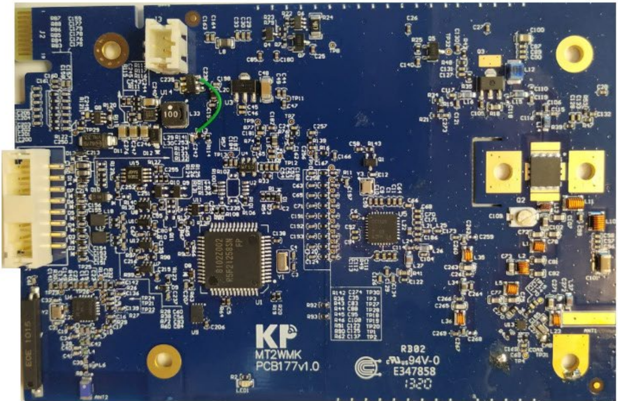
PCB Front, Shield Removed
