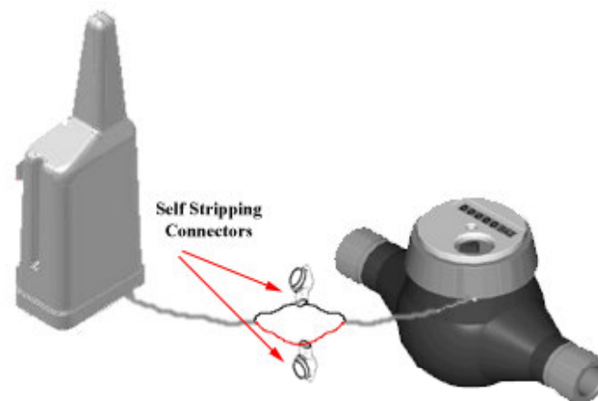
figure 4: wiring
