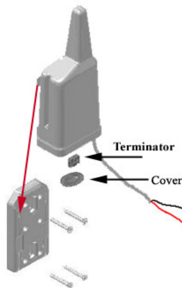
Figure 2: Wall Mounting
