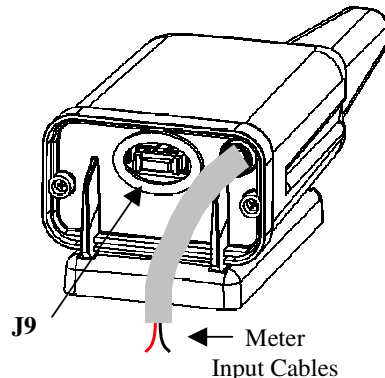
Figure 1: MTU150W™ View
