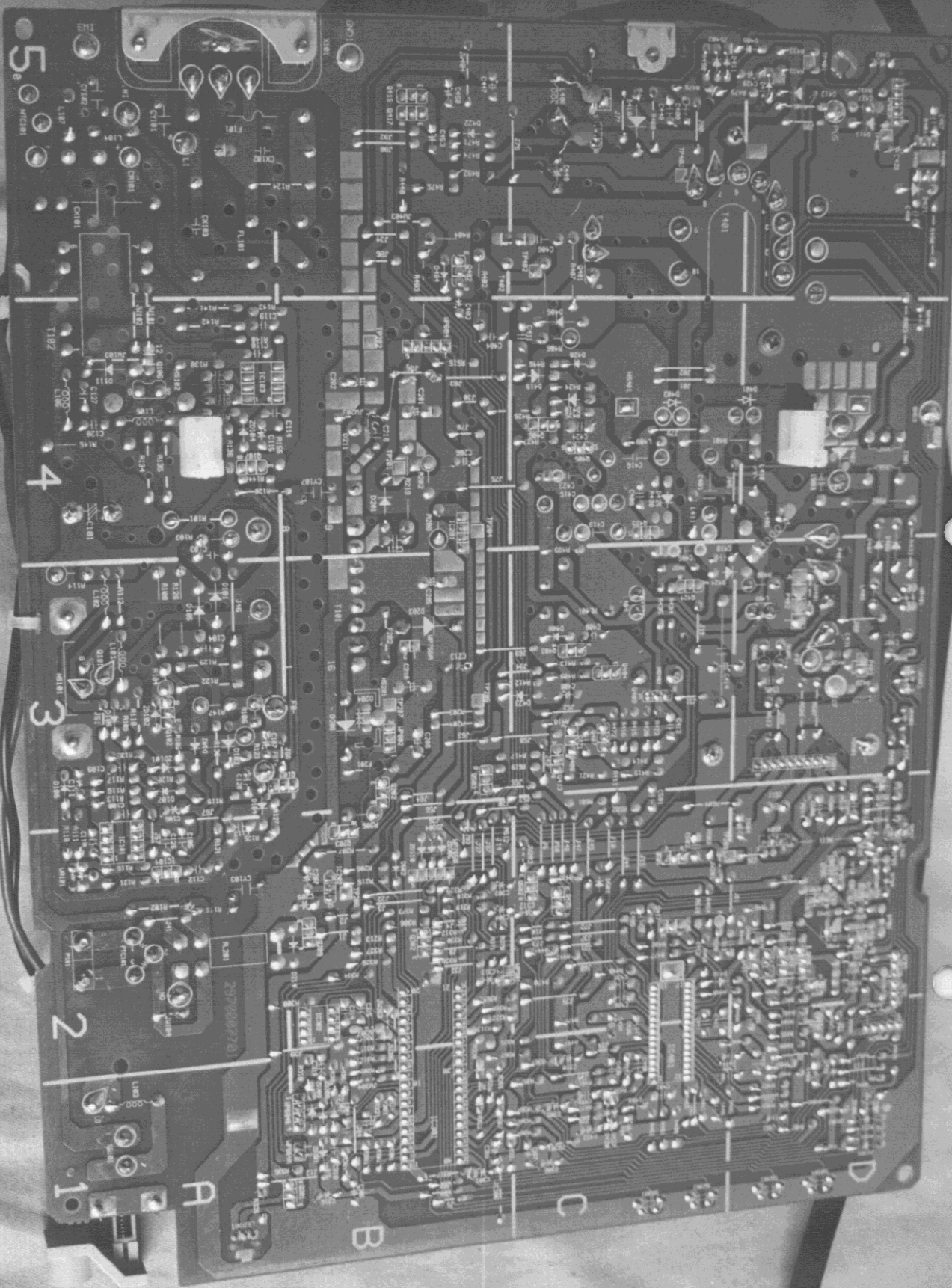
Figure 6 Main Board (Foil Side)
