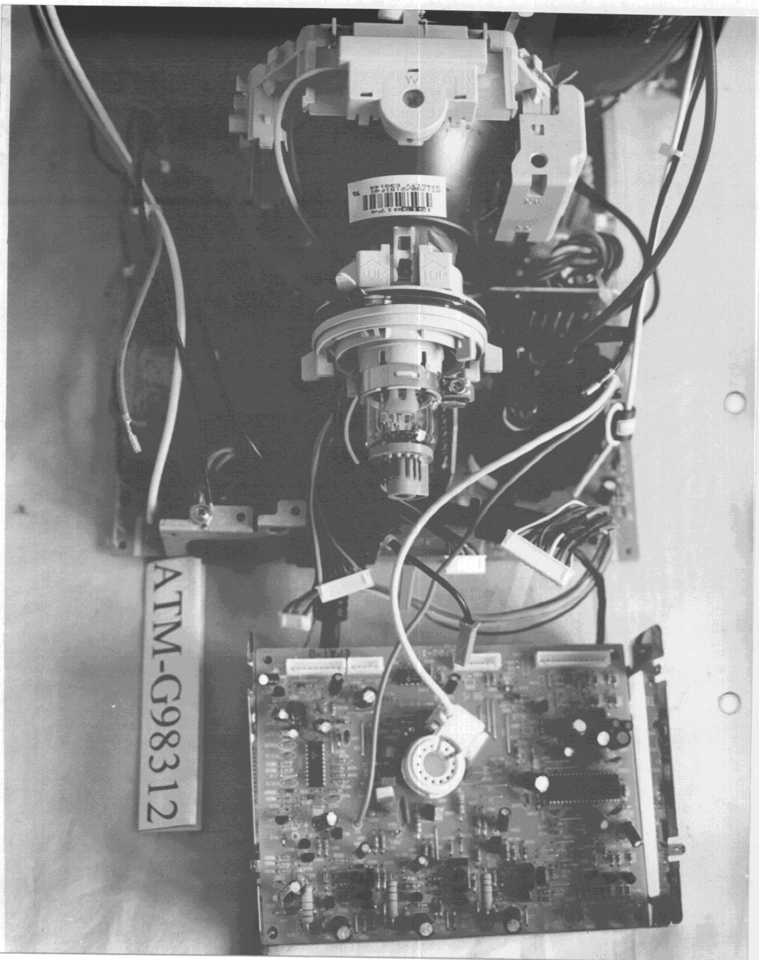
Figure 4 Internal View (Video Board)
