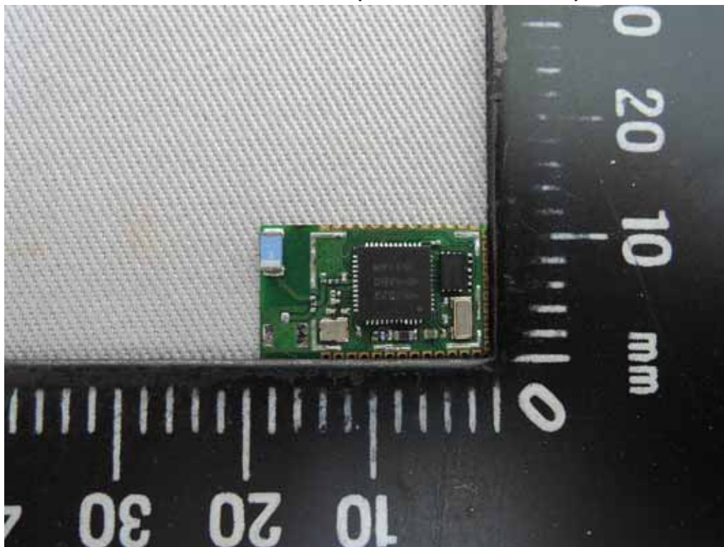
Front View of EUT (DFBM-NQ621-DT0R)
