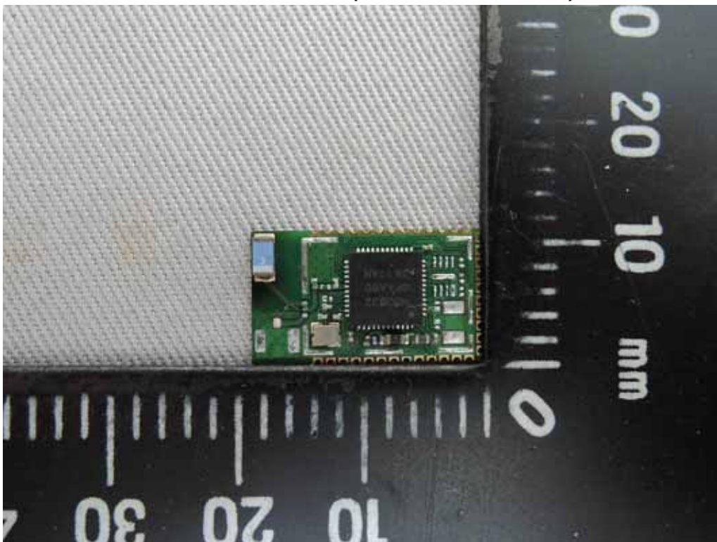
Front View of EUT (DFBM-NQ625-DT0R)
