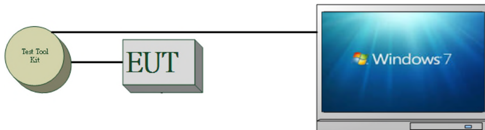
Fig. 2-1 AC Power Line Conducted Emission Configuration
