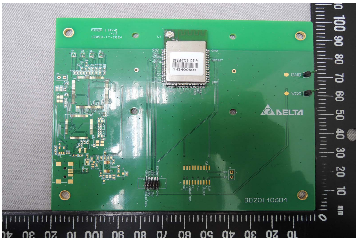
Front View of EUT (DFZM-TT211-DT0R)
