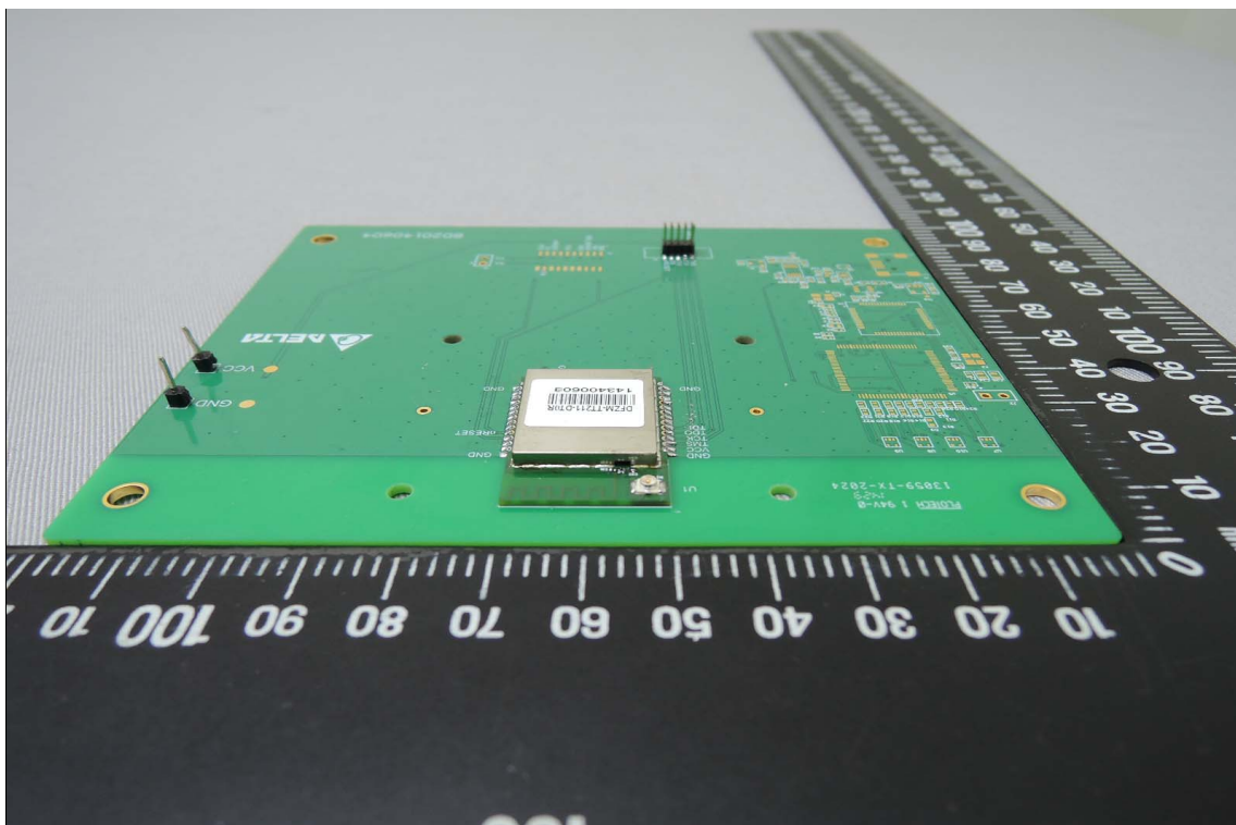
Side View of EUT – 3(DFZM-TT210-DT0R)
