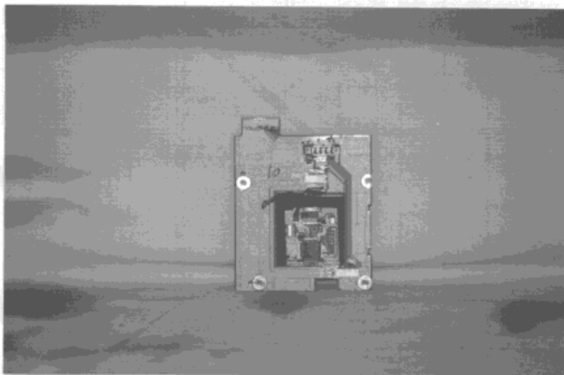
Mouse Main Board Solder Side View
