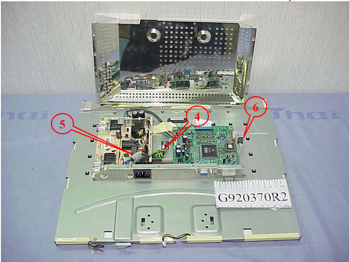
Figure 6 Internal View (Main Metal Cover)
