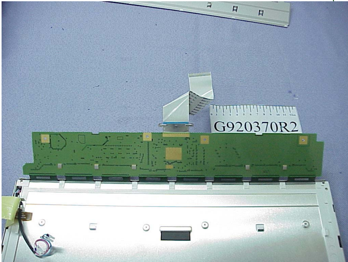
Figure 17 PCB of LCD Panel (Foil Side)
