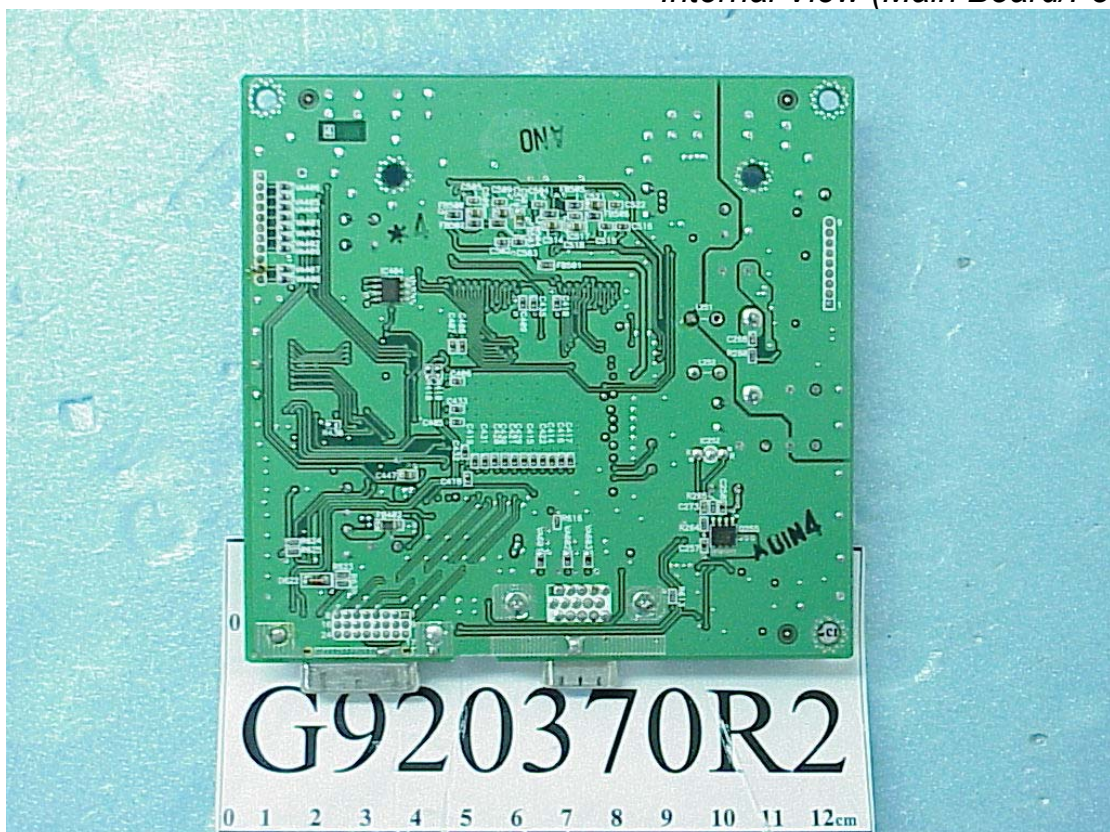
Figure 8 Internal View (Main Board/Foil Side)
