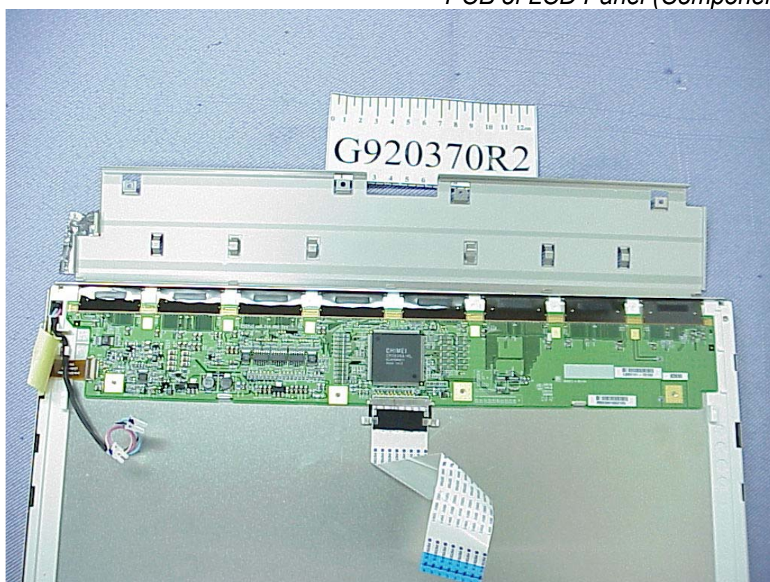
Figure 16 PCB of LCD Panel (Component Side)
