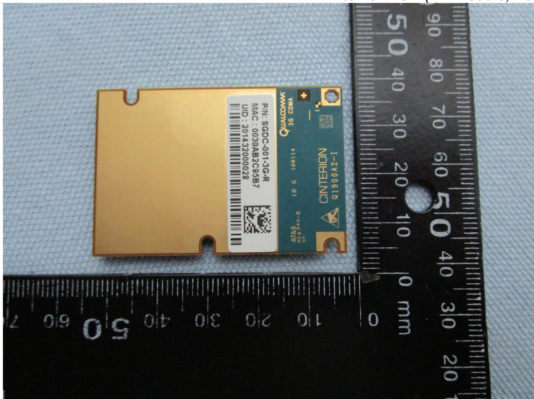
Figure 9 Internal View (RF Module, Back View)
