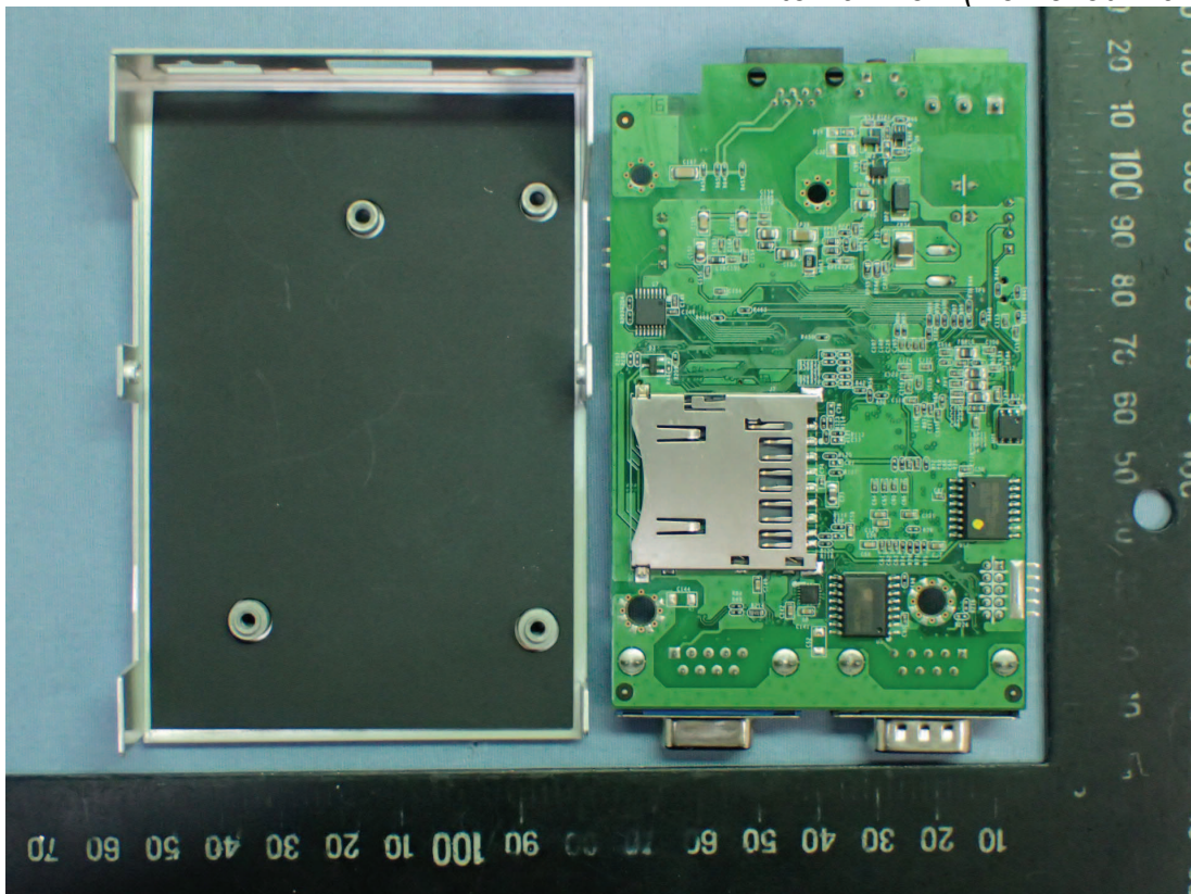
Figure 13 Internal View (Removed Main Board)
