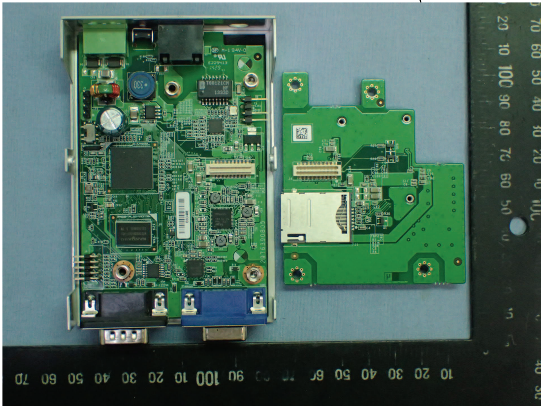
Figure 10 Internal View (Removed Internal Board)
