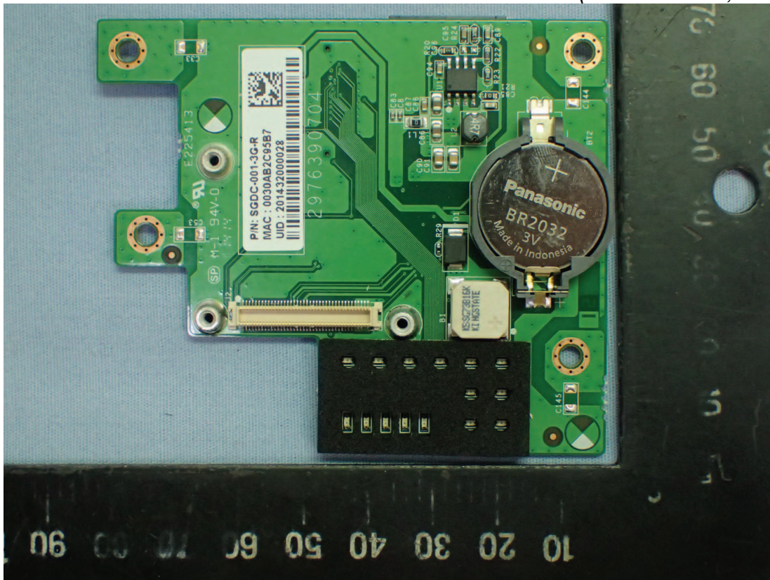
Figure 12 Internal View (Internal Board, Front View)
