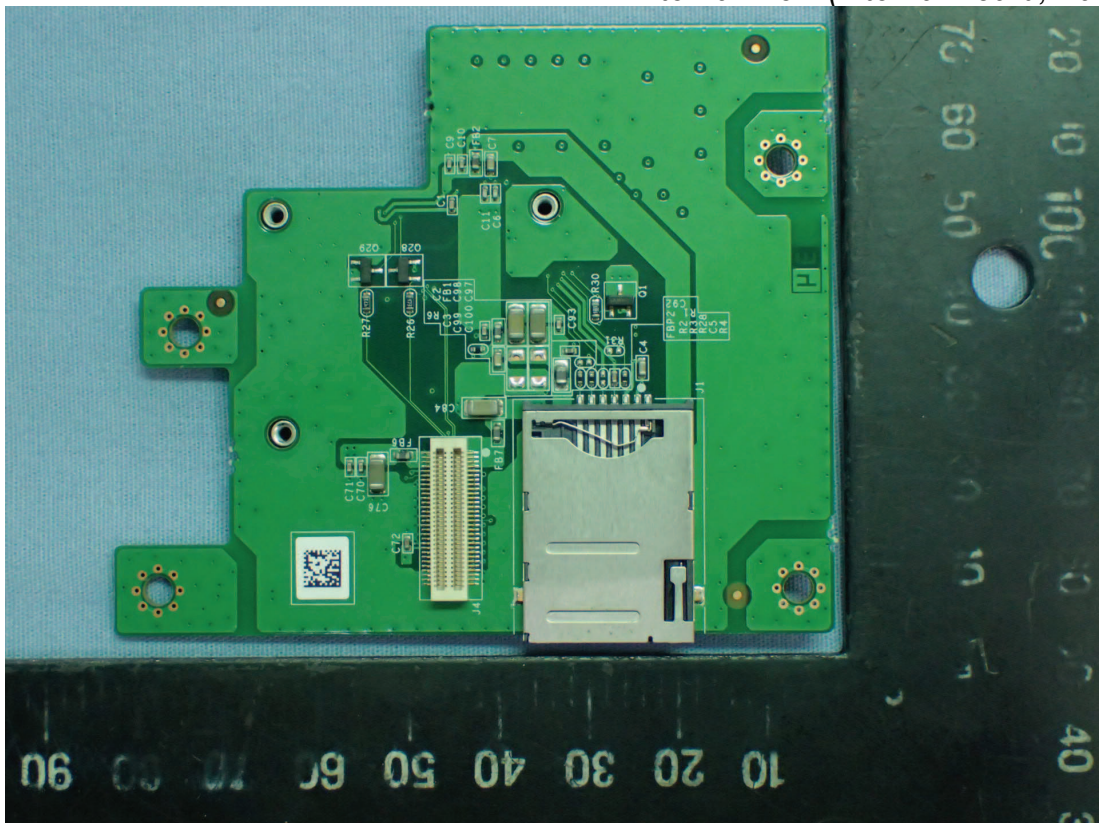
Figure 11 Internal View (Internal Board, Back View)
