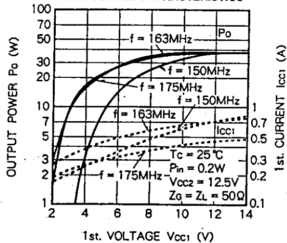
OUTPUT POWER, 1st. CURRENT VS. 1st. VOLTAGE CHARACTERISTICS
