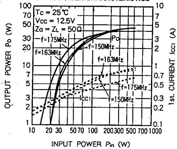
OUTPUT POWER, 1st. CURRENT VS. INPUT POWER CHARACTERISTICS
