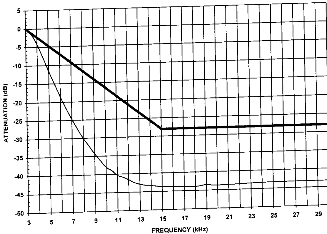
AUDIO FILTER RESPONSE FOR 6.25 kHz/12.5 kHz SPACED EQUIPMENT 27.41 - 174 MHz
