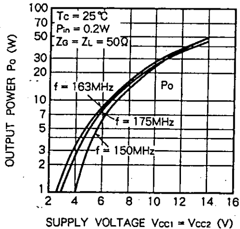
OUTPUT POWER VS. SUPPLY VOLTAGE CHARACTERISTICS
