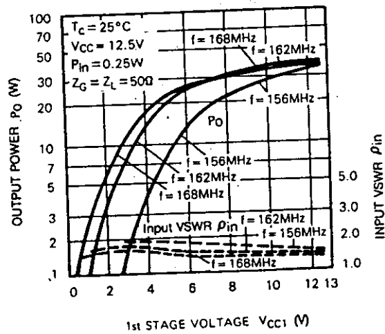
OUTPUT POWER, INPUT VSWR VS. FIRST STAGE VOLTAGE
