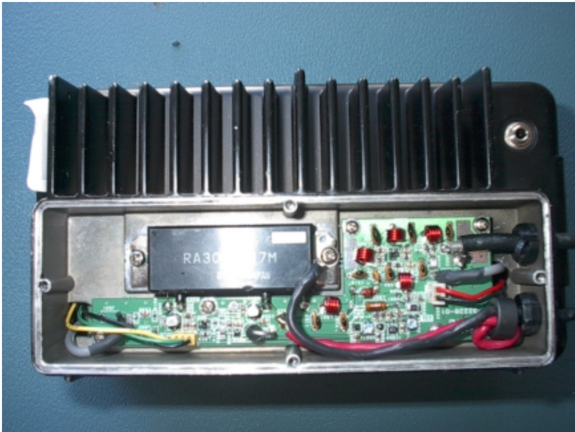
Fig. 11 – PA PCB Mounted
