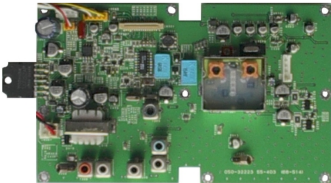
Fig 10 Main PCB front side without shield
