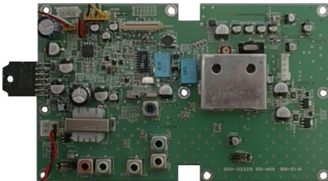
Fig. 9 Main PCB front side with Shield
