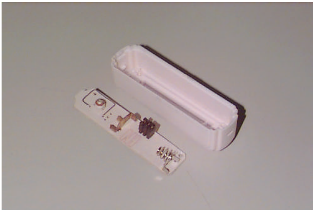
Transmitter SAMPLE PHOTOGRAPHS – INSIDE VIEW
