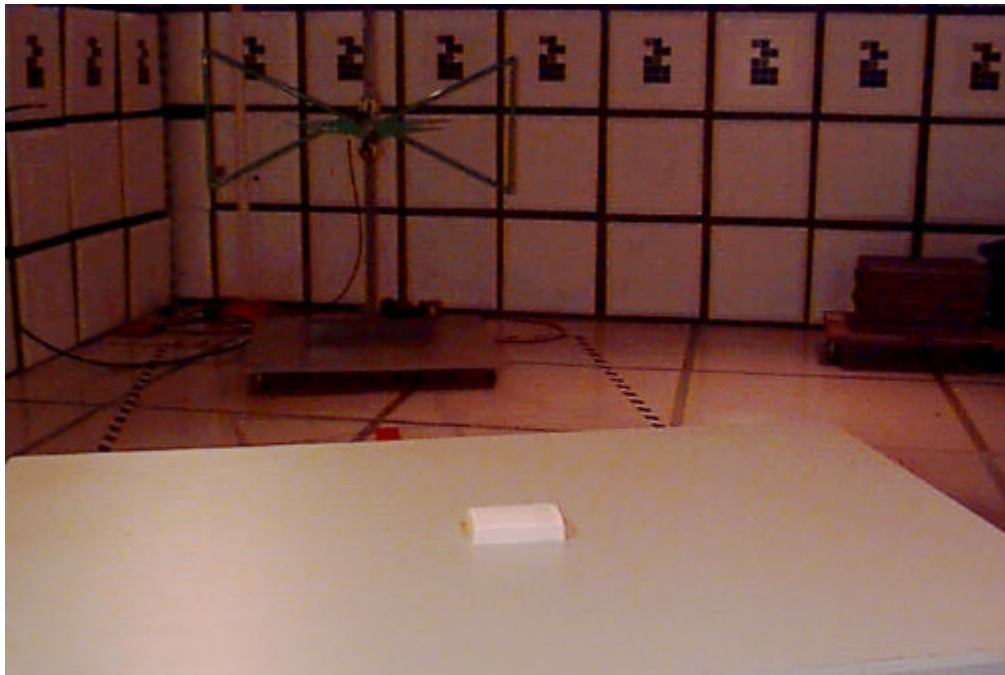
Radiated Emission Test Set-up – Receiver
