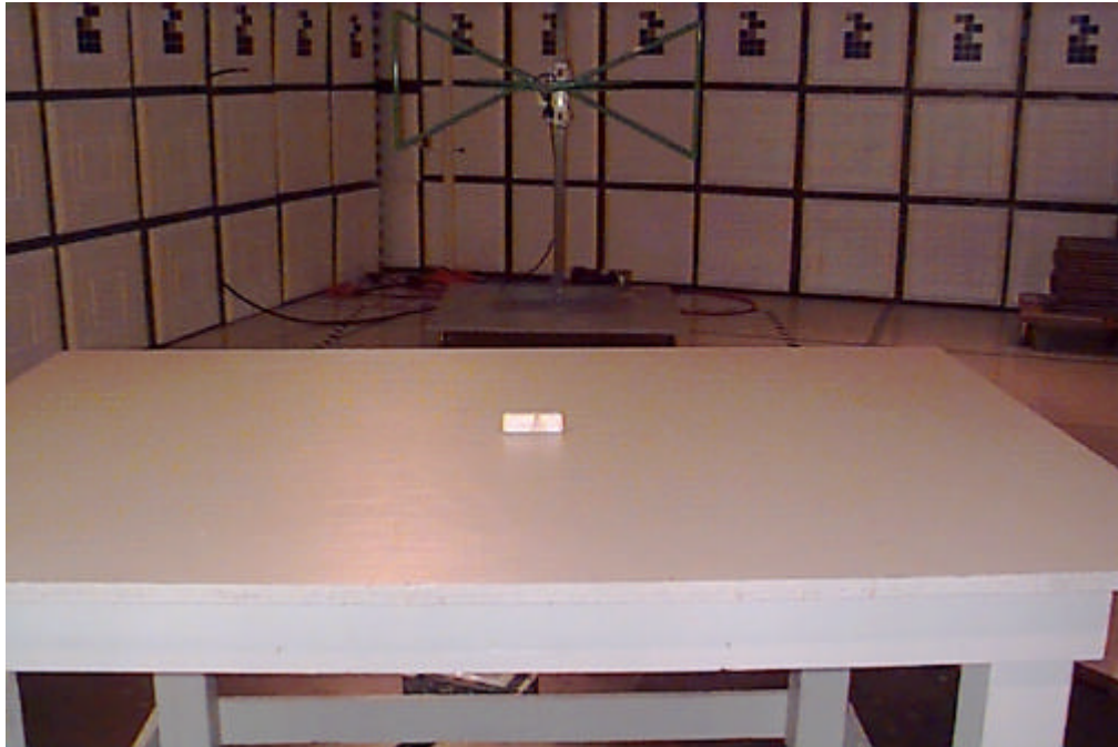
Radiated Emission Test Set-up – Transmitter
