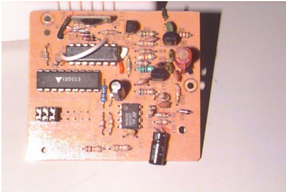
Receiver SAMPLE PHOTOGRAPHS – PCB COMPONENT SIDE VIEW
