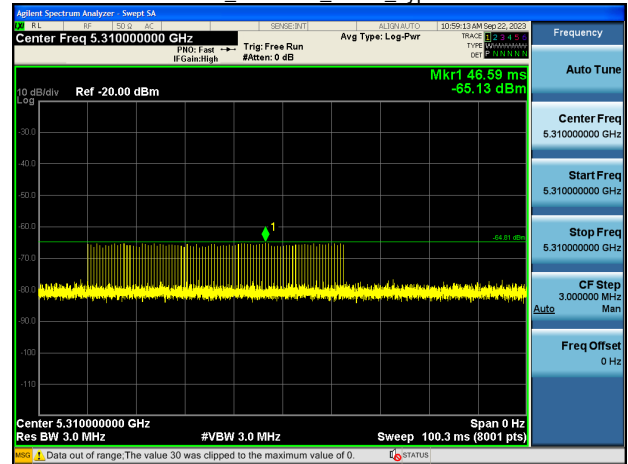
EHT40_5310MHz_Radar_Type 1-B
