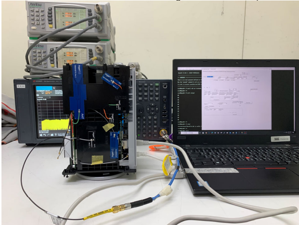
Part_15.247_2.4G_CDD_Conducted_setup
