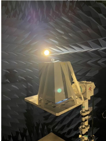
MLO_Setup
