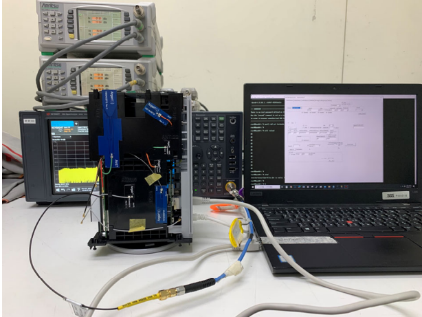
Part_15.247_BLE_Conducted_Setup
