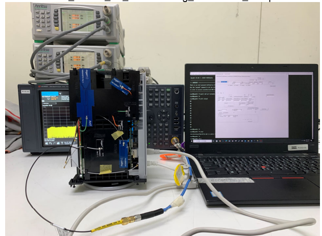
Part_15.407_6E_CDD_Conducted_Setup
