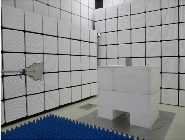
Part_15.247_2.4G_CDD_Radiated_Setup
