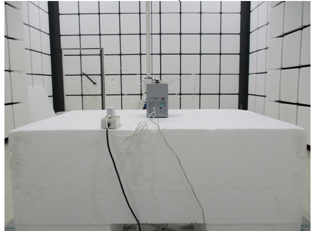
MLO_Setup
