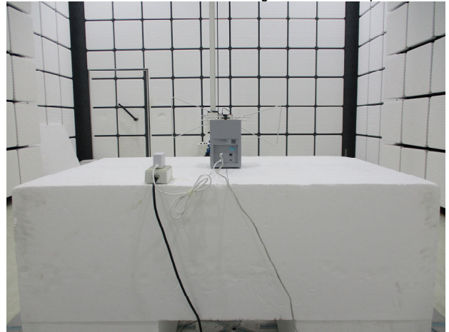
Part_15.407_5G_CDD_Radiated_Setup
