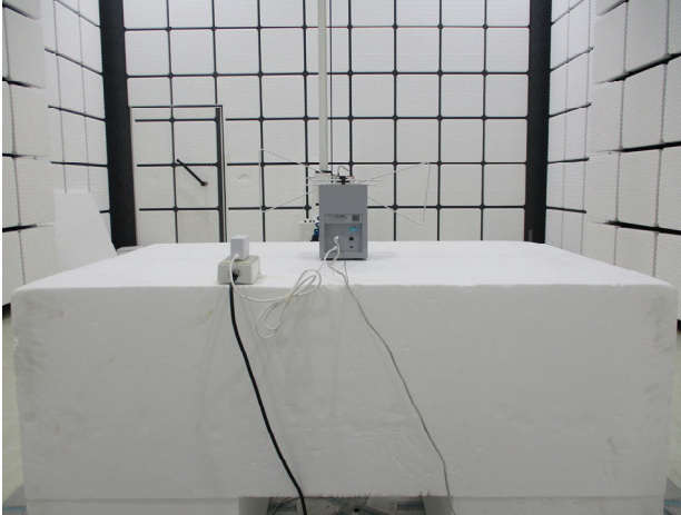
Part_15.407_6E_Beamforming_Radiated_Setup
