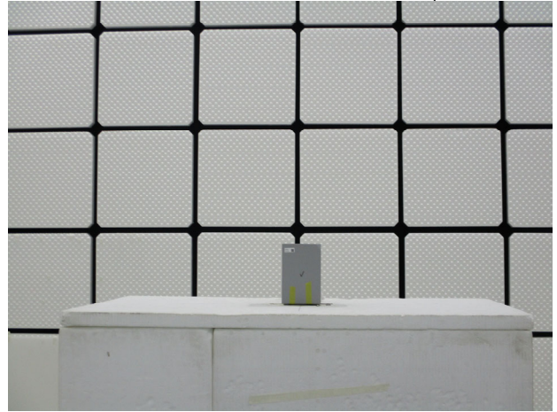
Part_15.247_2.4G_Beamforming_Radiated_Setup
