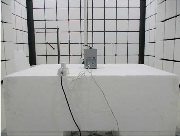
Part_15.407_6E_CDD_Radiated_Setup
