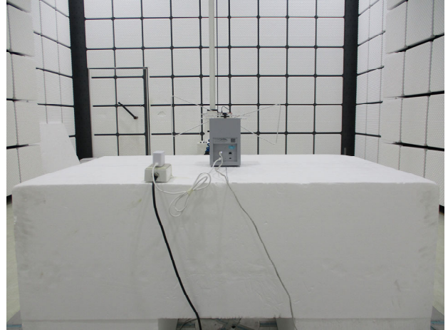
Part_15.247_2.4G_CDD_Radiated_Setup
