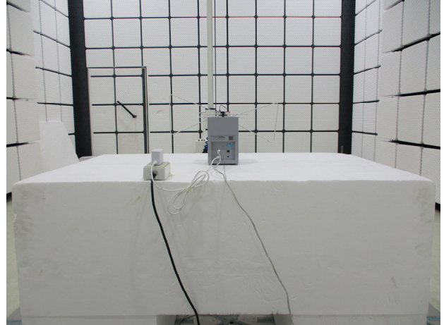
Part_15.247_2.4G_CDD_Radiated_Setup
