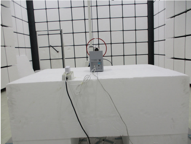
Part_15.407_6E_Beamforming_Radiated_Setup
