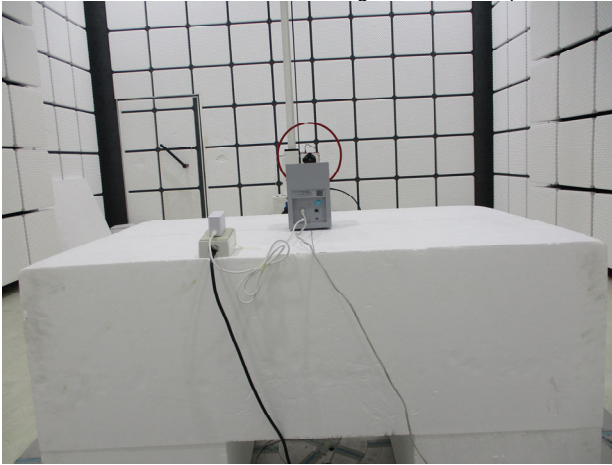
Part_15.407_5G_CDD_Radiated_Setup
