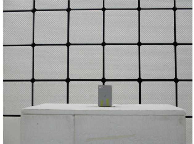
Part_15.407_5G_Beamforming_Radiated_Setup
