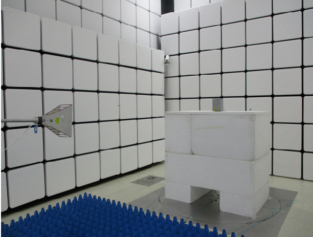
Part_15.247_2.4G_Beamforming_Radiated_Setup
