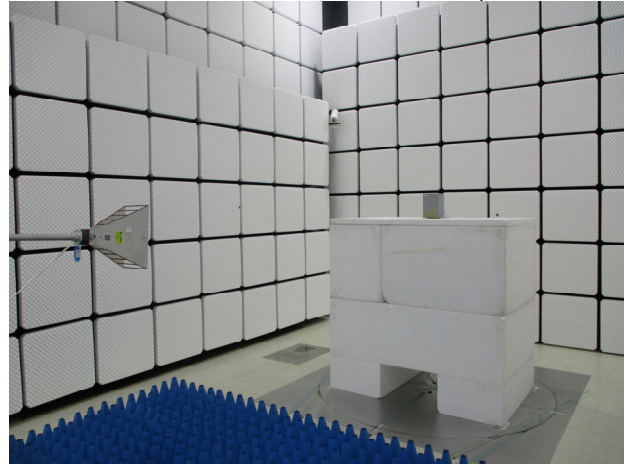
Part_15.407_6E_Beamforming_Radiated_Setup
