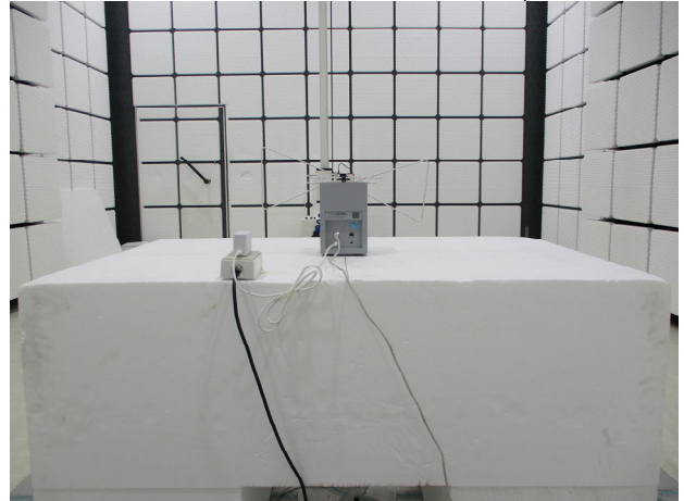
Part_15.407_5G_CDD_Radiated_Setup
