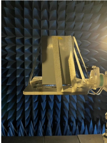
DG_EUT setup (2)
