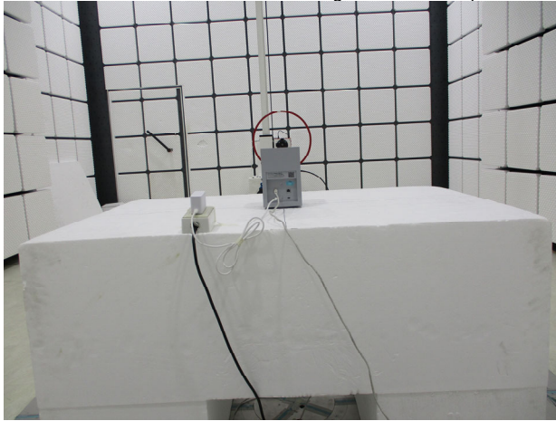
Part_15.247_2.4G_CDD_Radiated_Setup
