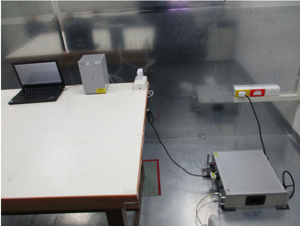
Part_15.407_5G_Conduction_Setup
