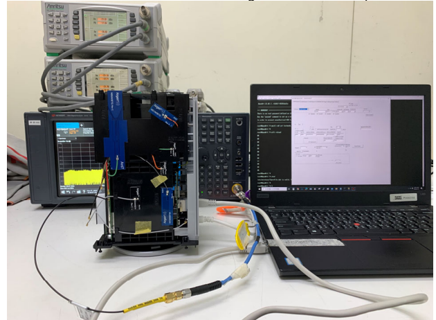
Part_15.407_5G_CDD_Conducted_Setup
