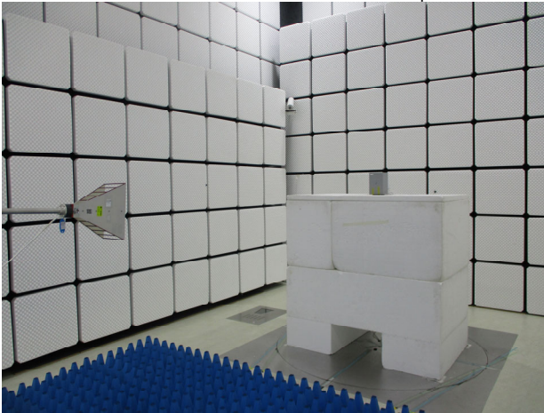
Part_15.407_5G_Beamforming_Radiated_Setup
