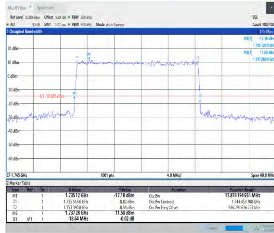
1-N66-PC3-15-20-M-3-DFT-16QAM-Outter_Full-100 @0-Ant3-17.874-18.640-≤20-PASS
