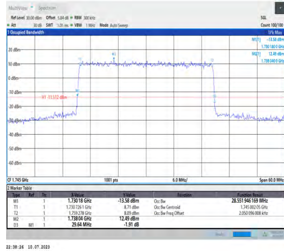
1-N66-PC3-15-30-M-1-DFT-QPSK-Outer_Full-160@ 0-Ant3-28.552-29.640-≤30-PASS
