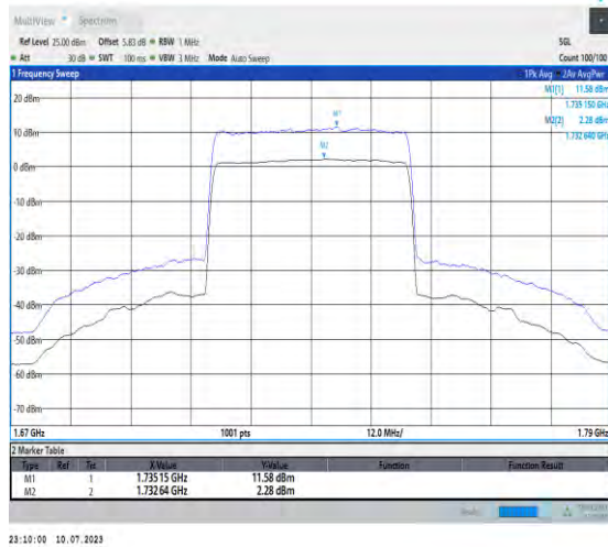
1-N66-PC3-15-40-L-1-DFT-256QAM-Outer_Full-216 @0-Ant3-9.30-100%-0.00-9.30-PASS-≤13
