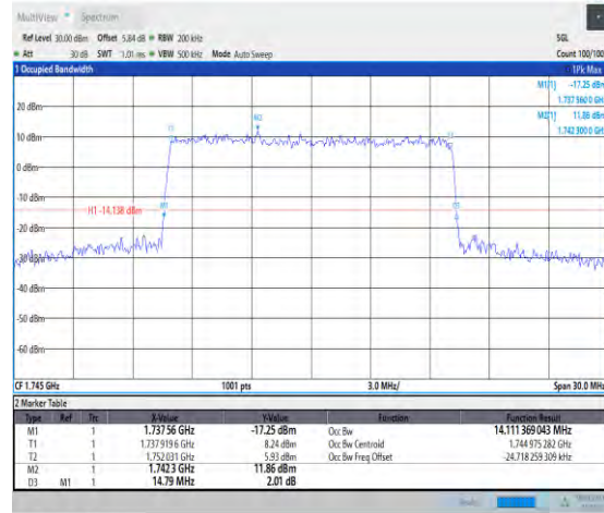
1-N66-PC3-15-15-M-8-CP-64QAM-Outer_Full-79@0 -Ant3-14.111-14.790-≤15-PASS
