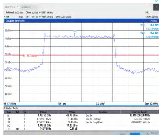
1-N66-PC3-15-15-M-2-DFT-PI2BPSK-Outer_Full-75@ 0-Ant3-13.411-14.070≤15-PASS
