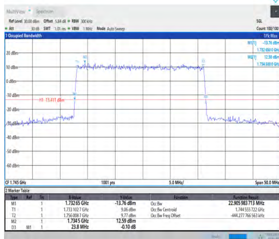
1-N66-PC3-15-25-M-3-DFT-16QAM-Outter_Full-128 @0-Ant3-22.906-23.800-≤25-PASS
