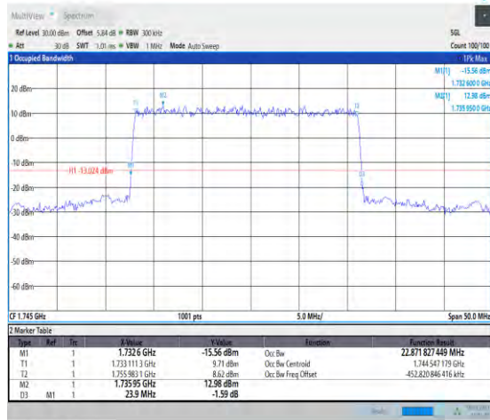
1-N66-PC3-15-25-M-1-DFT-QPSK-Outter_Full-128@ 0-Ant3-22.872-23.900-≤25-PASS
