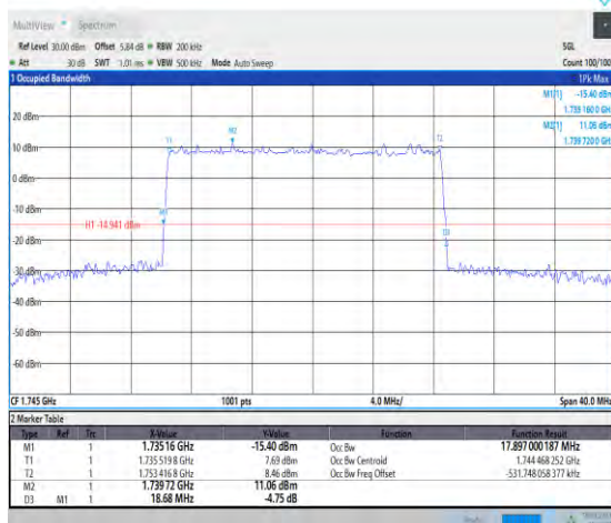
1-N66-PC3-15-20-M-4-DFT-64QAM-Outter_Full-100 @0-Ant3-17.897-18.680-≤20-PASS
