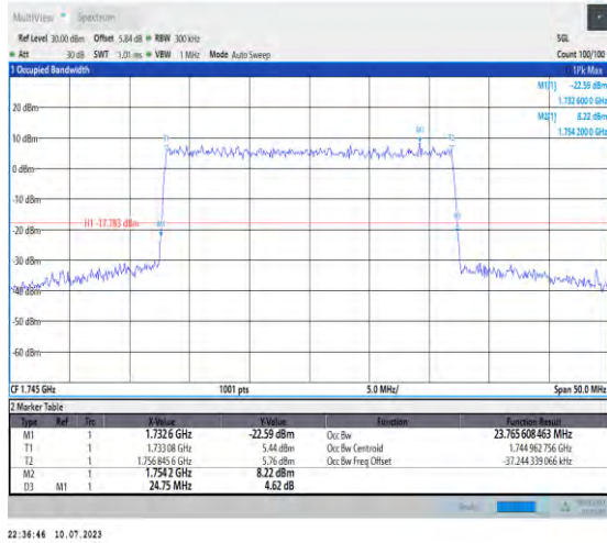
1-N66-PC3-15-25-M-9-CP-256QAM-Outer_Full-133 @0-Ant3-23.766-24.750-≤25-PASS
