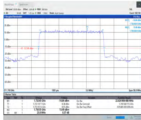
1-N66-PC3-15-25-M-2-DFT-PI2BPSK-Outter_Full-128 @0-Ant3-22.825-23.800-≤25-PASS
