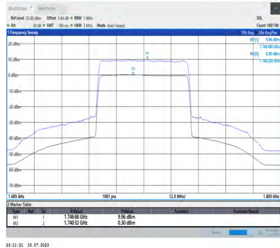
1-N66-PC3-15-40-M-2-CP-256QAM-Outer_Full-216 @0-Ant3-9.66-100%-0.00-9.66-PASS-≤13
