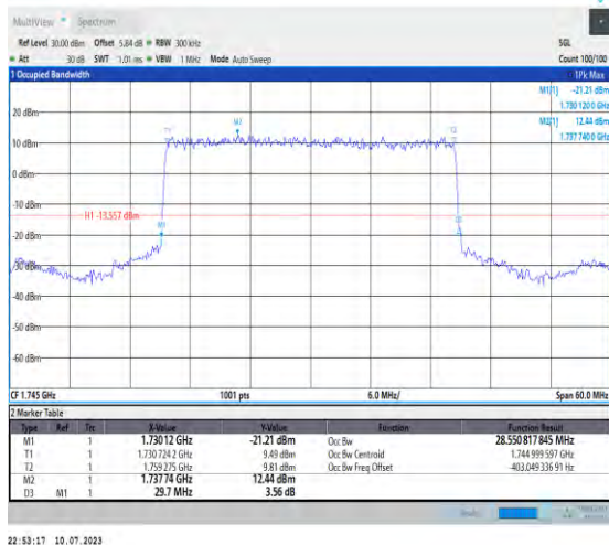
1-N66-PC3-15-30-M-2-DFT-PI2BPSK-Outer_Full-160 @0-Ant3-28.551-29.700-≤30-PASS
