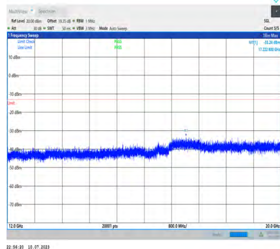
1-N66-PC3-15-40-M-1-DFT-PI2BPSK-Inner_1RB_L t-1@1-12000-20000-Ant3-17222.80--33.24--13-PASS
