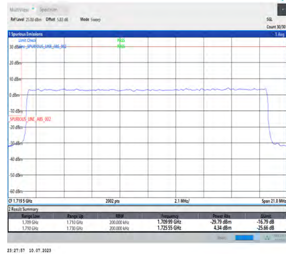
1-N66-PC3-15-20-L-3-DFT-PI2BPSK-Outer_Full-100@0-Ant3-1-seegraph-PASS-see graph
