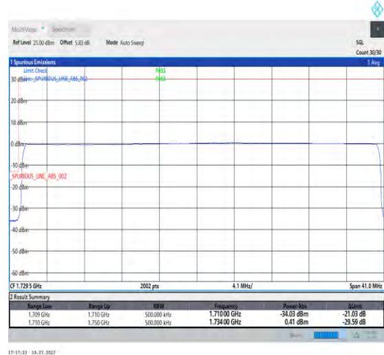
1-N66-PC3-15-40-L-6-CP-QPSK-Outer_Full-216@0-Ant3-1-seegraph-PASS-see graph
