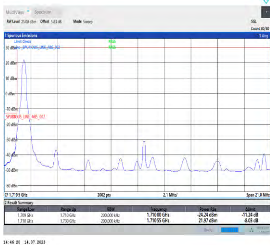
1-N66-PC3-15-20-L-4-CP-QPSK-Edge_1RB_Left-1@0-Ant3-1-seegraph-PASS-see graph
