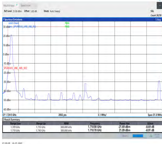
1-N66-PC3-15-30-L-1-DFT-PI2BPSK-Edge_1RB_Left-1@0-Ant3-1-seegraph-PASS-see graph
