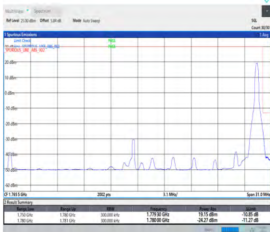
1-N66-PC3-15-30-H-5-CP-QPSK-Edge_1RB_Right-1@159-Ant3-1-seegraph-PASS-see graph
