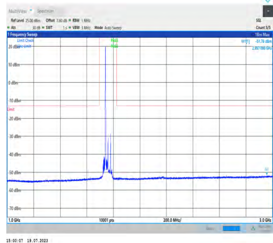
1-N66-PC3-15-40-H-1-DFT-PI2BPSK-Inner_1RB_Lef t-1@1-1000-3000-Ant3-2597.00--51.78--13-PASS
