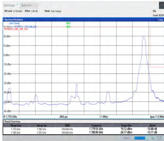
1-N66-PC3-15-10-H-2-DFT-PI2BPSK-Edge_1RB_Right-t-1@51-Ant3-1-seegraph-PASS-see graph
