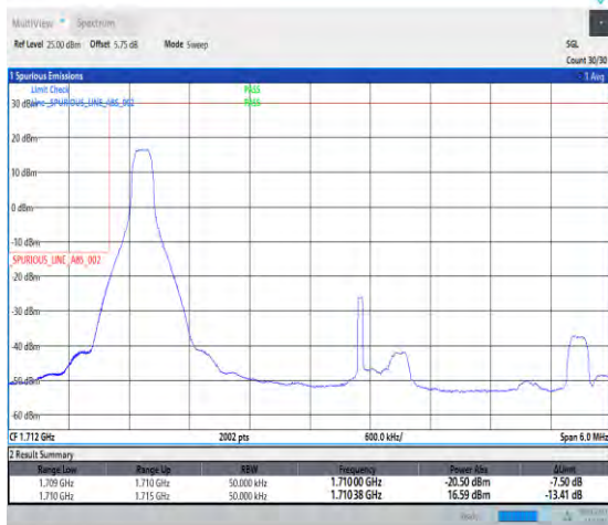
1-N66-PC3-15-5-L-4-CP-QPSK-Edge_1RB_Left-1@0-Ant3-1-seegraph-PASS-see graph
