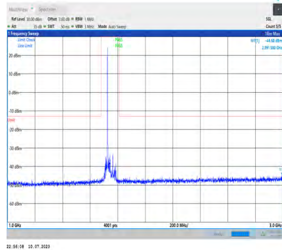
1-N66-PC3-15-40-M-1-DFT-PI2BPSK-Inner_1RB_L t-1@1-1000-3000-Ant3-2991.50--44.68--13-PASS
