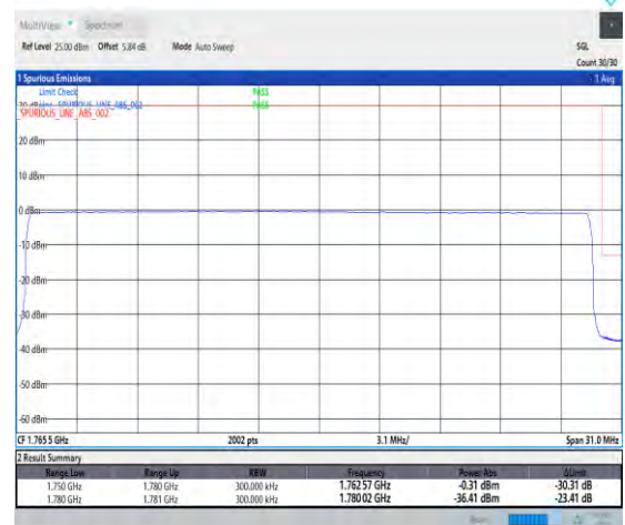
1-N66-PC3-15-30-H-6-CP-QPSK-Outer_Full-160@0-Ant3-1-seegraph-PASS-see graph
