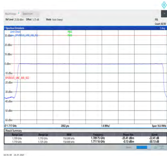
1-N66-PC3-15-15-L-6-CP-QPSK-Outer_Full-79@0-Ant3-1-seegraph-PASS-see graph
