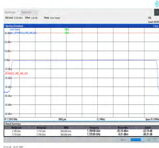
1-N66-PC3-15-30-L-6-CP-QPSK-Outer_Full-160@0-Ant3-1-seegraph-PASS-see graph
