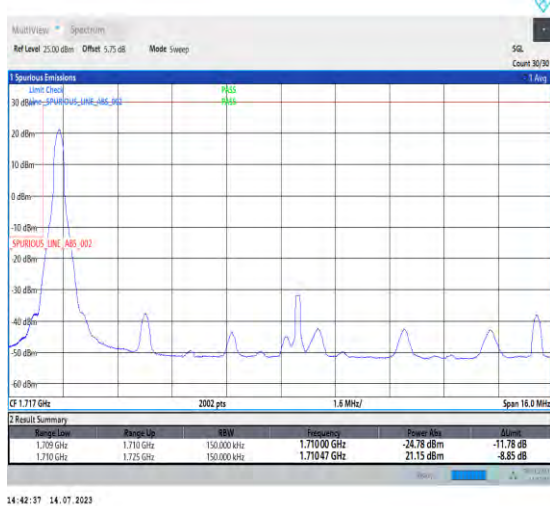
1-N66-PC3-15-15-L-4-CP-QPSK-Edge_1RB_Left-1@0-Ant3-1-seegraph-PASS-see graph
