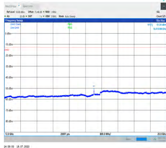
1-N66-PC3-15-40-M-1-DFT-PI2BPSK-Inner_1RB_L t-1@1-12000-20000-Ant3-16416.00--51.54--13-PASS
