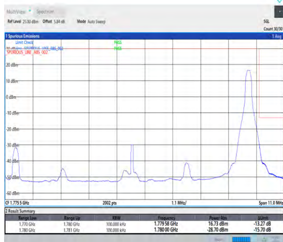
1-N66-PC3-15-10-H-5-CP-QPSK-Edge_1RB_Right-1@51-Ant3-1-seegraph-PASS-see graph
