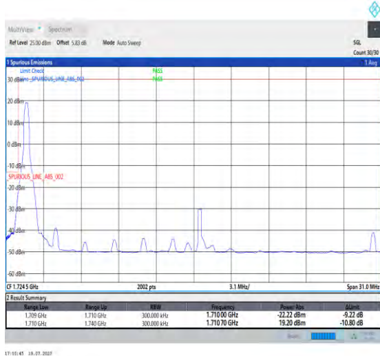
1-N66-PC3-15-30-L-4-CP-QPSK-Edge_1RB_Left-1@0-Ant3-1-seegraph-PASS-see graph
