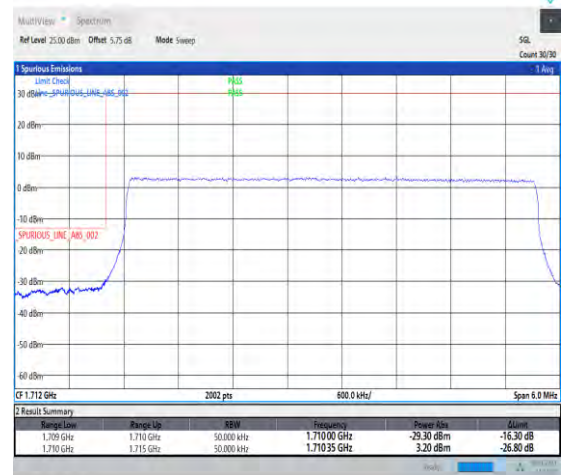
1-N66-PC3-15-5-L-6-CP-QPSK-Outer_Full-25@0-Ant3-1-seegraph-PASS-see graph
