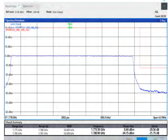
1-N66-PC3-15-5-H-6-CP-QPSK-Outer_Full-25@0-Ant3-1-seegraph-PASS-see graph
