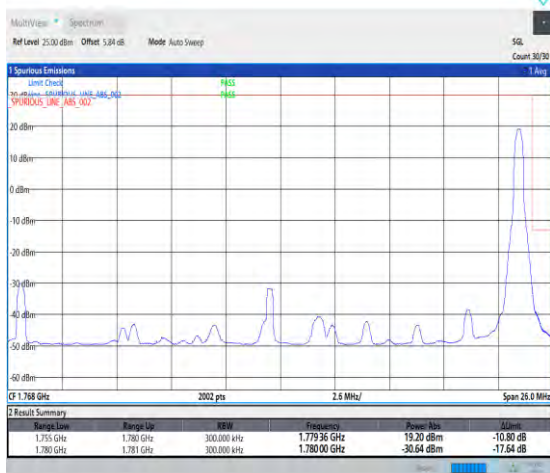
1-N66-PC3-15-25-H-5-CP-QPSK-Edge_1RB_Right-1@132-Ant3-1-seegraph-PASS-see graph
