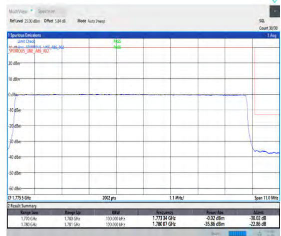
1-N66-PC3-15-10-H-6-CP-QPSK-Outer_Full-52@0-Ant3-1-seegraph-PASS-see graph
