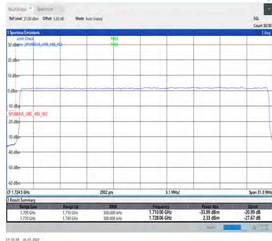
1-N66-PC3-15-30-L-3-DFT-PI2BPSK-Outer_Full-160@0-Ant3-1-seegraph-PASS-see graph
