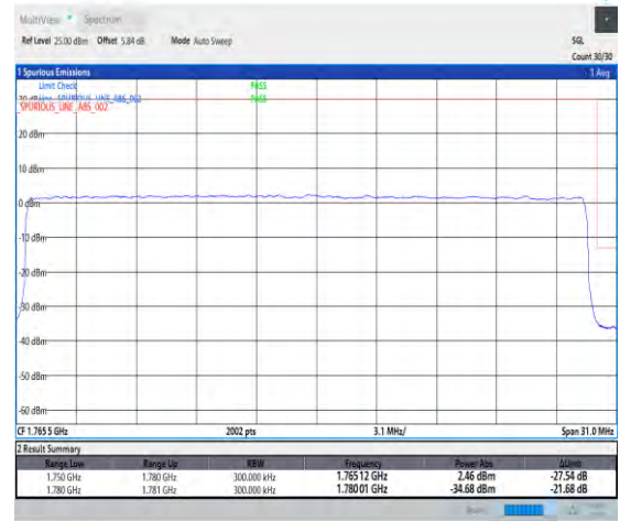
1-N66-PC3-15-30-H-3-DFT-PI2BPSK-Outer_Full-160@0-Ant3-1-seegraph-PASS-see graph
