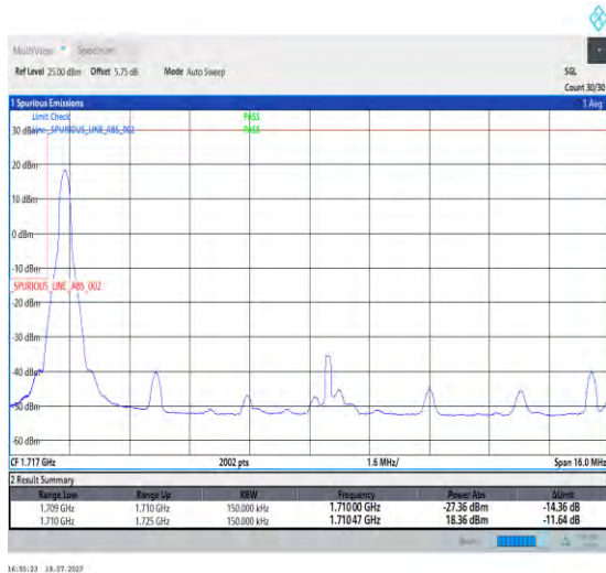
1-N66-PC3-15-15-L-4-CP-QPSK-Edge_1RB_Left-1@0-Ant3-1-seegraph-PASS-see graph
