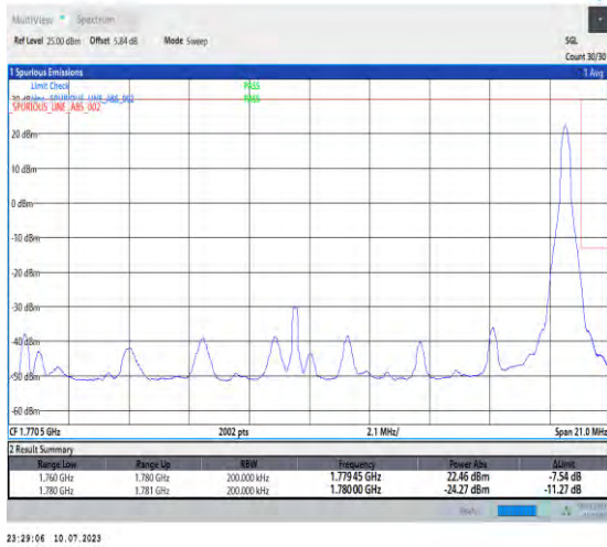
1-N66-PC3-15-20-H-2-DFT-PI2BPSK-Edge_1RB_Right-t-1@105-Ant3-1-seegraph-PASS-see graph
