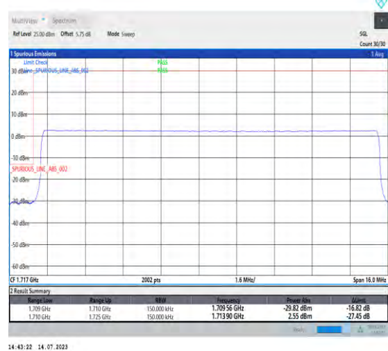
1-N66-PC3-15-15-L-6-CP-QPSK-Outer_Full-79@0-Ant3-1-seegraph-PASS-see graph
