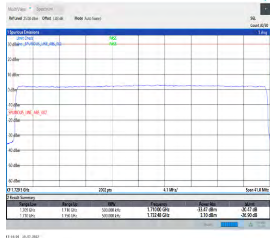
1-N66-PC3-15-40-L-3-DFT-PI2BPSK-Outer_Full-216@0-Ant3-1-seegraph-PASS-see graph
