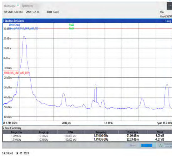
1-N66-PC3-15-10-L-1-DFT-PI2BPSK-Edge_1RB_Left-1@0-Ant3-1-seegraph-PASS-see graph
