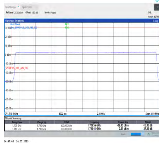
1-N66-PC3-15-20-L-6-CP-QPSK-Outer_Full-106@0-Ant3-1-seegraph-PASS-see graph
