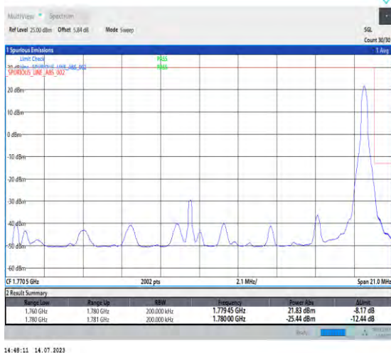
1-N66-PC3-15-20-H-5-CP-QPSK-Edge_1RB_Right-1@105-Ant3-1-seegraph-PASS-see graph
