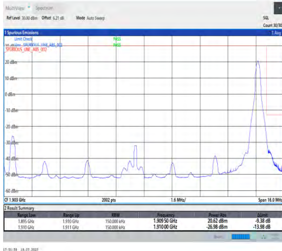
1-N2-PC3-15-15-H-2-DFT-PI2BPSK-Edge_1RB_Right-1@78-Ant3-1-seegraph-PASS-see graph
