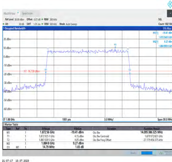
1-N2-PC3-15-15-M-9-CP-256QAM-Outer_Full-79@0- Ant3-14.095-14.790-≤15-PASS
