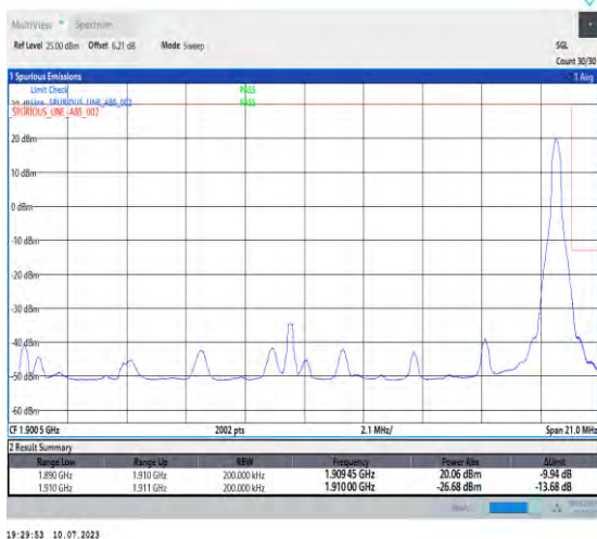
1-N2-PC3-15-20-H-5-CP-QPSK-Edge_1RB_Right-1@105-Ant3-1-seegraph-PASS-see graph
