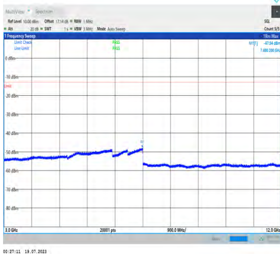
1-N2-PC3-15-20-M-1-DFT-PI2BPSK-Inner_1RB_Lef t-1@1-3000-12000-Ant3-7480.2--47.94--13-PASS
