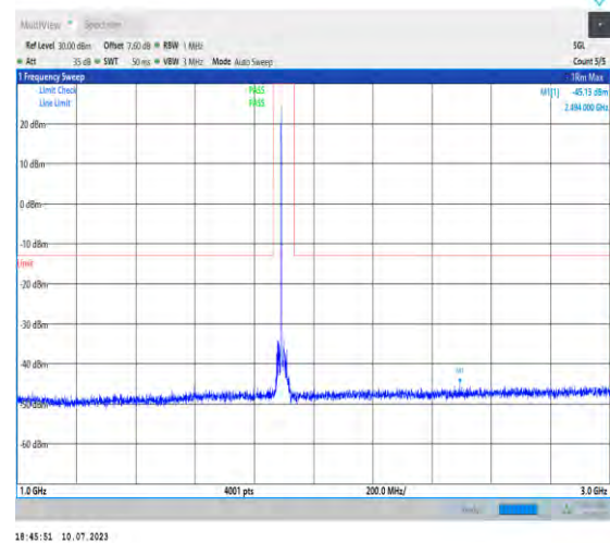
1-N2-PC3-15-20-H-1-DFT-PI2BPSK-Inner_1RB_Left- 1@1-1000-3000-Ant3-2494.00--45.13--13-PASS
