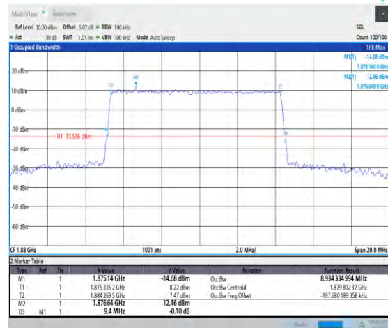
1-N2-PC3-15-10-M-3-DFT-16QAM-Outer_Full-50@0-Ant3-8.934-9.400-≤10-PASS
