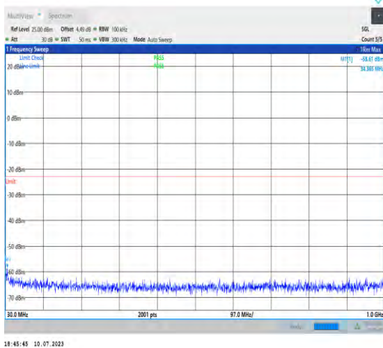
1-N2-PC3-15-20-H-1-DFT-PI2BPSK-Inner_1RB_Lef t-1@1-30-1000-Ant3-34.37--58.61--23-PASS
