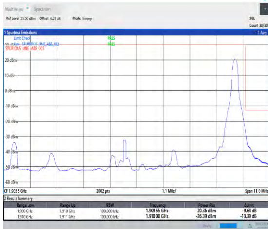
1-N2-PC3-15-10-H-2-DFT-PI2BPSK-Edge_1RB_Right-1@51-Ant3-1-seegraph-PASS-see graph
