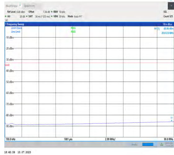
1-N2-PC3-15-20-H-1-DFT-PI2BPSK-Inner_1RB_Left- 1@1-0.15-30-Ant3-29.61--85.94--33-PASS
