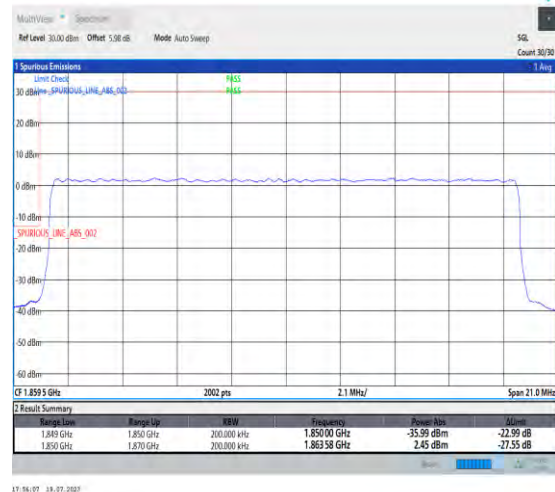
1-N2-PC3-15-20-L-3-DFT-PI2BPSK-Outer_Full-100@0-Ant3-1-seegraph-PASS-see graph
