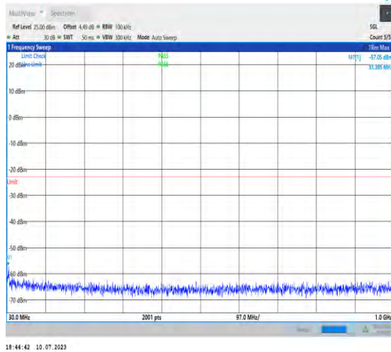
1-N2-PC3-15-20-M-1-DFT-PI2BPSK-Inner_1RB_Left- t-1@1-30-1000-Ant3-33.40--57.05--23-PASS
