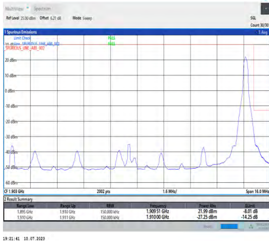
1-N2-PC3-15-15-H-2-DFT-PI2BPSK-Edge_1RB_Right-1@78-Ant3-1-seegraph-PASS-see graph
