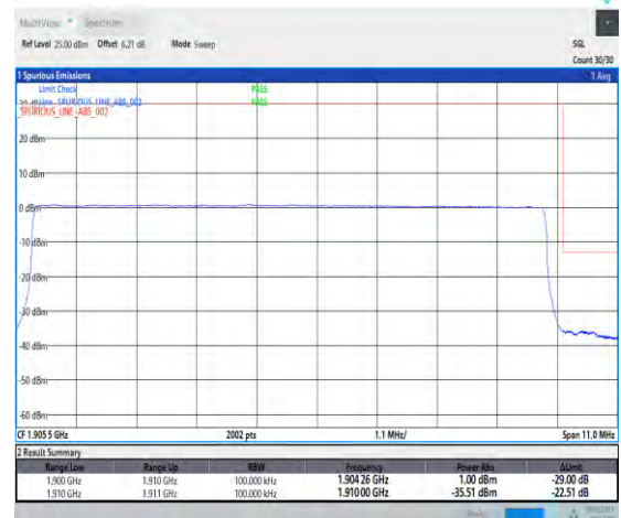
1-N2-PC3-15-10-H-6-CP-QPSK-Outer_Full-52@0-Ant3-1-seegraph-PASS-see graph
