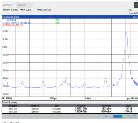
1-N2-PC3-15-15-H-5-CP-QPSK-Edge_1RB_Right-1@78-Ant3-1-seegraph-PASS-see graph
