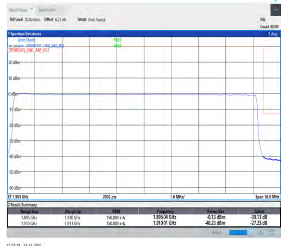
1-N2-PC3-15-15-H-6-CP-QPSK-Outer_Full-79@0-Ant3-1-seegraph-PASS-see graph
