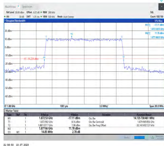
1-N2-PC3-15-15-M-6-CP-QPSK-Outer_Full-79@0-Ant3-14.136-14.850-≤15-PASS
