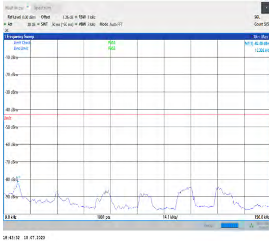
1-N2-PC3-15-20-L-1-DFT-PI2BPSK-Inner_1RB_Left -1@1-0.009-0.15-Ant3-0.02--82.48--43-PASS
