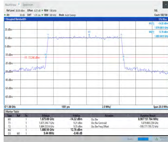
1-N2-PC3-15-10-M-1-DFT-QPSK-Outer_Full-50@0- Ant3-8.907-9.440-≤10-PASS
