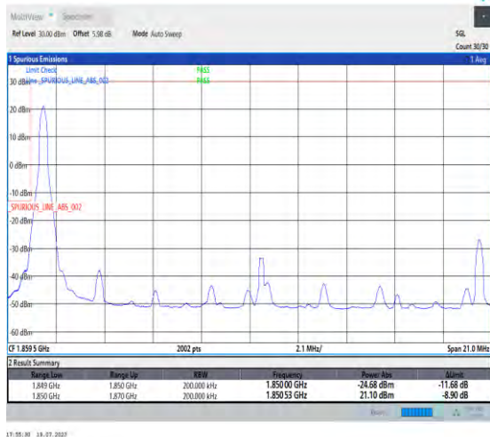
1-N2-PC3-15-20-L-1-DFT-PI2BPSK-Edge_1RB_Left-1@0-Ant3-1-seegraph-PASS-see graph
