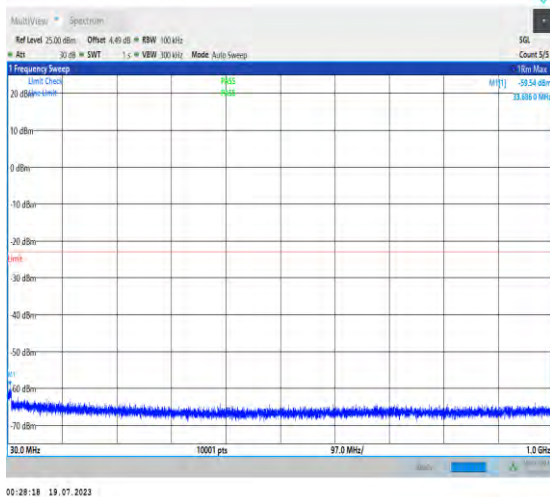
1-N2-PC3-15-20-H-1-DFT-PI2BPSK-Inner_1RB_Left -1@1-30-1000-Ant3-33.686--59.54--23-PASS
