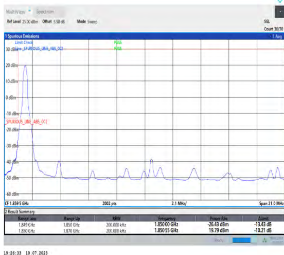
1-N2-PC3-15-20-L-4-CP-QPSK-Edge_1RB_Left-1@0-Ant3-1-seegraph-PASS-see graph
