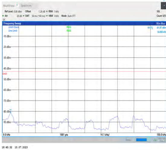
1-N2-PC3-15-20-H-1-DFT-PI2BPSK-Inner_1RB_Lef t-1@1-0.009-0.15-Ant3-0.02--81.97--43-PASS
