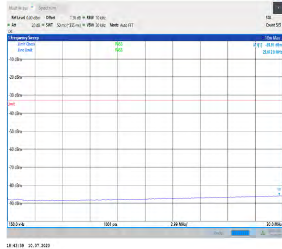
1-N2-PC3-15-20-L-1-DFT-PI2BPSK-Inner_1RB_Left- 1@1-0.15-30-Ant3-29.61--85.91--33-PASS
