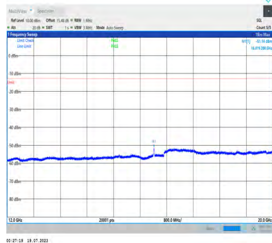
1-N2-PC3-15-20-M-1-DFT-PI2BPSK-Inner_1RB_Left- 1@1-12000-20000-Ant3-16419.2--51.14--13-PASS
