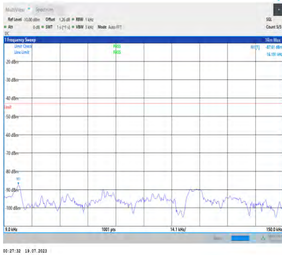
1-N2-PC3-15-20-H-1-DFT-PI2BPSK-Inner_1RB_Left -1@1-0.009-0.15-Ant3-16.191--87.61--43-PASS
