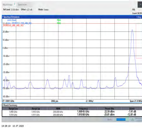
1-N2-PC3-15-20-H-2-DFT-PI2BPSK-Edge_1RB_Right-1@105-Ant3-1-seegraph-PASS-see graph
