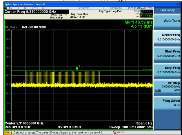
EHT40_5310MHz_Radar_Type 1-B
