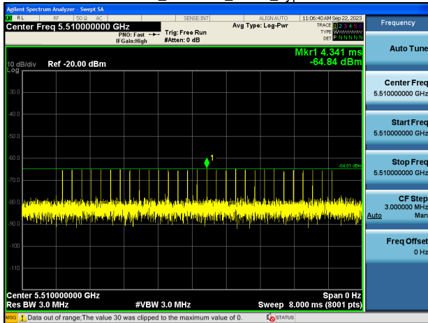
EHT40_5510MHz_Radar_Type 3
