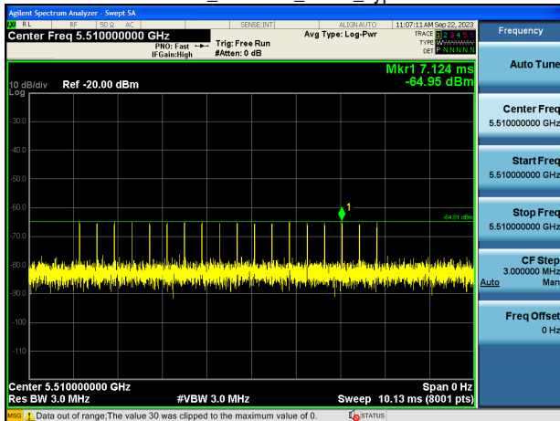
EHT40_5510MHz_Radar_Type 3
