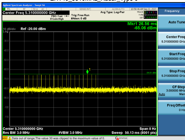
EHT40_5310MHz_Radar_Type 0
