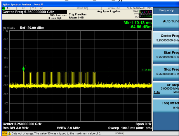
EHT160_5250MHz_Radar_Type 1-B
