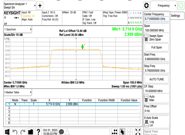
802.11n_40MHz_Chain0_5710MHz_UNII 2C
