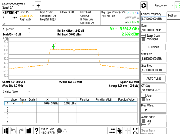
802.11n_40MHz_Chain3_5710MHz_UNII 2C
