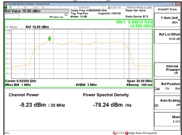
Channel Power+PSD_802.11be20_802.11be20 6855MHz
