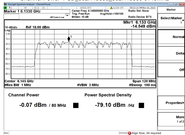
Channel Power+PSD_802.11be80_802.11be80 6145MHz
