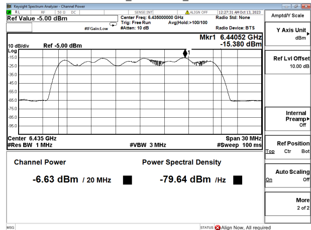
Channel Power+PSD_802.11be20_802.11be20 6435MHz
