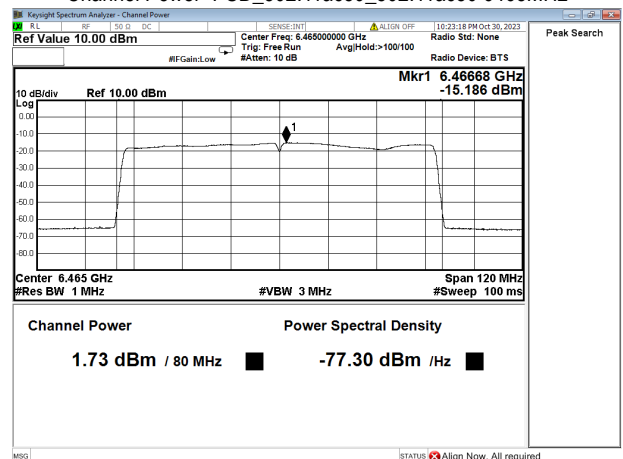
Channel Power+PSD_802.11ac80_802.11ac80 6465MHz
