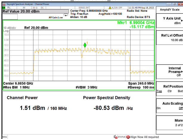
Channel Power+PSD_802.11ac160_802.11ac160 6985MHz
