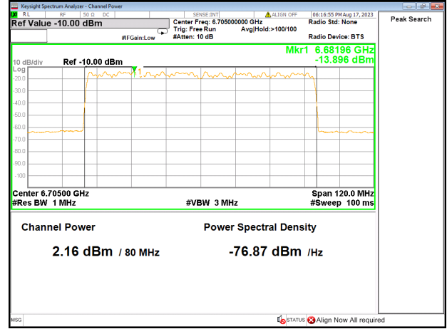
Channel Power+PSD_802.11be80_802.11be80 6705MHz
