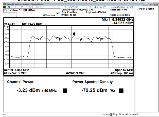
Channel Power+PSD_802.11be40_802.11be40 6845MHz
