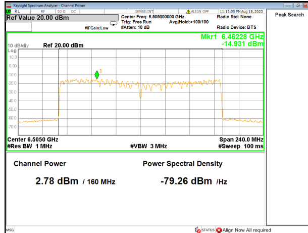
Channel Power+PSD_802.11ac160_802.11ac160 6505MHz
