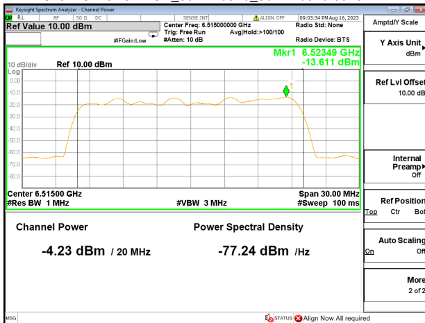
Channel Power+PSD_802.11be20_802.11be20 6515MHz
