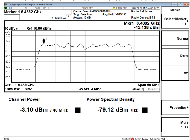
Channel Power+PSD_802.11n40_802.11n40 6485MHz
