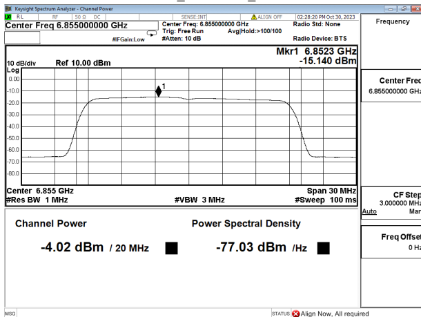
Channel Power+PSD_802.11n20_802.11n20 6855MHz
