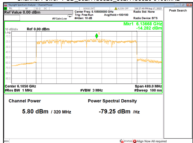
Channel Power+PSD_802.11be320_802.11be320 6105MHz
