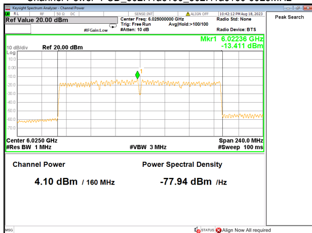
Channel Power+PSD_802.11ac160_802.11ac160 6025MHz
