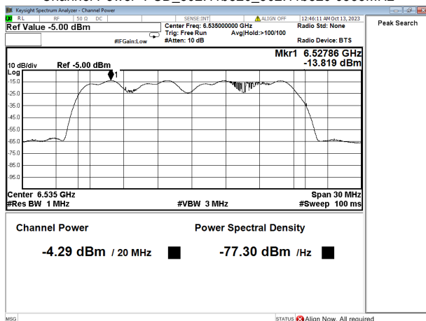
Channel Power+PSD_802.11be20_802.11be20 6535MHz
