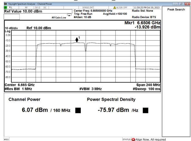
Channel Power+PSD_802.11ac160_802.11ac160 6665MHz
