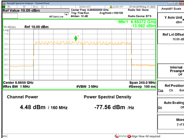
Channel Power+PSD_802.11be160_802.11be160 6665MHz
