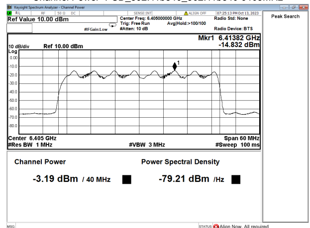
Channel Power+PSD_802.11be40_802.11be40 6405MHz
