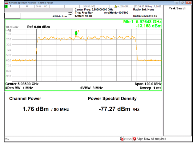
Channel Power+PSD_802.11be80_802.11be80 5985MHz
