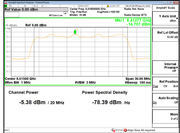
Channel Power+PSD_802.11be20_802.11be20 6415MHz
