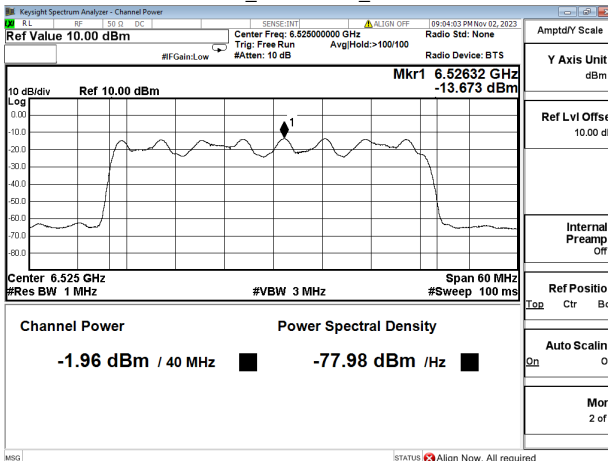
Channel Power+PSD_802.11be40_802.11be40 6525MHz
