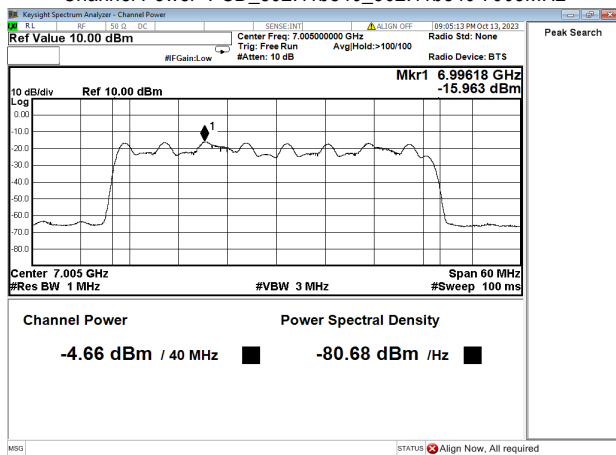
Channel Power+PSD_802.11be40_802.11be40 7005MHz
