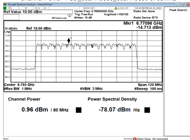
Channel Power+PSD_802.11be80_802.11be80 6785MHz
