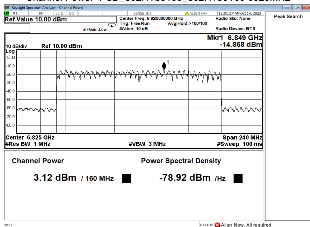
Channel Power+PSD_802.11be160_802.11be160 6825MHz
