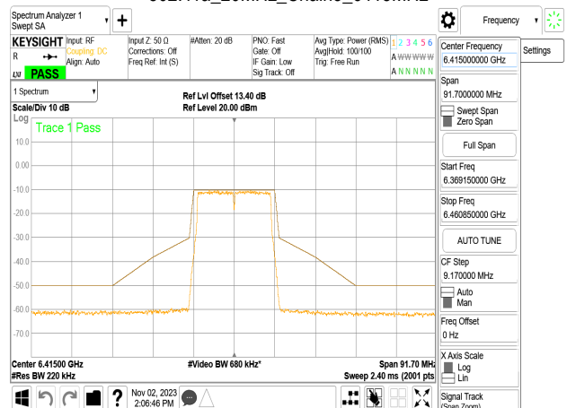
802.11a_20MHz_Chain3_6415MHz
