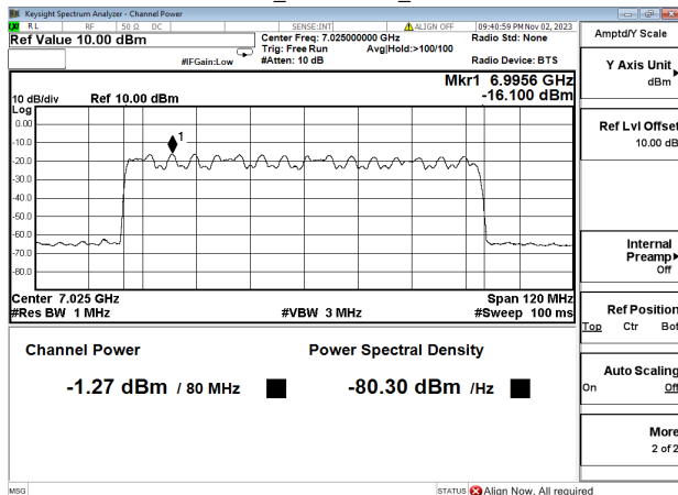
Channel Power+PSD_802.11be80_802.11be80 7025MHz
