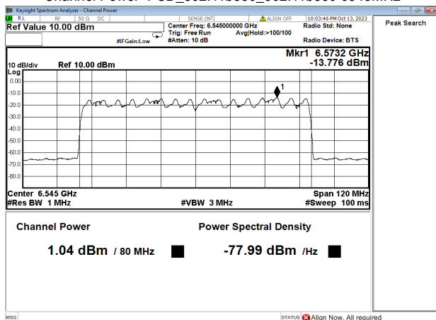
Channel Power+PSD_802.11be80_802.11be80 6545MHz
