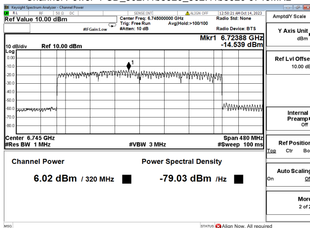
Channel Power+PSD_802.11be320_802.11be320 6745MHz
