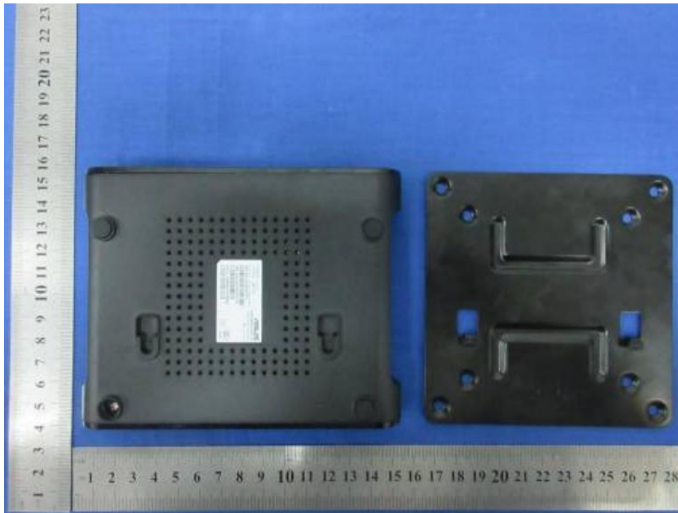
(7) EUT Photo
