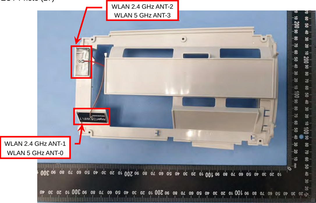
EUT Photo (28)
