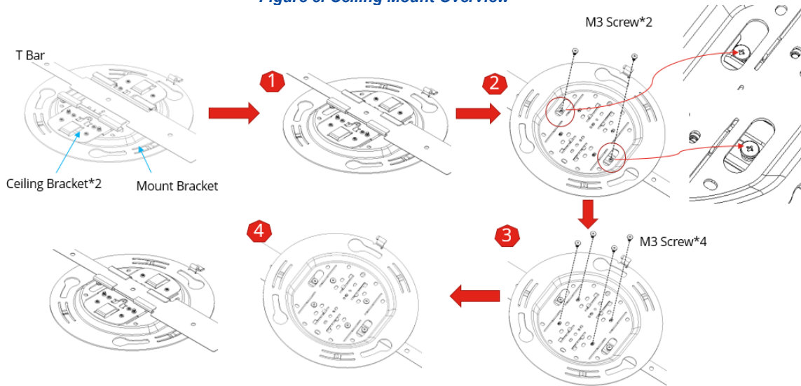
Figure 8. Ceiling Mount Overview
