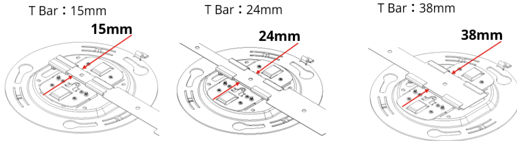
Figure 7. T Bar Width
