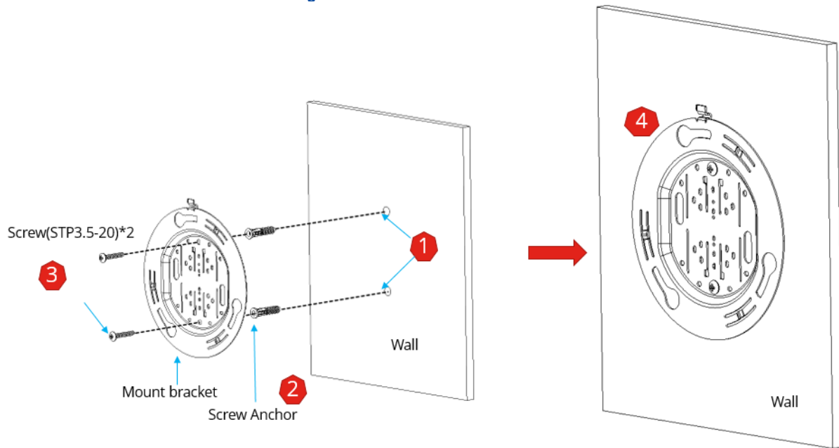
Figure 6. Wall Mount Overview
