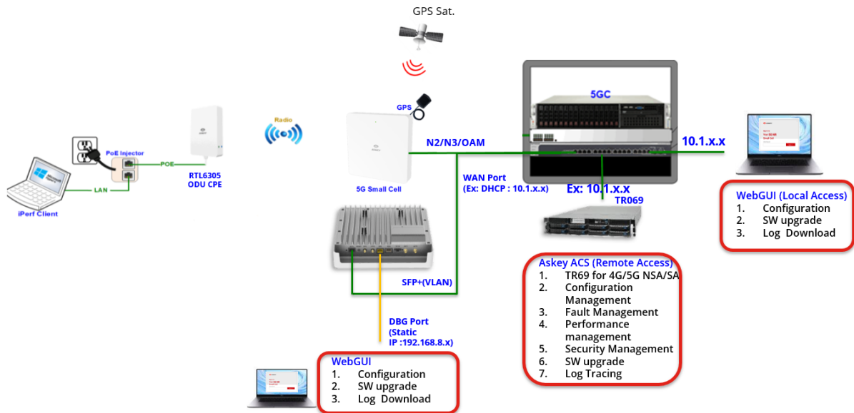
Figure 34. The Askey OAM Architecture
