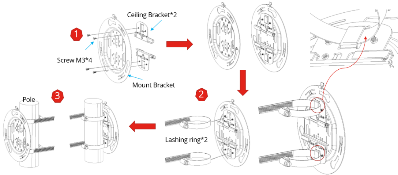
Figure 9. Pole Mount Overview
