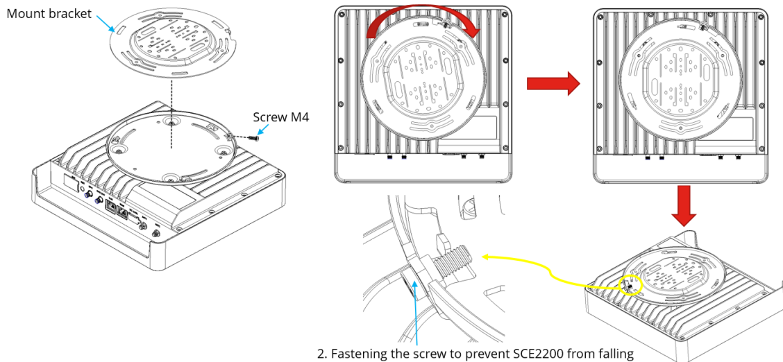
Figure 10. Align the Mount Base and the Mount Bracket
