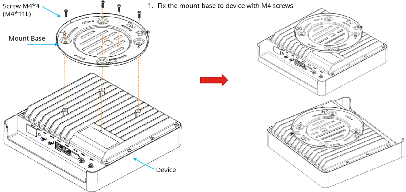
Figure 5. Fix the Mount Base to NR xCell 46116A
