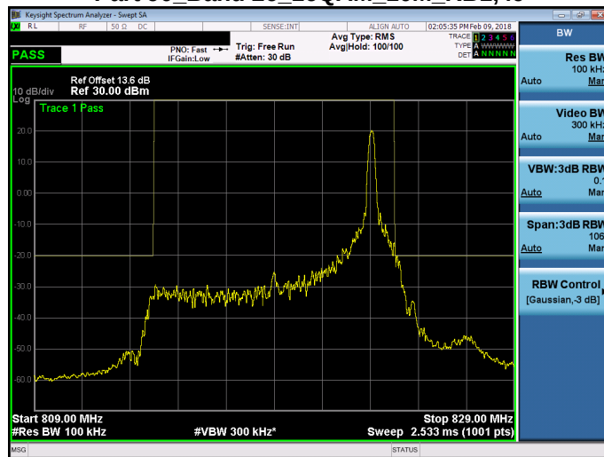
Part 90 Band 26_16QAM_10M_RB50,0
