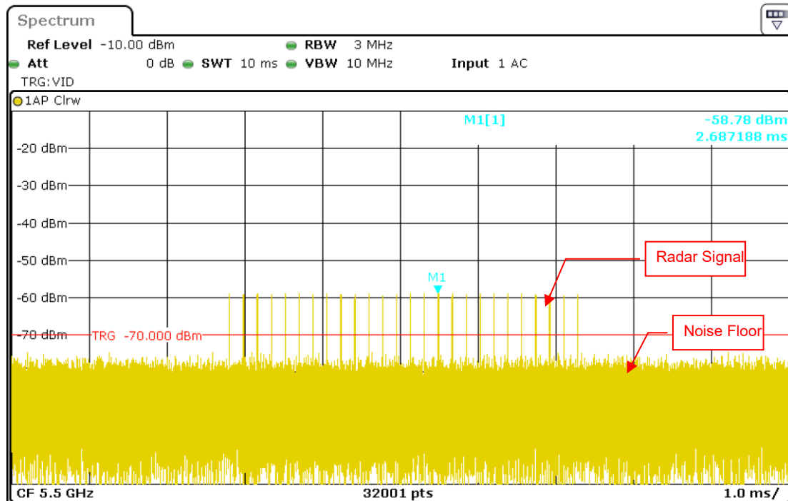
Radar Signal 2
