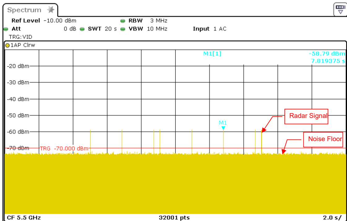
Radar Signal 5
