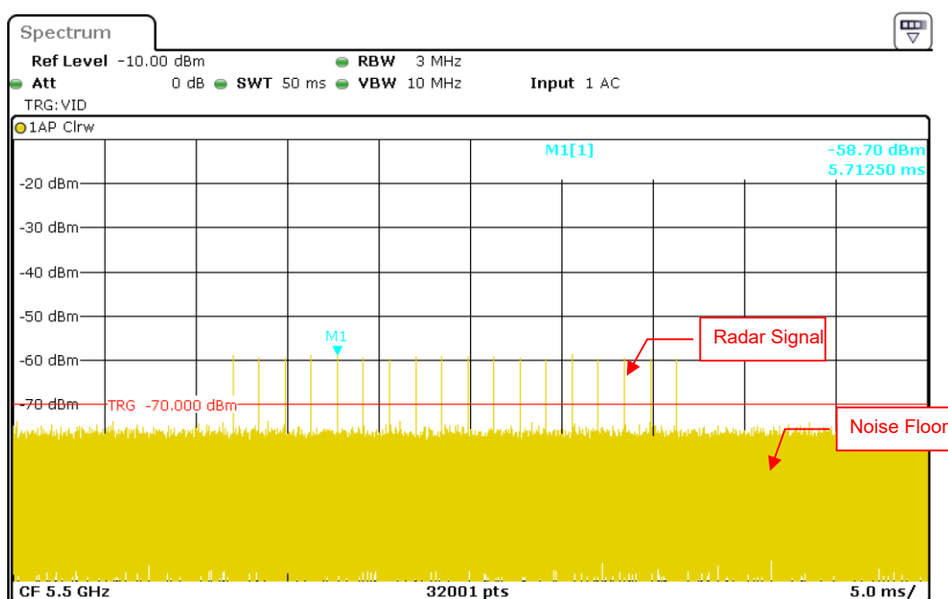
Radar Signal 0
