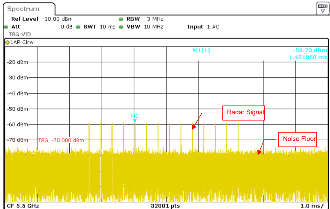
Radar Signal 4
