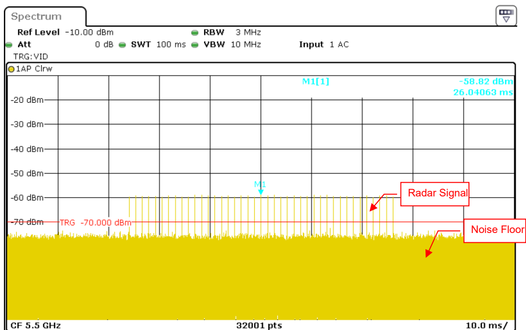
Radar Signal 1 (Test B)
