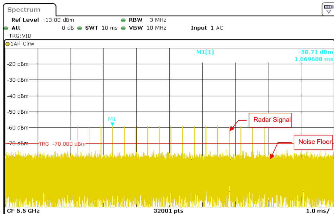
Radar Signal 3
