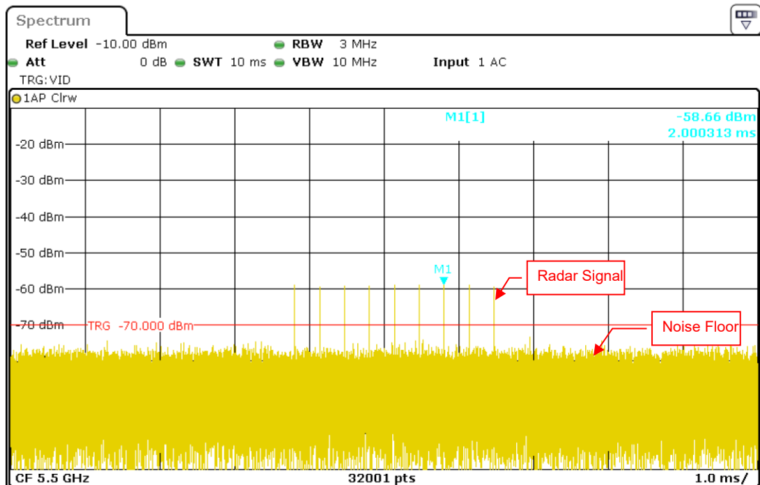
Radar Signal 6
