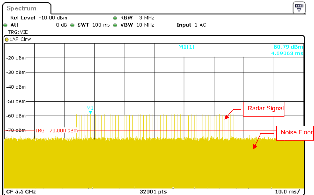
Radar Signal 1 (Test A)
