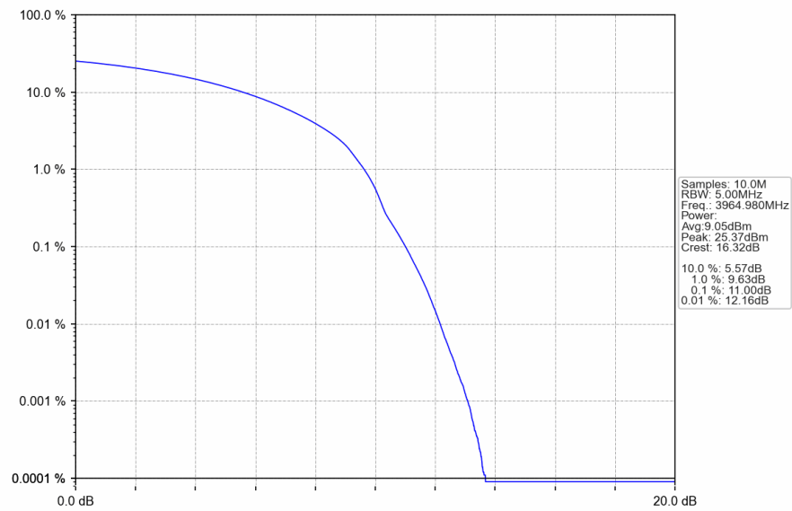
n77a_30kHz_SISO_NTNV_30MHz_DFT-s-OFDM_64_QAM_3964.98MHz_Outer_Full
