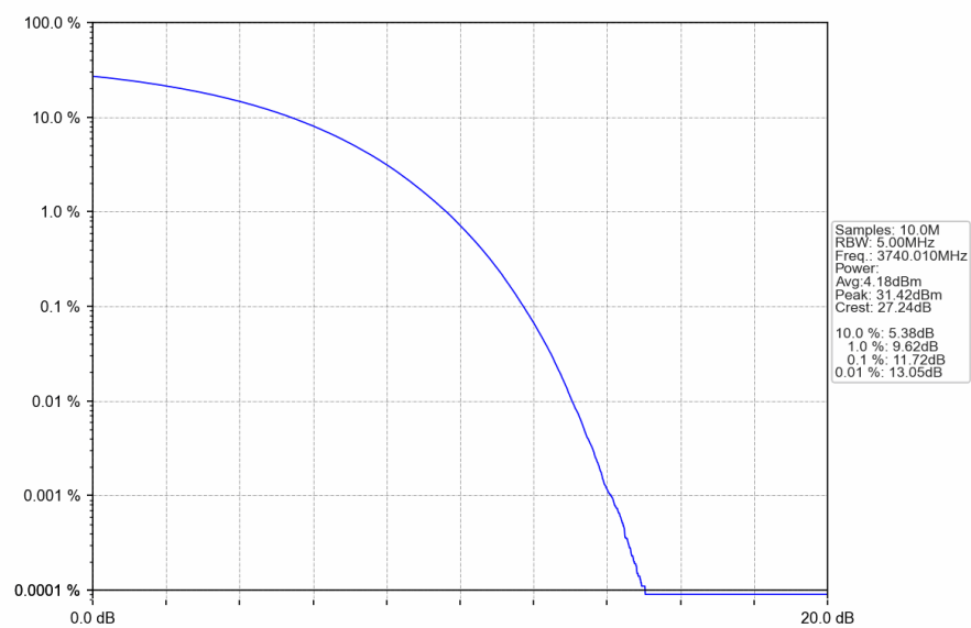
n77a_30kHz_SISO_NTNV_80MHz_CP-OFDM_QPSK_3740.01MHz_Outer_Full
