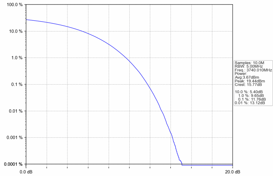
n77a_30kHz_SISO_NTNV_80MHz_CP-OFDM_64_QAM_3740.01MHz_Outer_Full
