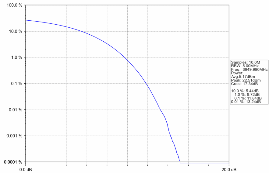
n77a_30kHz_SISO_NTNV_60MHz_CP-OFDM_QPSK_3949.98MHz_Outer_Full
