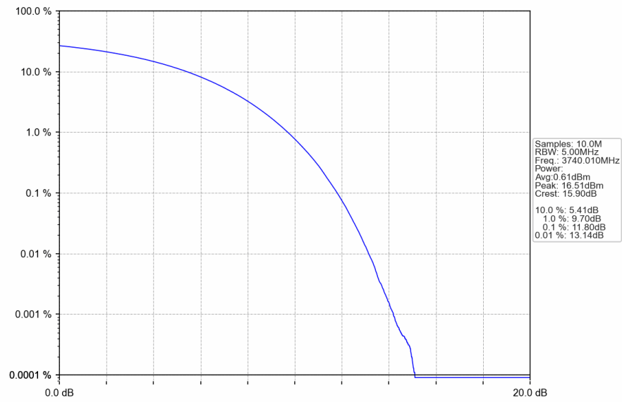
n77a_30kHz_SISO_NTNV_80MHz_CP-OFDM 256 QAM_3740.01MHz_Outer_Full
