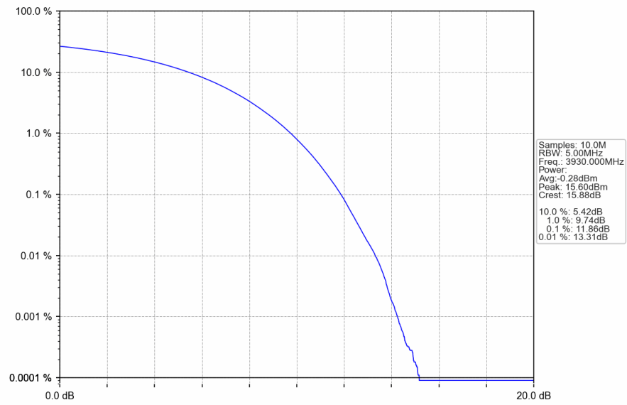
n77a_30kHz_SISO_NTNV_100MHz_CP-OFDM_256_QAM_3930MHz_Outer_Full
