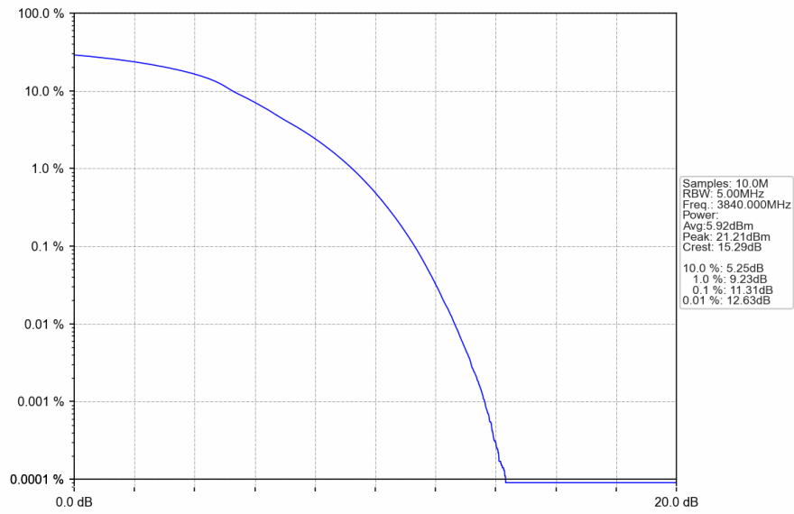
n77a_30kHz_SISO_NTNV_60MHz_DFT-s-OFDM_64_QAM_3840MHz_Outer_Full
