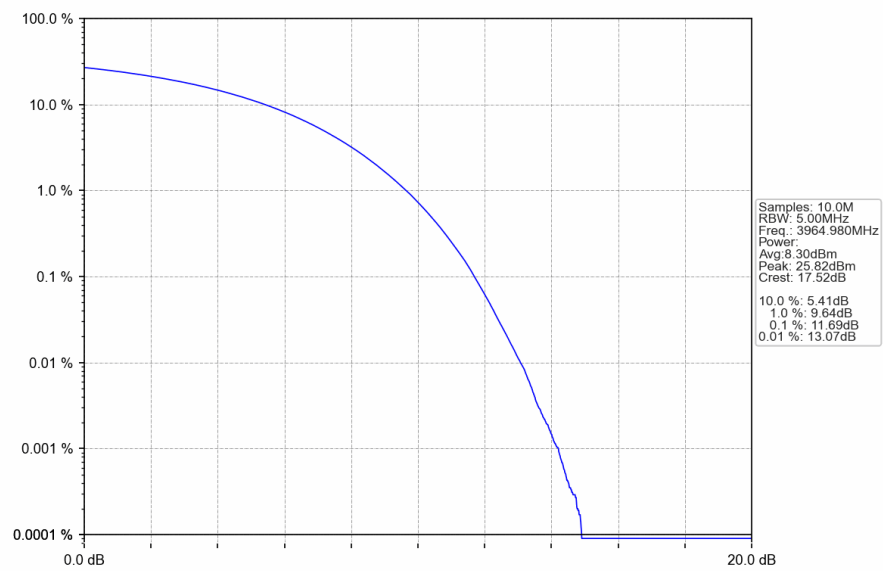
n77a 30kHz SISO NTN 30MHz CP-OFDM QPSK 3964.98MHz Outer Full
