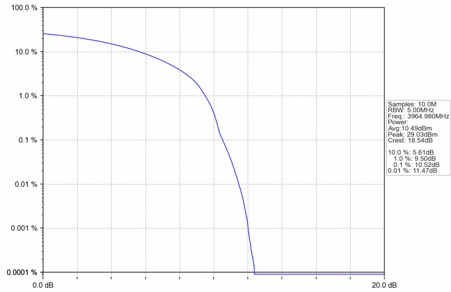
n77a_30kHz_SISO_NTNV_30MHz_DFT-s-OFDM_QPSK_3964.98MHz_Outer_Full
