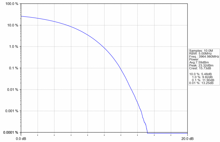
n77a_30kHz_SISO_NTNV_30MHz_CP-OFDM 64 QAM_3964.98MHz_Outer_Full
