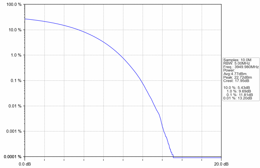
n77a_30kHz_SISO_NTNV_60MHz_CP-OFDM_64_QAM_3949.98MHz_Outer_Full
