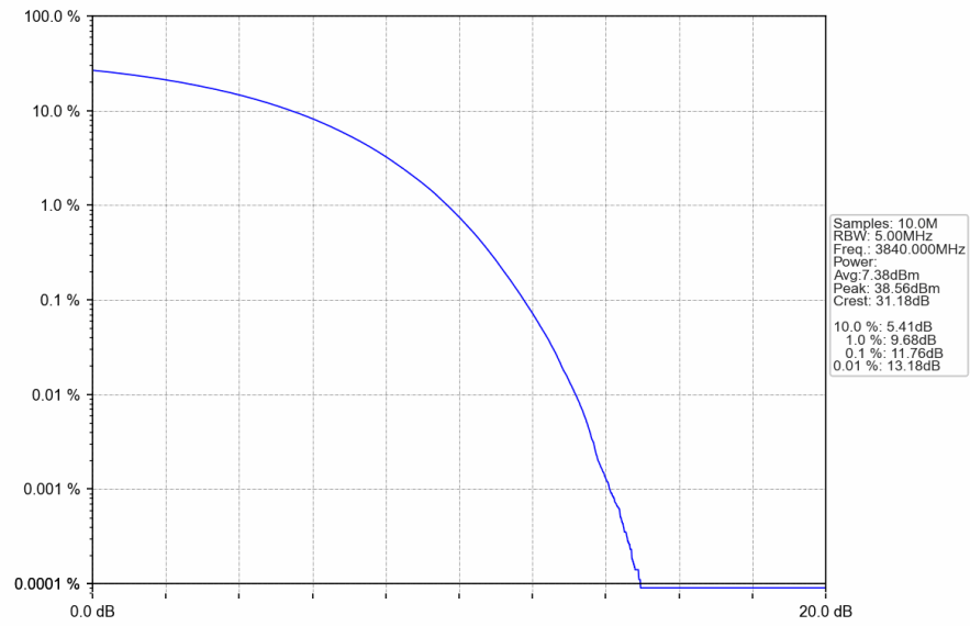
n77a_30kHz_SISO_NTNV_40MHz_CP-OFDM_QPSK_3840MHz_Outer_Full
