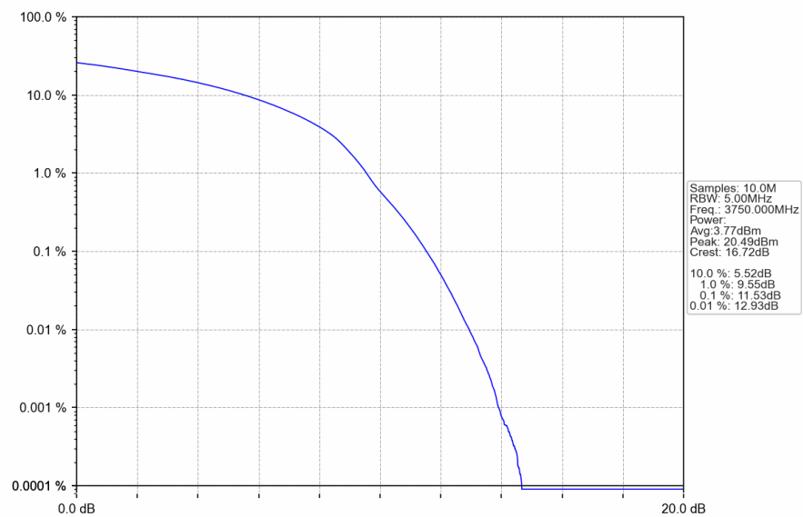
n77a_30kHz_SISO_NTNV_100MHz_DFT-s-OFDM_64_QAM_3750MHz_Outer_Full
