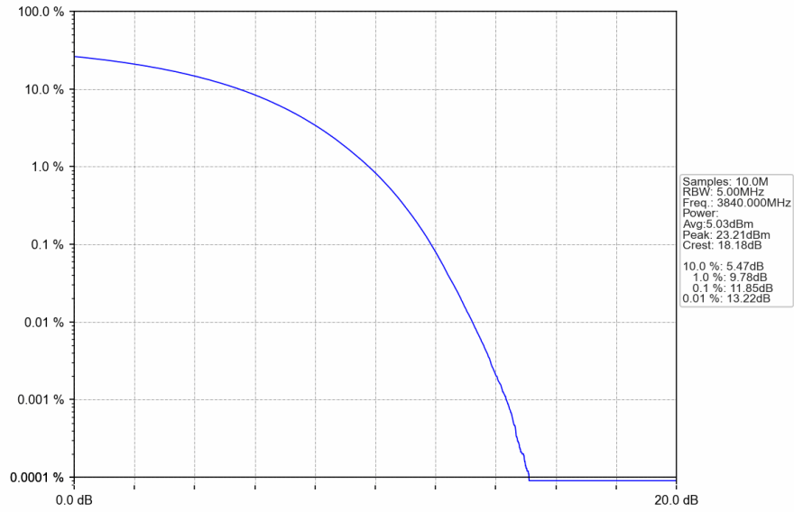
n77a_30kHz_SISO_NTNV_30MHz_CP-OFDM_256_QAM_3840MHz_Outer_Full
