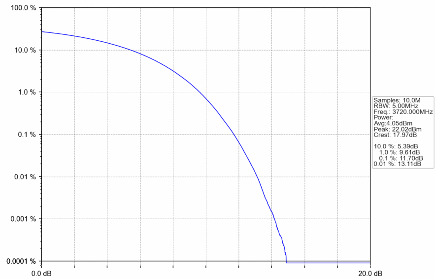
n77a 30kHz SISO NTN 40MHz CP-OFDM 256 QAM 3720MHz Outer Full
