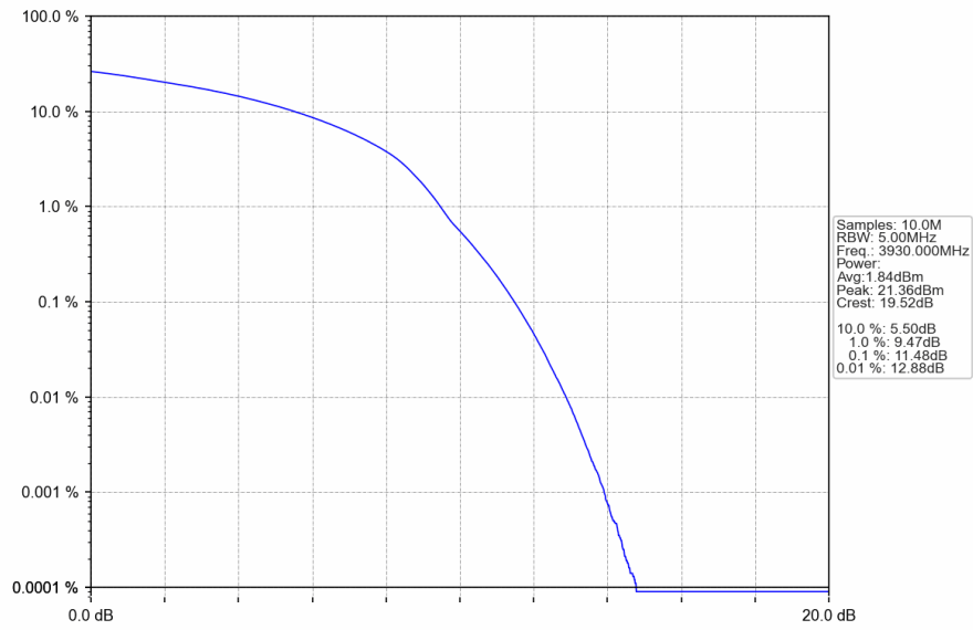
n77a_30kHz_SISO_NTNV_100MHz_DFT-s-OFDM_256_QAM_3930MHz_Outer_Full
