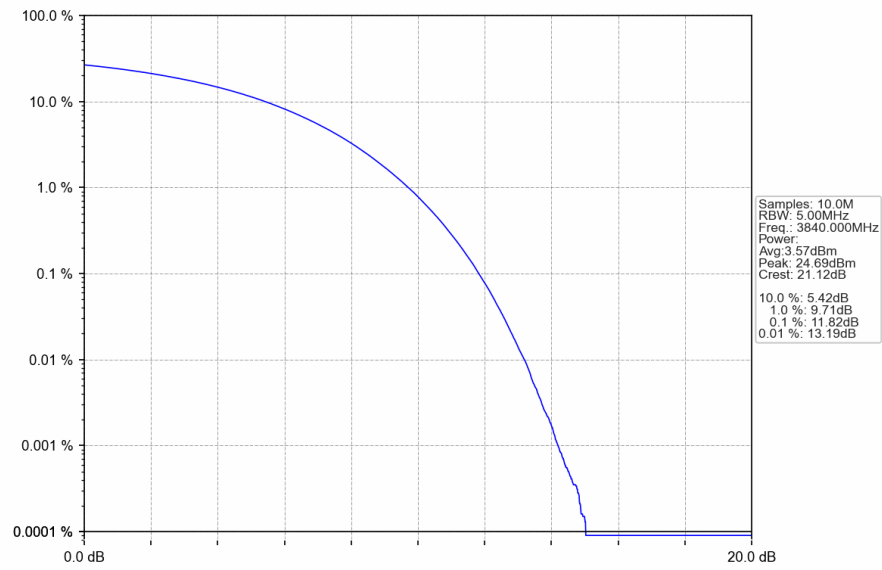
n77a_30kHz_SISO_NTNV_80MHz_CP-OFDM_64_QAM_3840MHz_Outer_Full
