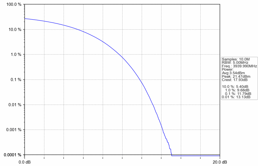
n77a_30kHz_SISO_NTNV_80MHz_CP-OFDM 64 QAM_3939.99MHz_Outer_Full
