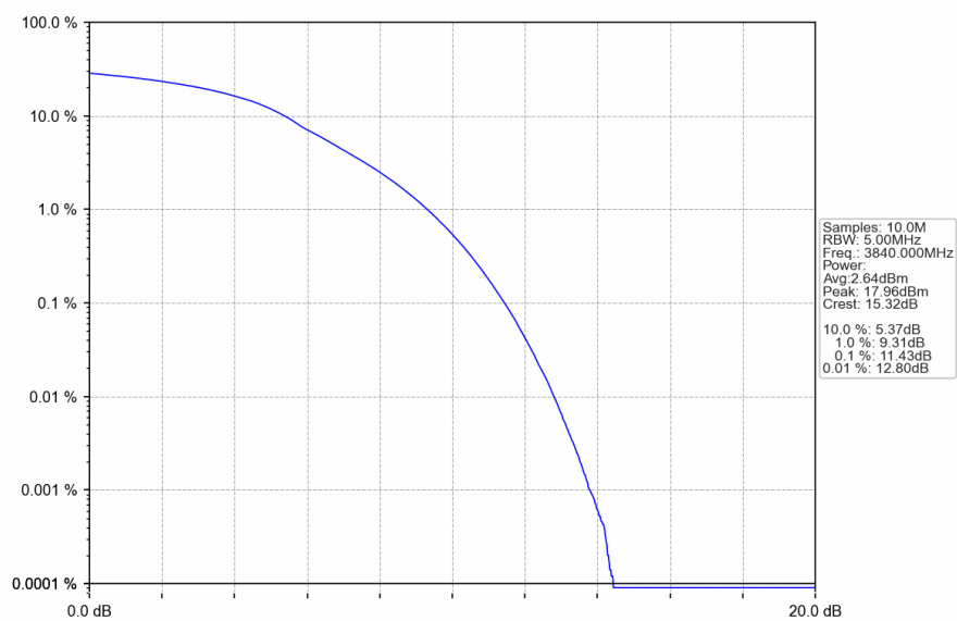
n77a_30kHz_SISO_NTNV_80MHz_DFT-s-OFDM_256_QAM_3840MHz_Outer_Full
