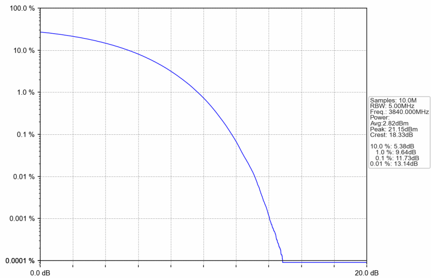
n77a_30kHz_SISO_NTNV_100MHz_CP-OFDM_64_QAM_3840MHz_Outer_Full
