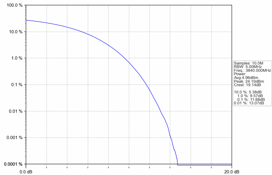
n77a_30kHz_SISO_NTNV_60MHz_CP-OFDM_64_QAM_3840MHz_Outer_Full
