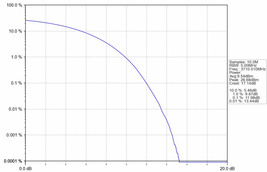
n77a_30kHz_SISO_NTNV_20MHz_CP-OFDM 64 QAM_3710.01MHz_Outer_Full
