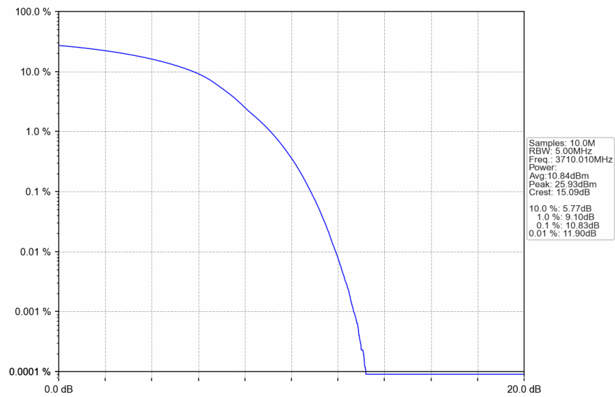
n77a_30kHz_SISO_NTNV_20MHz_DFT-s-OFDM_64_QAM_3710.01MHz_Outer_Full
