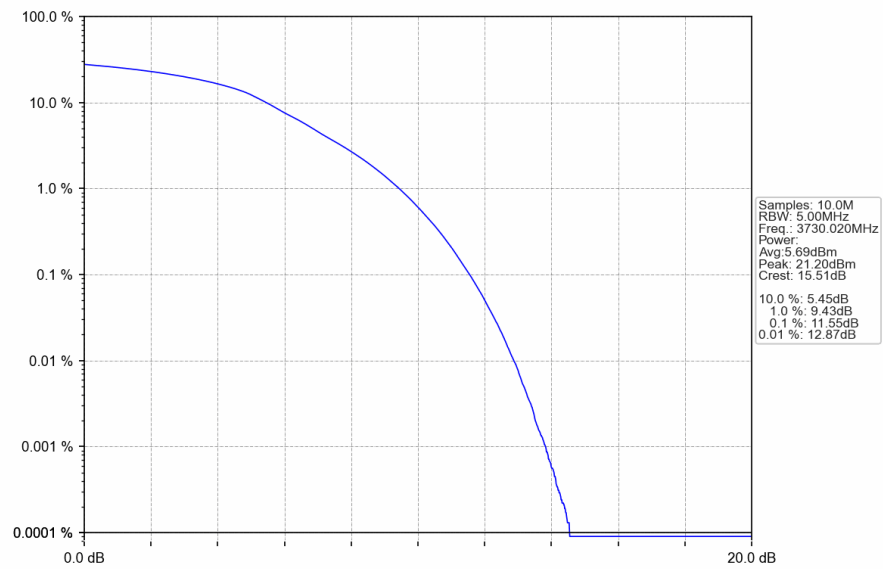
n77a_30kHz_SISO_NTNV_60MHz_DFT-s-OFDM_64_QAM_3730.02MHz_Outer_Full
