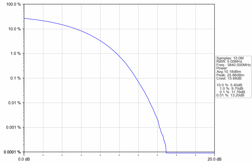
n77a 30kHz SISO_NTNV_20MHz_CP-OFDM QPSK_3840MHz_Outer_Full
