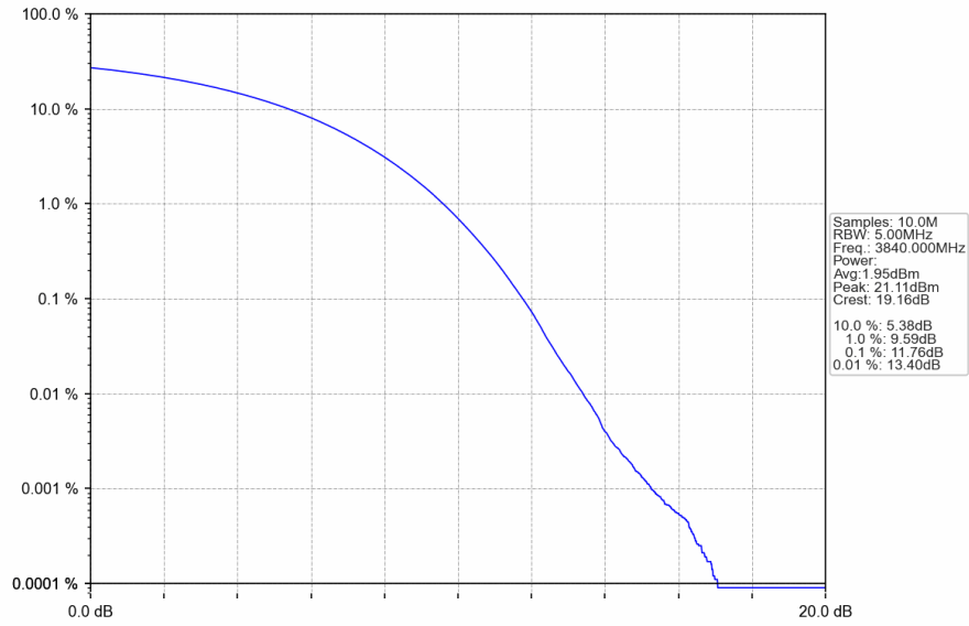
n77a_30kHz_SISO_NTNV_60MHz_CP-OFDM_256_QAM_3840MHz_Outer_Full
