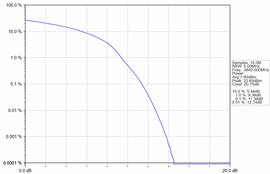
n77a_30kHz_SISO_NTNV_100MHz_DFT-s-OFDM_256_QAM_3840MHz_Outer_Full
