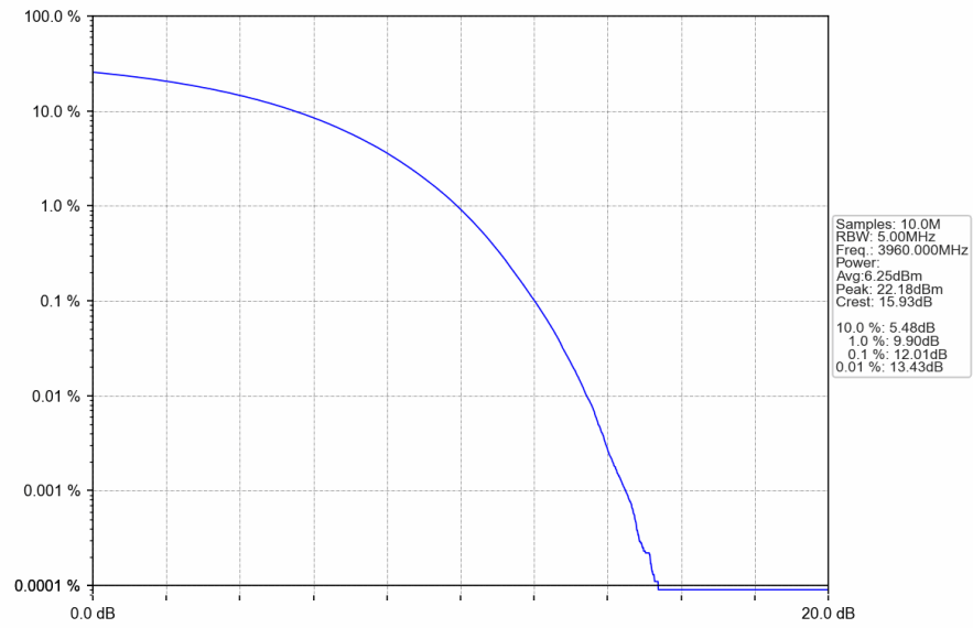
n77a 30kHz SISO NTN 40MHz CP-OFDM 64 QAM 3960MHz Outer Full
