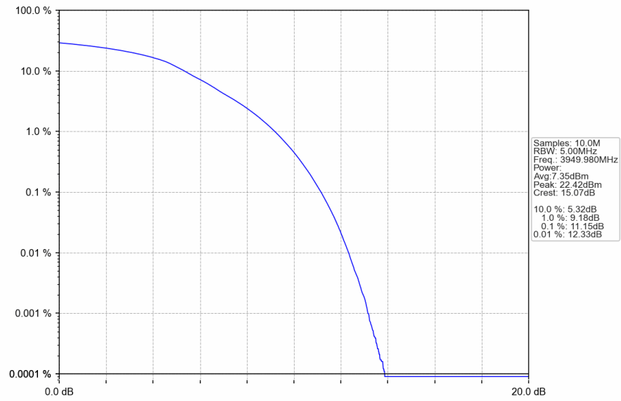
n77a_30kHz_SISO_NTNV_60MHz_DFT-s-OFDM_QPSK_3949.98MHz_Outer_Full
