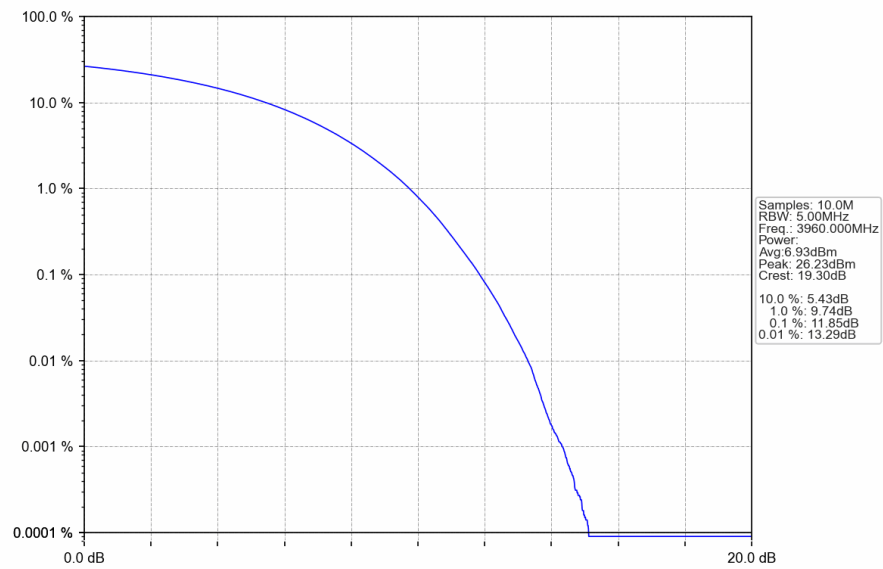
n77a_30kHz_SISO_NTNV_40MHz_CP-OFDM_QPSK_3960MHz_Outer_Full
