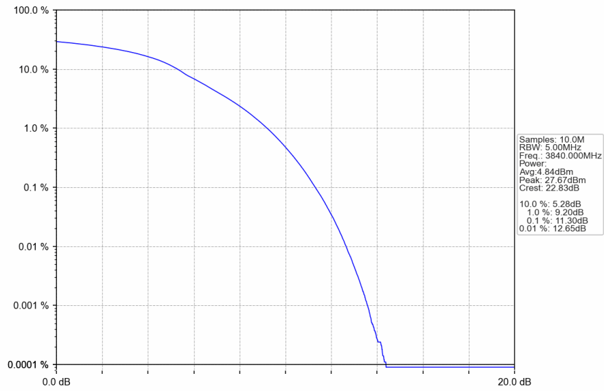
n77a_30kHz_SISO_NTNV_80MHz_DFT-s-OFDM_64_QAM_3840MHz_Outer_Full
