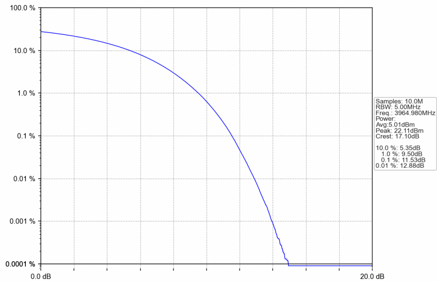
n77a_30kHz_SISO_NTNV_30MHz_CP-OFDM_256_QAM_3964.98MHz_Outer_Full
