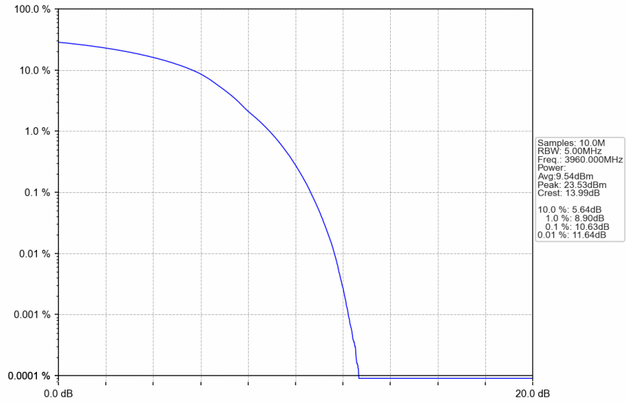
n77a_30kHz_SISO_NTNV_40MHz_DFT-s-OFDM_QPSK_3960MHz_Outer_Full
