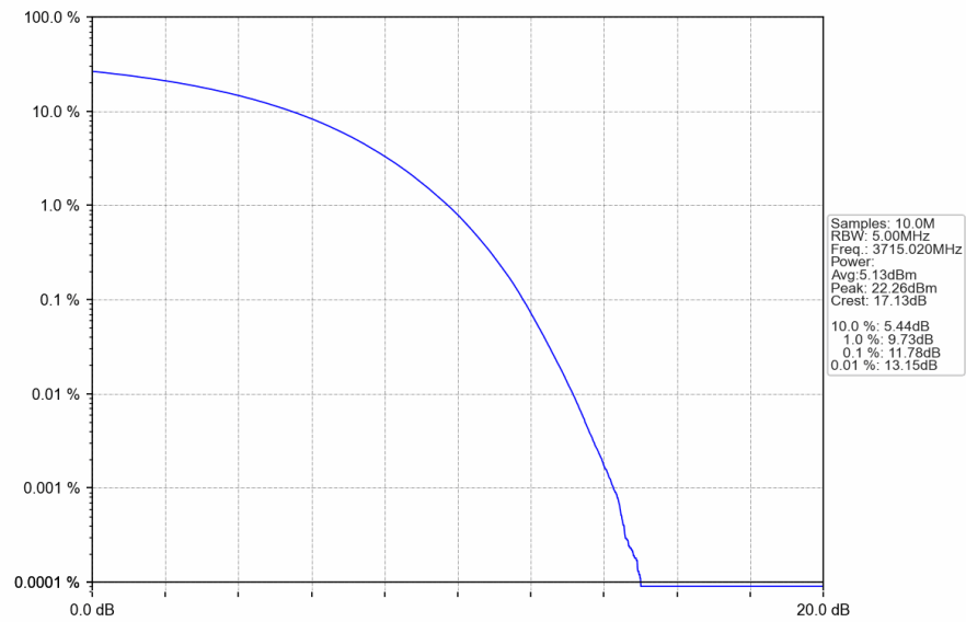
n77a_30kHz_SISO_NTNV_30MHz_CP-OFDM 256 QAM_3715.02MHz_Outer_Full
