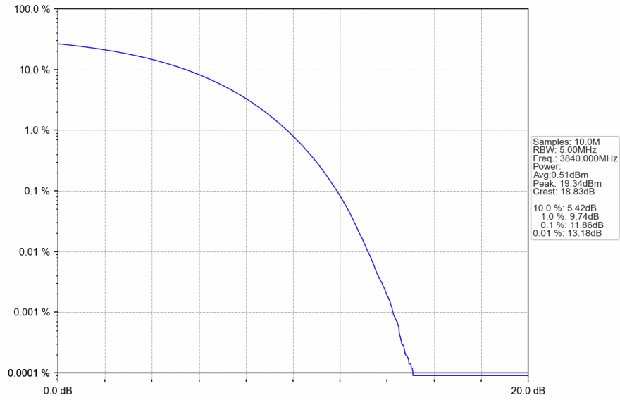
n77a_30kHz_SISO_NTNV_80MHz_CP-OFDM_256_QAM_3840MHz_Outer_Full
