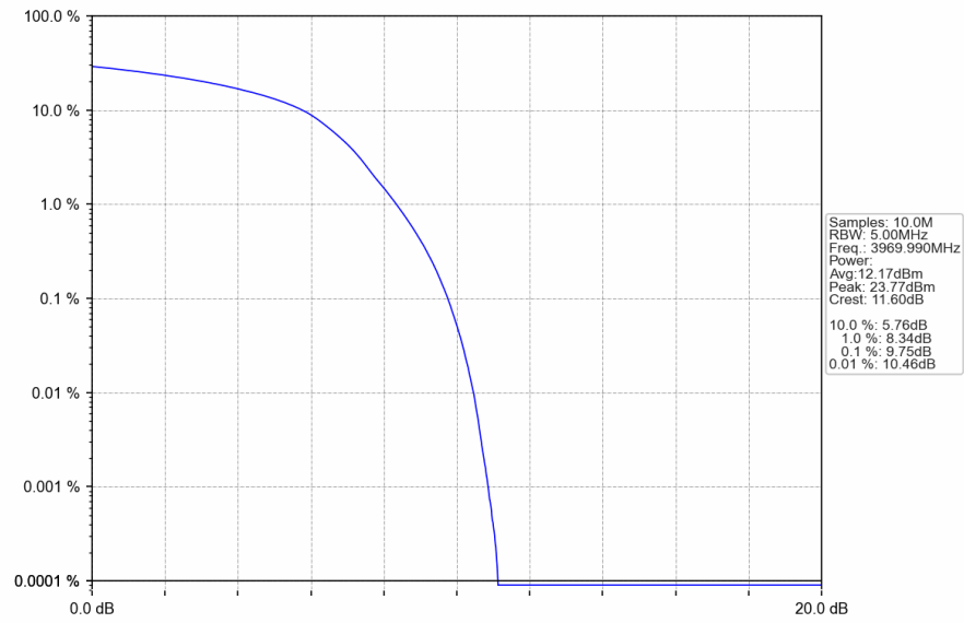
n77a_30kHz_SISO_NTNV_20MHz_DFT-s-OFDM_QPSK_3969.99MHz_Outer_Full
