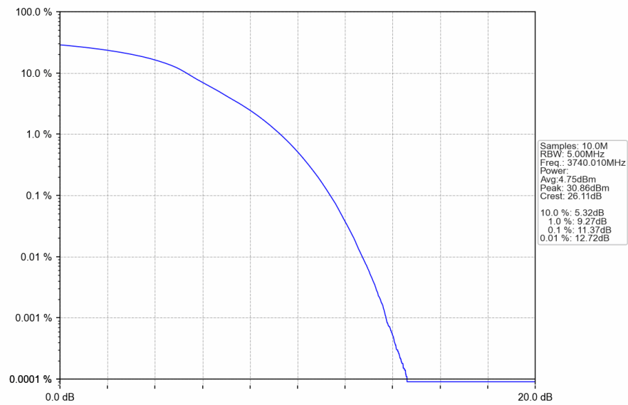
n77a_30kHz_SISO_NTNV_80MHz_DFT-s-OFDM_64_QAM_3740.01MHz_Outer_Full
