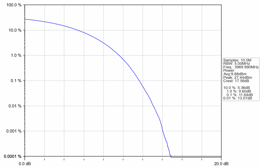
n77a 30kHz SISO_NTNV_20MHz_CP-OFDM QPSK_3969.99MHz_Outer_Full
