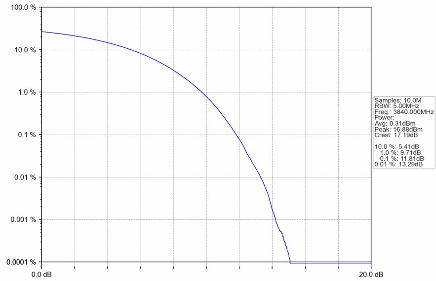
n77a_30kHz_SISO_NTNV_100MHz_CP-OFDM_256_QAM_3840MHz_Outer_Full
