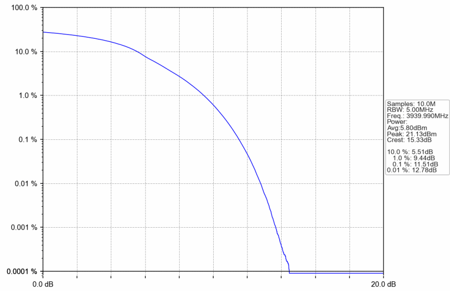
n77a_30kHz_SISO_NTNV_80MHz_DFT-s-OFDM_QPSK_3939.99MHz_Outer_Full
