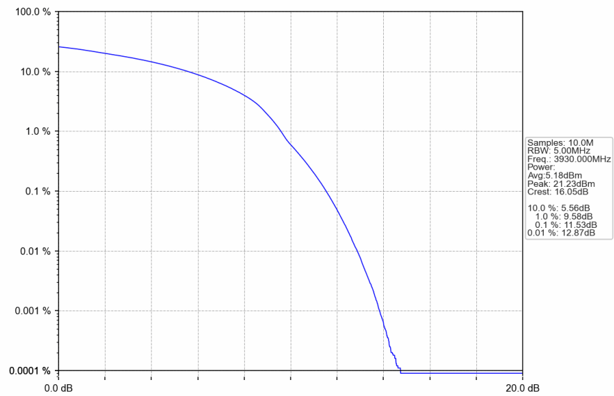
n77a_30kHz_SISO_NTNV_100MHz_DFT-s-OFDM_QPSK_3930MHz_Outer_Full
