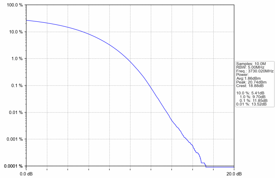
n77a_30kHz_SISO_NTNV_60MHz_CP-OFDM_256_QAM_3730.02MHz_Outer_Full
