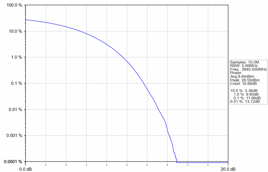
n77a_30kHz_SISO_NTNV_20MHz_CP-OFDM 64 QAM_3840MHz_Outer_Full
