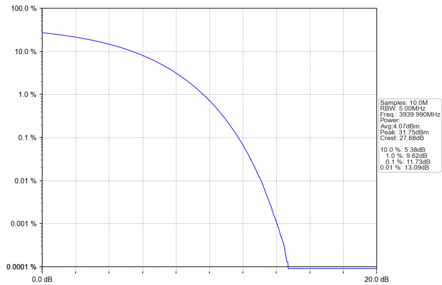
n77a_30kHz_SISO_NTNV_80MHz_CP-OFDM_QPSK_3939.99MHz_Outer_Full
