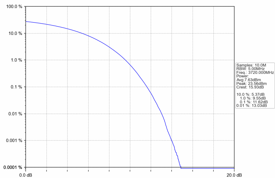
n77a_30kHz_SISO_NTNV_40MHz_CP-OFDM_QPSK_3720MHz_Outer_Full
