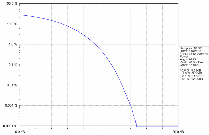
n77a_30kHz_SISO_NTNV_80MHz_CP-OFDM_QPSK_3840MHz_Outer_Full
