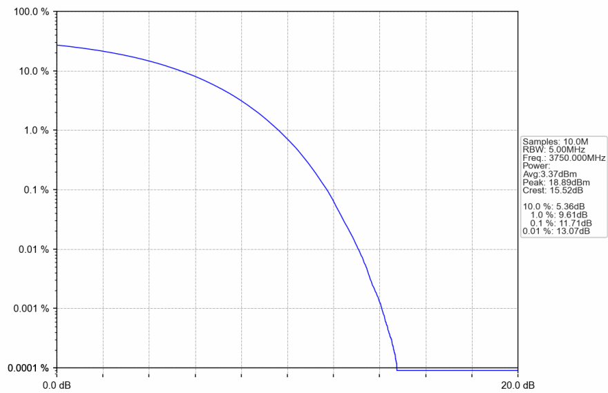
n77a_30kHz_SISO_NTNV_100MHz_CP-OFDM_QPSK_3750MHz_Outer_Full
