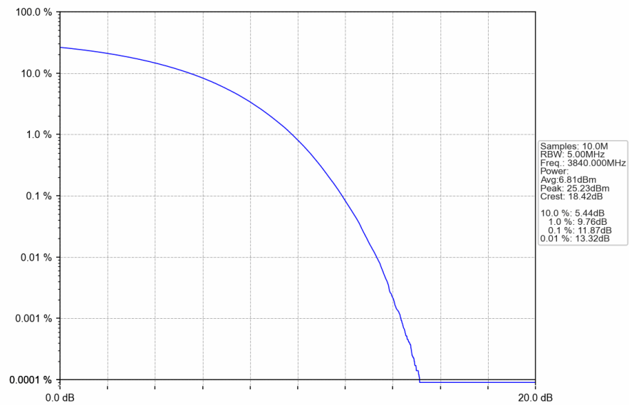
n77a_30kHz_SISO_NTNV_40MHz_CP-OFDM_64_QAM_3840MHz_Outer_Full
