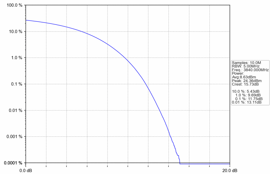
n77a 30kHz SISO NTN 30MHz CP-OFDM QPSK 3840MHz Outer Full
