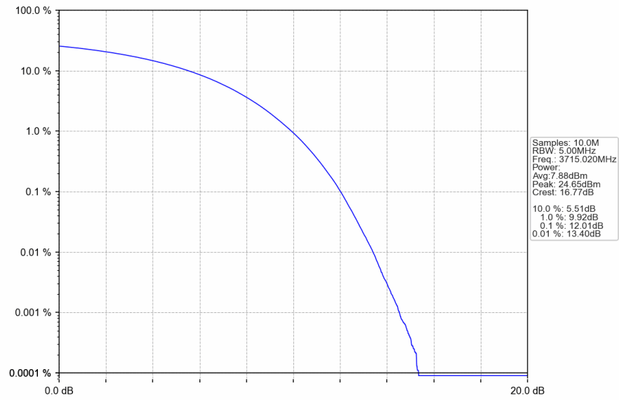
n77a_30kHz_SISO_NTNV_30MHz_CP-OFDM_64_QAM_3715.02MHz_Outer_Full
