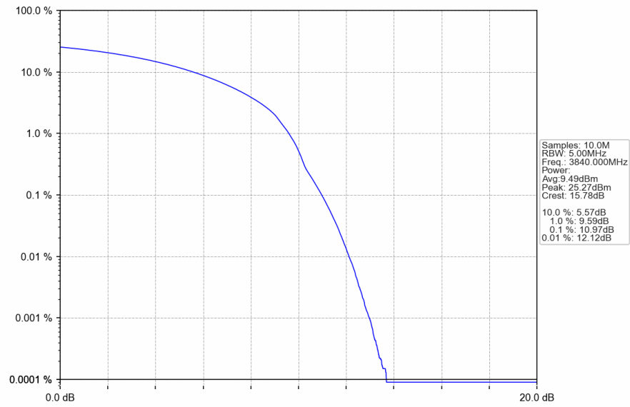
n77a_30kHz_SISO_NTNV_30MHz_DFT-s-OFDM_64_QAM_3840MHz_Outer_Full
