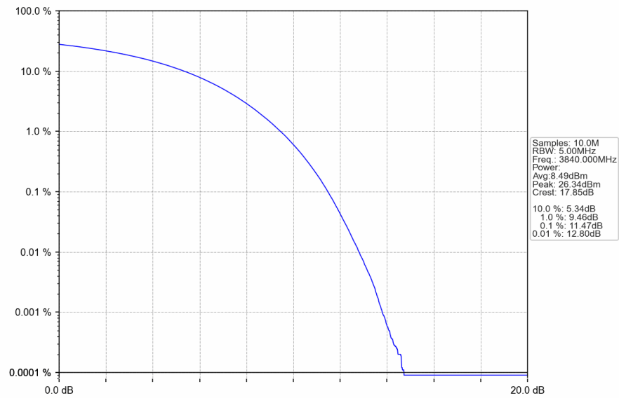
n77a_30kHz_SISO_NTNV_30MHz_CP-OFDM_64_QAM_3840MHz_Outer_Full
