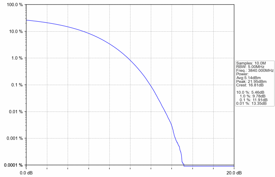
n77a_30kHz_SISO_NTNV_60MHz_CP-OFDM_QPSK_3840MHz_Outer_Full
