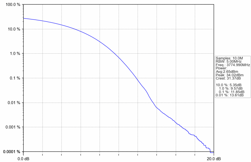
n78a_30kHz_SISO_NTNV_50MHz_CP-OFDM_256_QAM_3774.99MHz_Outer_Full
