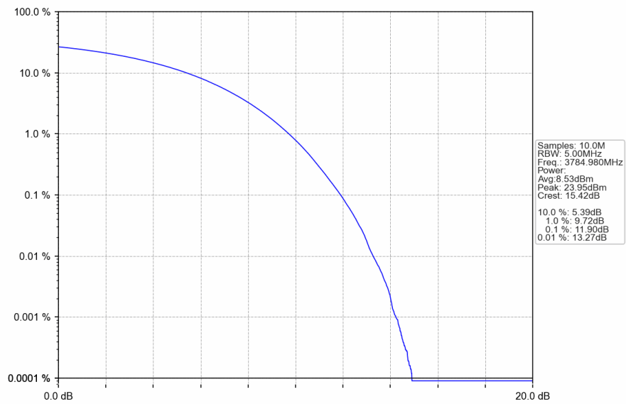
n78a 30kHz SISO NTN 30MHz CP-OFDM QPSK 3784.98MHz Outer Full
