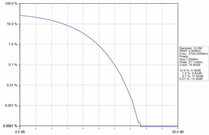
n78a_30kHz_SISO_NTNV_40MHz_CP-OFDM_QPSK_3750MHz_Outer_Full
