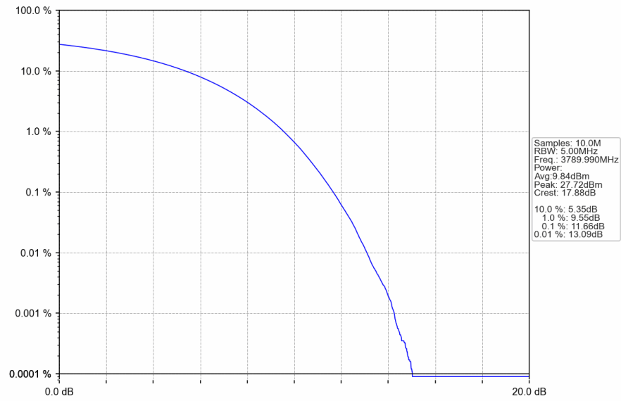
n78a_30kHz_SISO_NTNV_20MHz_CP-OFDM 64 QAM_3789.99MHz_Outer_Full
