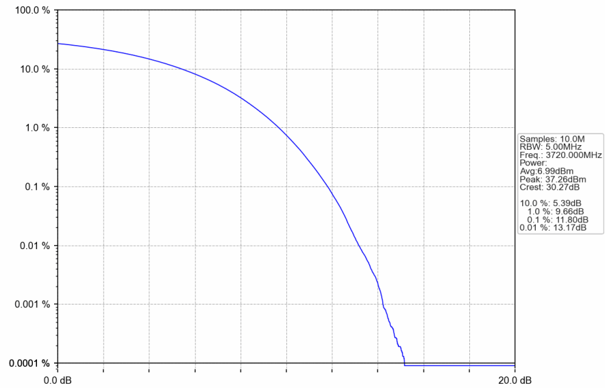
n78a_30kHz_SISO_NTNV_40MHz_CP-OFDM_64_QAM_3720MHz_Outer_Full
