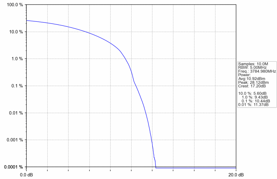
n78a_30kHz_SISO_NTNV_30MHz_DFT-s-OFDM QPSK_3784.98MHz_Outer_Full
