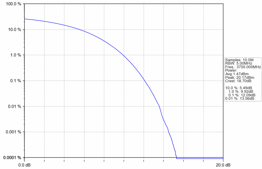
n78a_30kHz_SISO_NTNV_60MHz_CP-OFDM_256_QAM_3750MHz_Outer_Full
