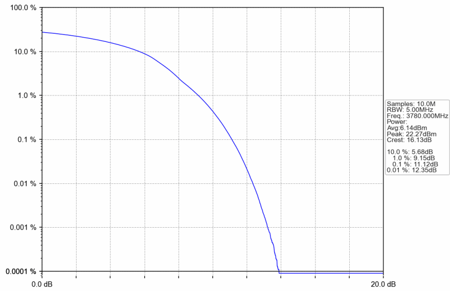
n78a_30kHz_SISO_NTNV_40MHz_DFT-s-OFDM_256_QAM_3780MHz_Outer_Full
