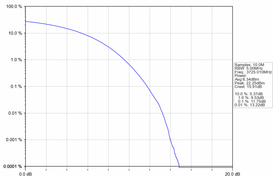
n78a_30kHz_SISO_NTNV_50MHz_CP-OFDM_QPSK_3725.01MHz_Outer_Full
