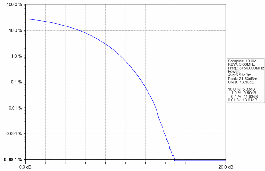
n78a_30kHz_SISO_NTNV_60MHz_CP-OFDM_QPSK_3750MHz_Outer_Full
