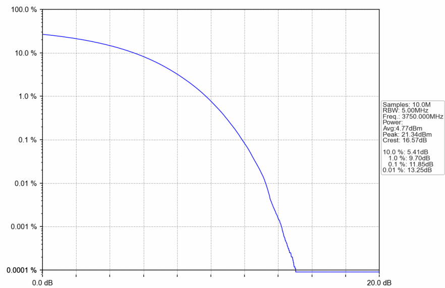
n78a 30kHz SISO NTN 60MHz CP-OFDM 64 QAM 3750MHz Outer Full
