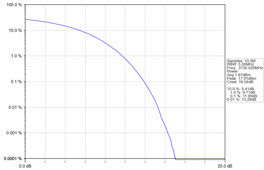
n78a_30kHz_SISO_NTNV_60MHz_CP-OFDM 256 QAM_3730.02MHz_Outer_Full
