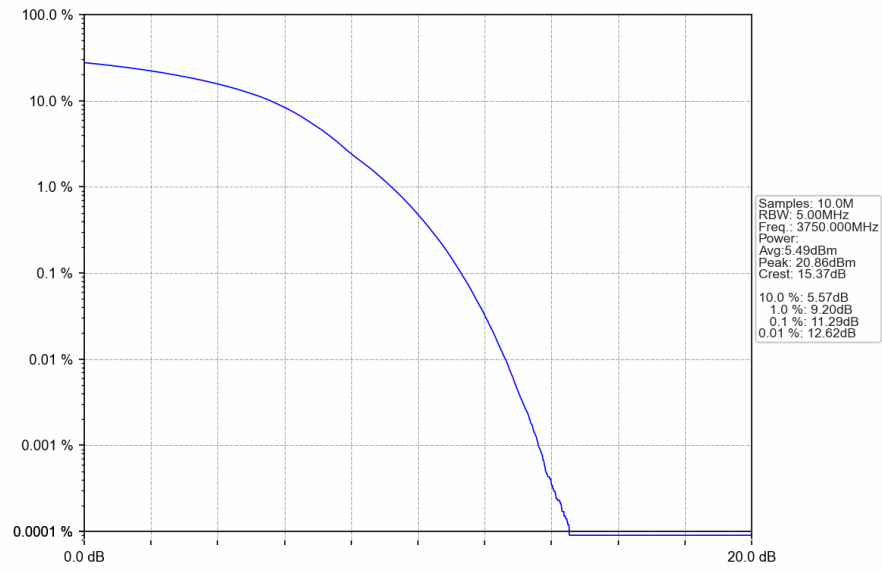
n78a_30kHz_SISO_NTNV_70MHz_DFT-s-OFDM_64_QAM_3750MHz_Outer_Full
