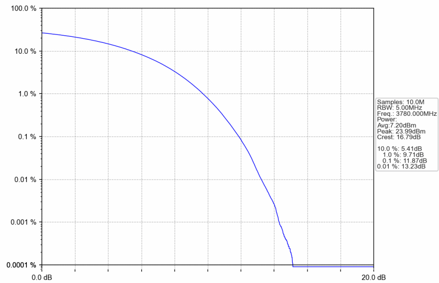
n78a_30kHz_SISO_NTNV_40MHz_CP-OFDM_QPSK_3780MHz_Outer_Full
