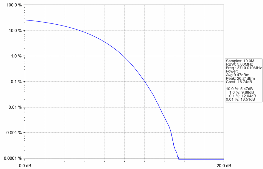
n78a 30kHz SISO NTN 20MHz CP-OFDM 64 QAM 3710.01MHz Outer Full
