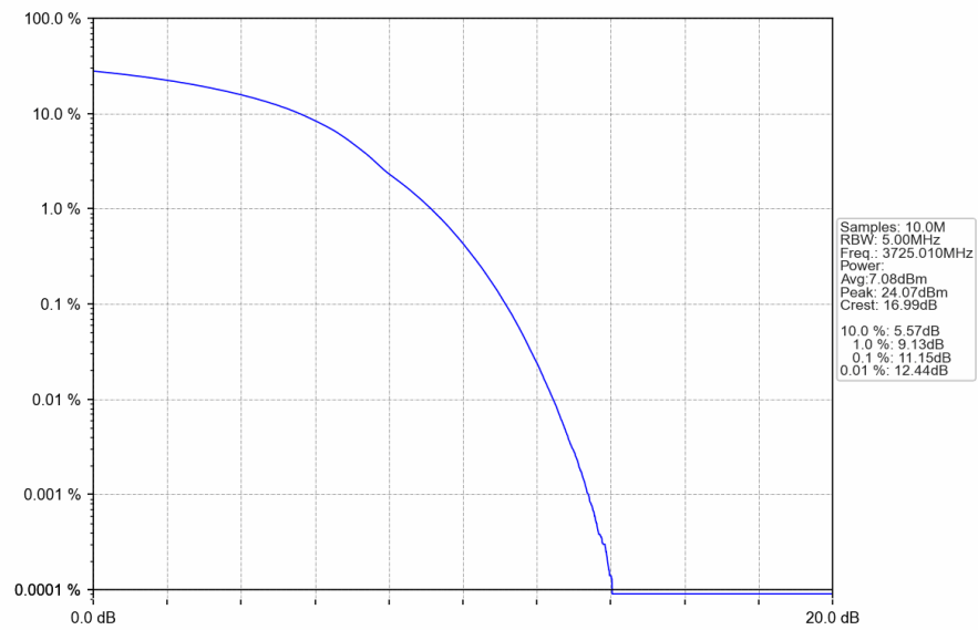
n78a_30kHz_SISO_NTNV_50MHz_DFT-s-OFDM_64_QAM_3725.01MHz_Outer_Full
