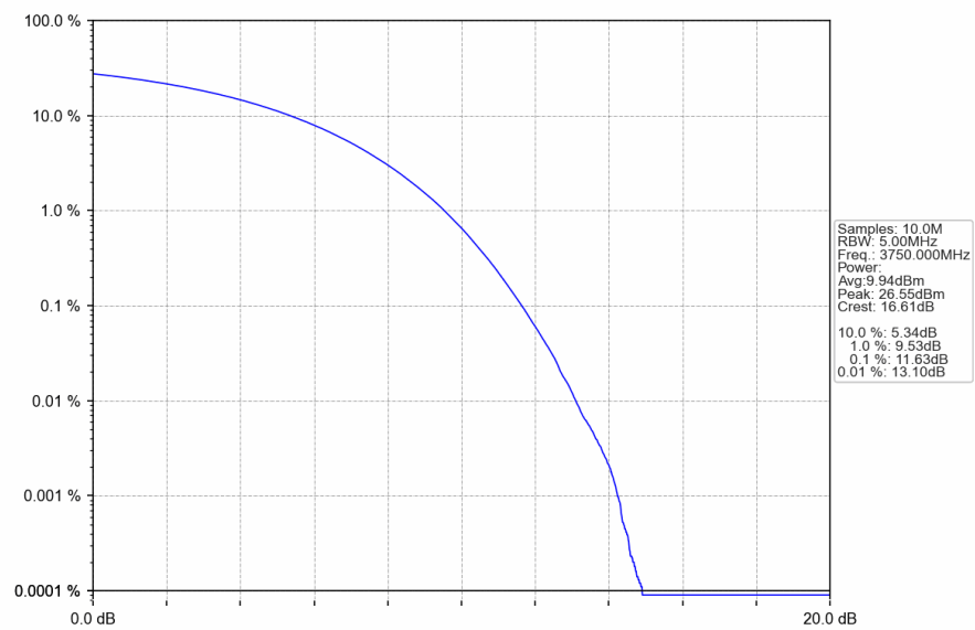
n78a 30kHz SISO NTN 20MHz CP-OFDM 64 QAM 3750MHz Outer Full
