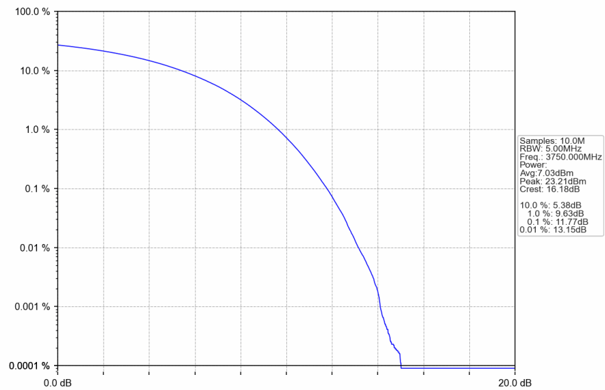
n78a_30kHz_SISO_NTNV_40MHz_CP-OFDM_64_QAM_3750MHz_Outer_Full
