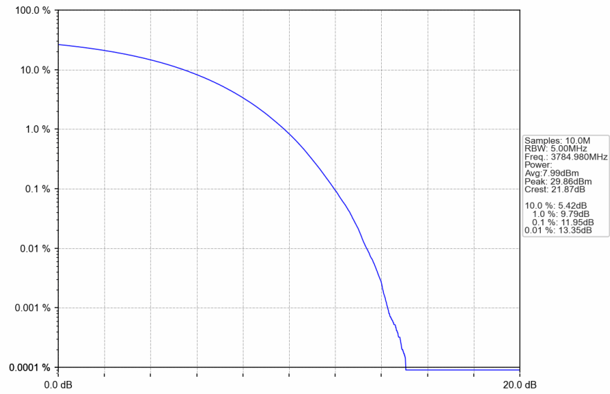
n78a_30kHz_SISO_NTNV_30MHz_CP-OFDM 64 QAM_3784.98MHz_Outer_Full
