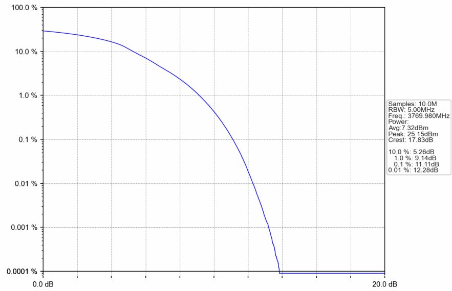
n78a_30kHz_SISO_NTNV_60MHz_DFT-s-OFDM_QPSK_3769.98MHz_Outer_Full
