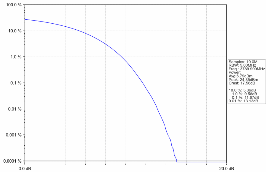
n78a_30kHz_SISO_NTNV_20MHz_CP-OFDM_256_QAM_3789.99MHz_Outer_Full
