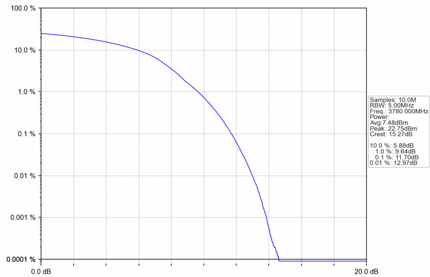
n78a_30kHz_SISO_NTNV_40MHz_DFT-s-OFDM_64_QAM_3780MHz_Outer_Full
