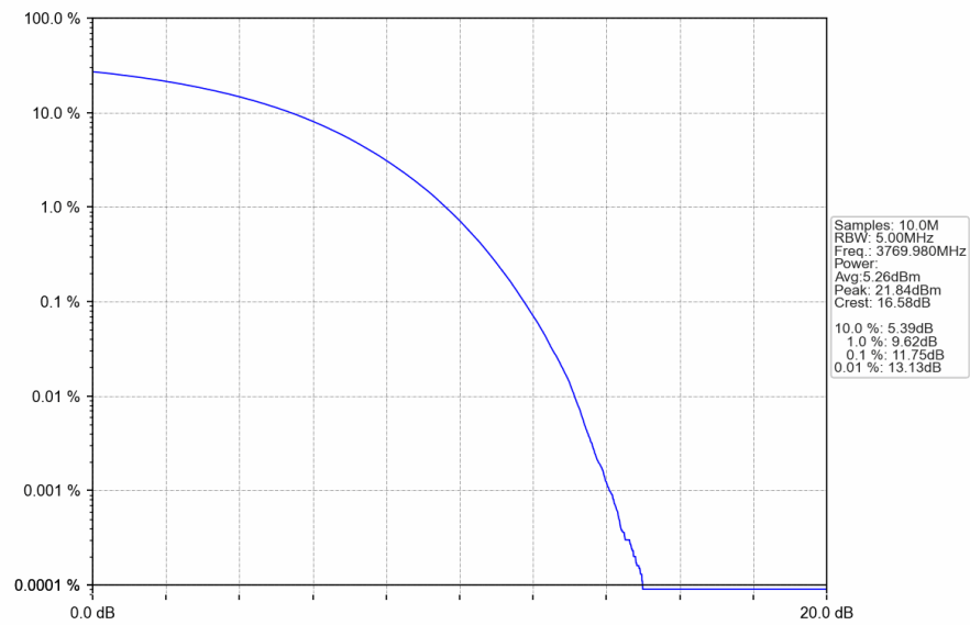
n78a_30kHz_SISO_NTNV_60MHz_CP-OFDM_QPSK_3769.98MHz_Outer_Full
