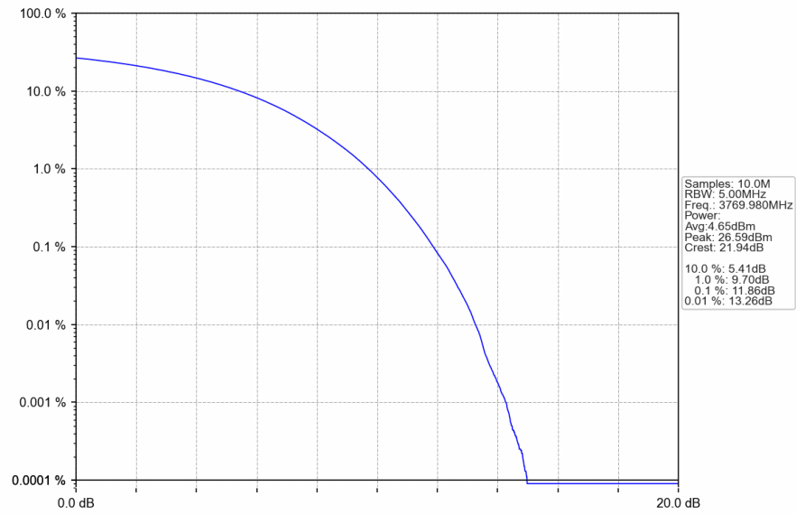
n78a_30kHz_SISO_NTNV_60MHz_CP-OFDM 64 QAM_3769.98MHz_Outer_Full
