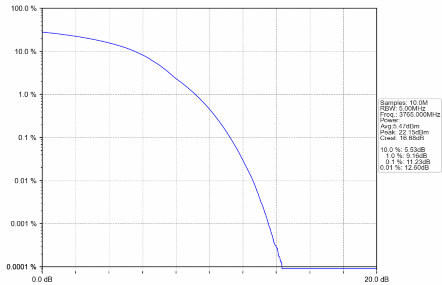
n78a_30kHz_SISO_NTNV_70MHz_DFT-s-OFDM_64_QAM_3765MHz_Outer_Full
