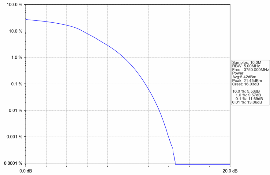
n78a_30kHz_SISO_NTNV_60MHz_DFT-s-OFDM_64_QAM_3750MHz_Outer_Full
