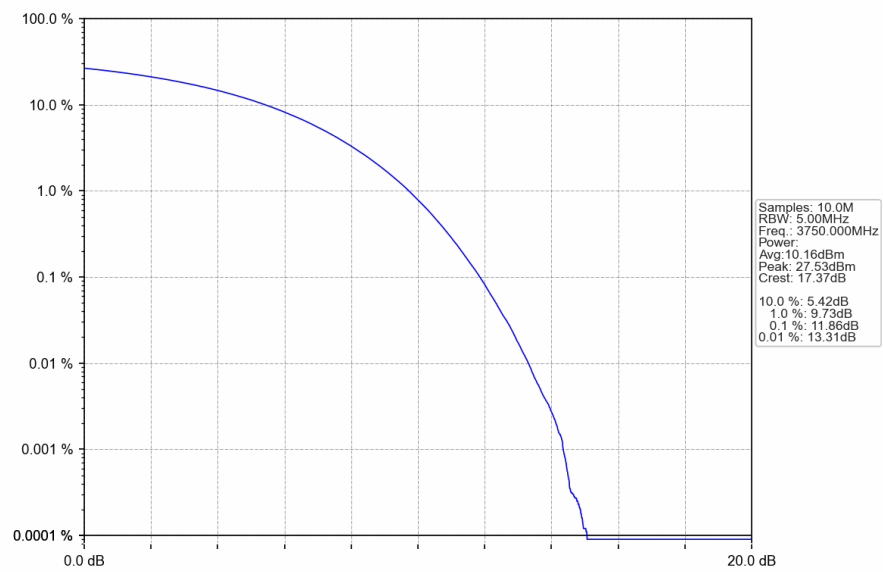
n78a 30kHz SISO_NTNV_20MHz_CP-OFDM QPSK_3750MHz_Outer_Full
