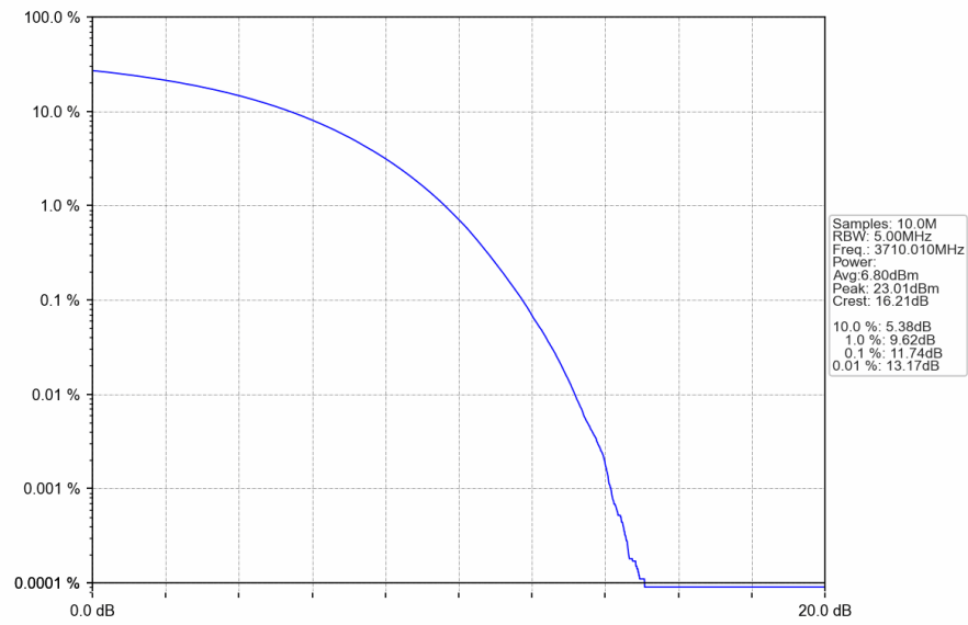
n78a_30kHz_SISO_NTNV_20MHz_CP-OFDM 256 QAM_3710.01MHz_Outer_Full
