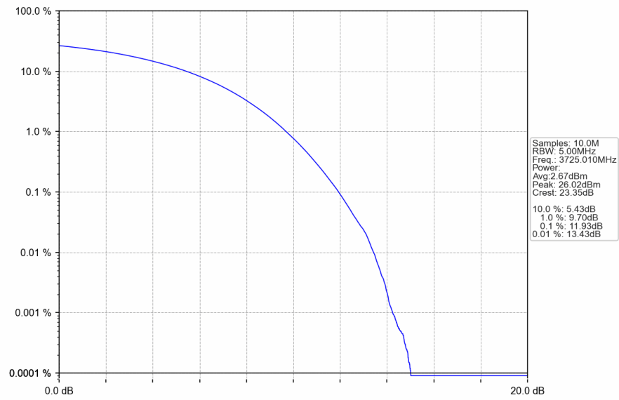
n78a_30kHz_SISO_NTNV_50MHz_CP-OFDM 256 QAM_3725.01MHz_Outer_Full
