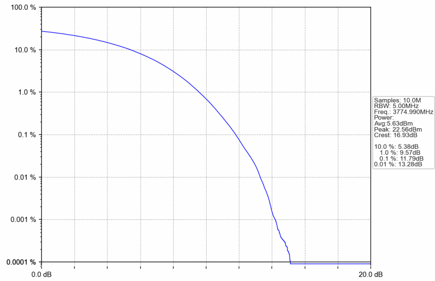
n78a_30kHz_SISO_NTNV_50MHz_CP-OFDM 64 QAM_3774.99MHz_Outer_Full
