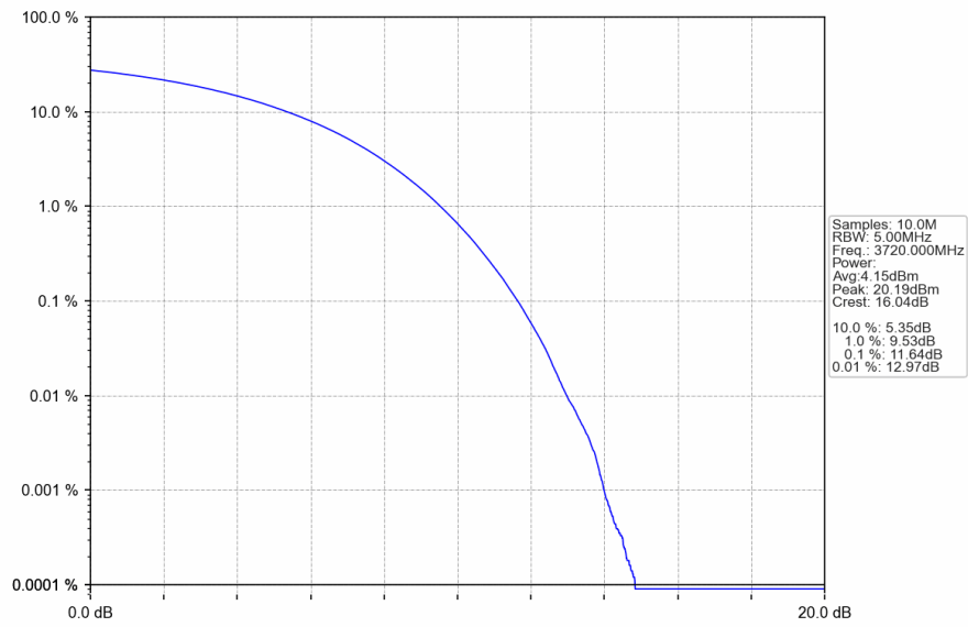
n78a 30kHz SISO NTN 40MHz CP-OFDM 256 QAM 3720MHz Outer Full
