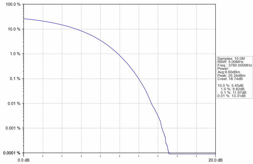
n78a 30kHz SISO NTN 40MHz CP-OFDM 64 QAM 3780MHz Outer Full
