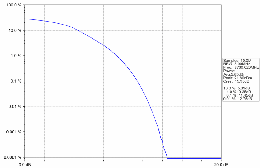
n78a_30kHz_SISO_NTNV_60MHz_DFT-s-OFDM_64_QAM_3730.02MHz_Outer_Full
