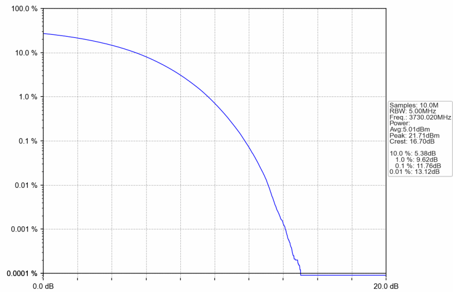
n78a 30kHz SISO NTN 60MHz CP-OFDM 64 QAM 3730.02MHz Outer Full
