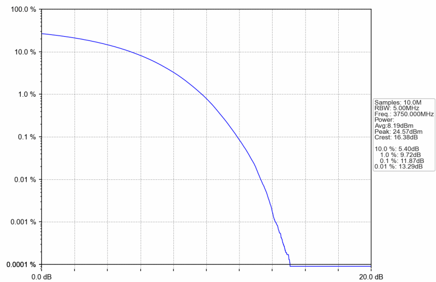
n78a 30kHz SISO NTN 30MHz CP-OFDM 64 QAM 3750MHz Outer Full
