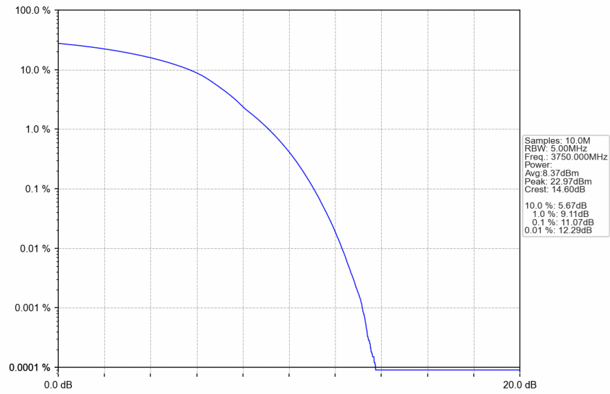
n78a_30kHz_SISO_NTNV_40MHz_DFT-s-OFDM_64_QAM_3750MHz_Outer_Full
