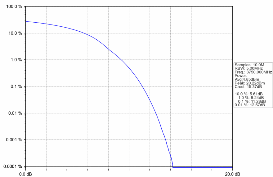
n78a_30kHz_SISO_NTNV_50MHz_DFT-s-OFDM_256_QAM_3750MHz_Outer_Full
