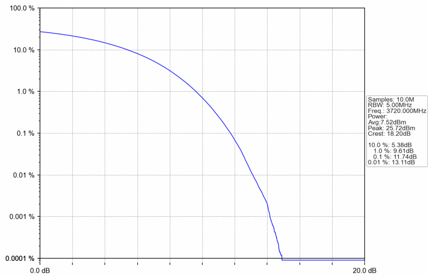
n78a_30kHz_SISO_NTNV_40MHz_CP-OFDM_QPSK_3720MHz_Outer_Full
