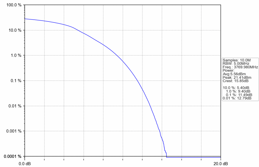
n78a_30kHz_SISO_NTNV_60MHz_DFT-s-OFDM_64_QAM_3769.98MHz_Outer_Full
