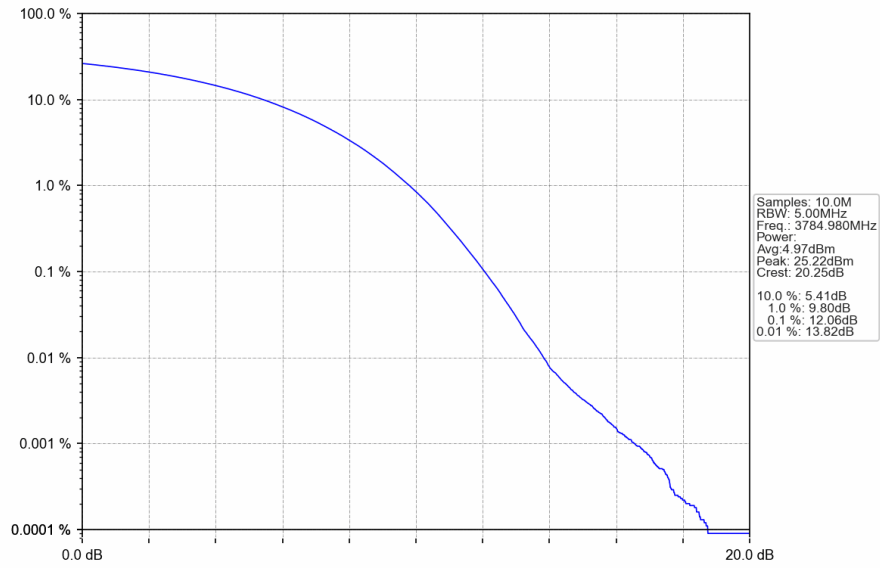
n78a_30kHz_SISO_NTNV_30MHz_CP-OFDM_256_QAM_3784.98MHz_Outer_Full
