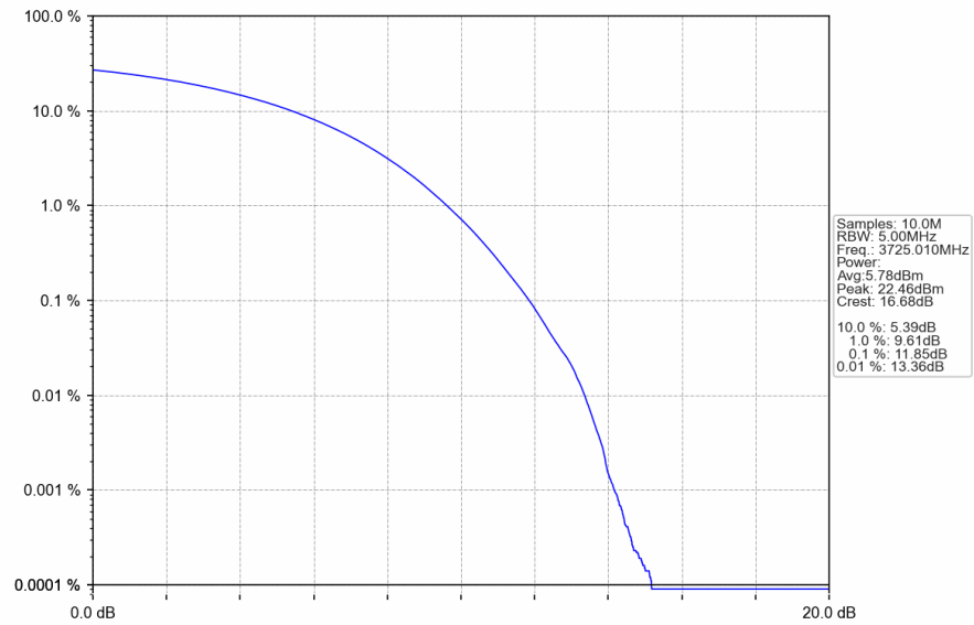
n78a 30kHz SISO NTN 50MHz CP-OFDM 64 QAM 3725.01MHz Outer Full
