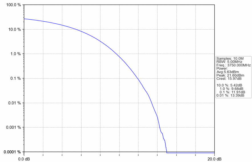
n78a 30kHz SISO NTN 50MHz CP-OFDM 64 QAM 3750MHz Outer Full
