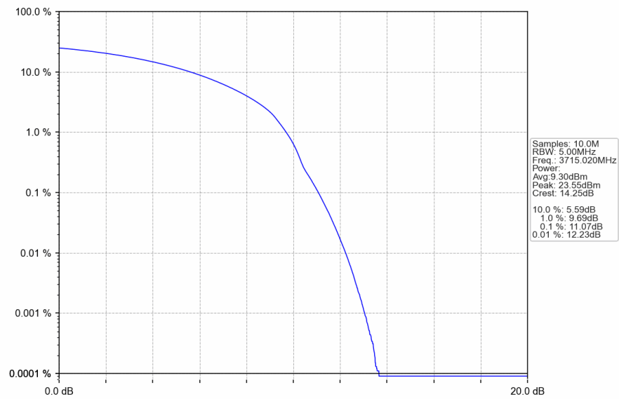
n78a_30kHz_SISO_NTNV_30MHz_DFT-s-OFDM 64 QAM_3715.02MHz_Outer_Full
