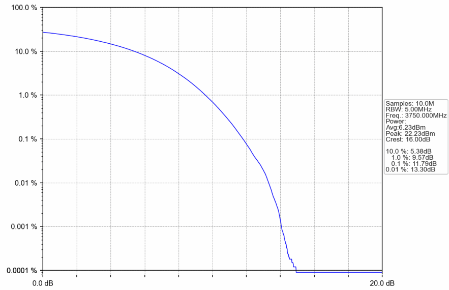
n78a 30kHz SISO NTN 50MHz CP-OFDM QPSK 3750MHz Outer Full
