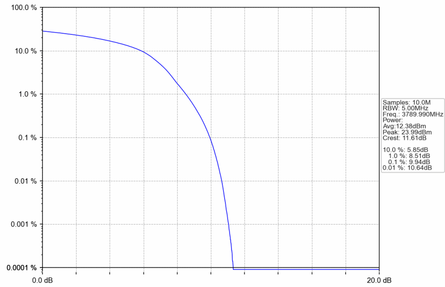
n78a_30kHz_SISO_NTNV_20MHz_DFT-s-OFDM_QPSK_3789.99MHz_Outer_Full
