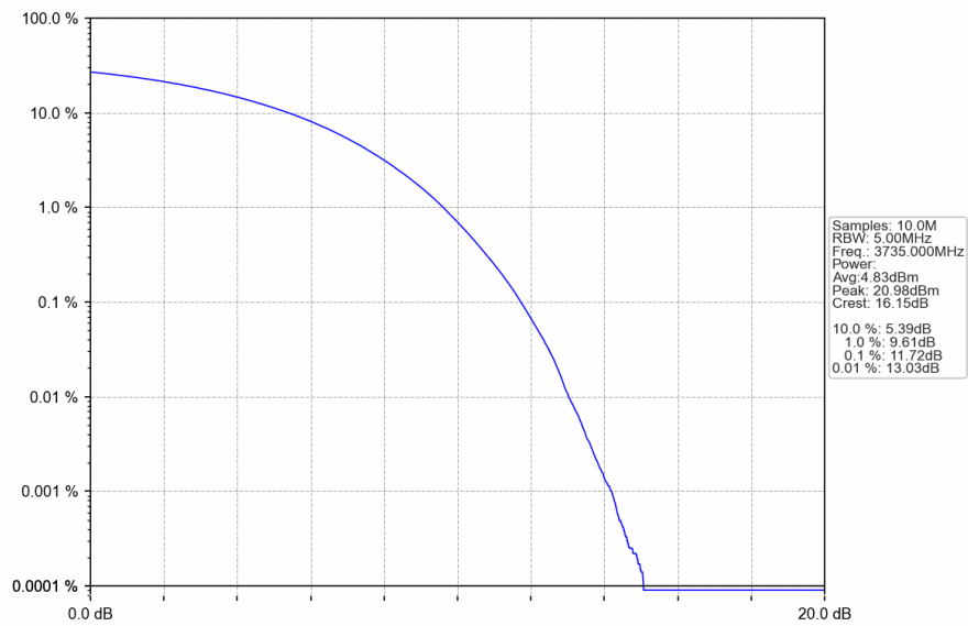
n78a_30kHz_SISO_NTNV_70MHz_CP-OFDM_QPSK_3735MHz_Outer_Full
