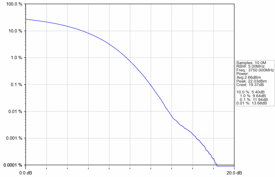
n78a_30kHz_SISO_NTNV_50MHz_CP-OFDM_256_QAM_3750MHz_Outer_Full
