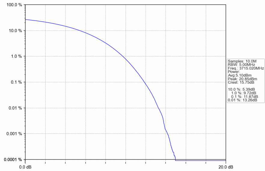
n78a_30kHz_SISO_NTNV_30MHz_CP-OFDM 256 QAM_3715.02MHz_Outer_Full
