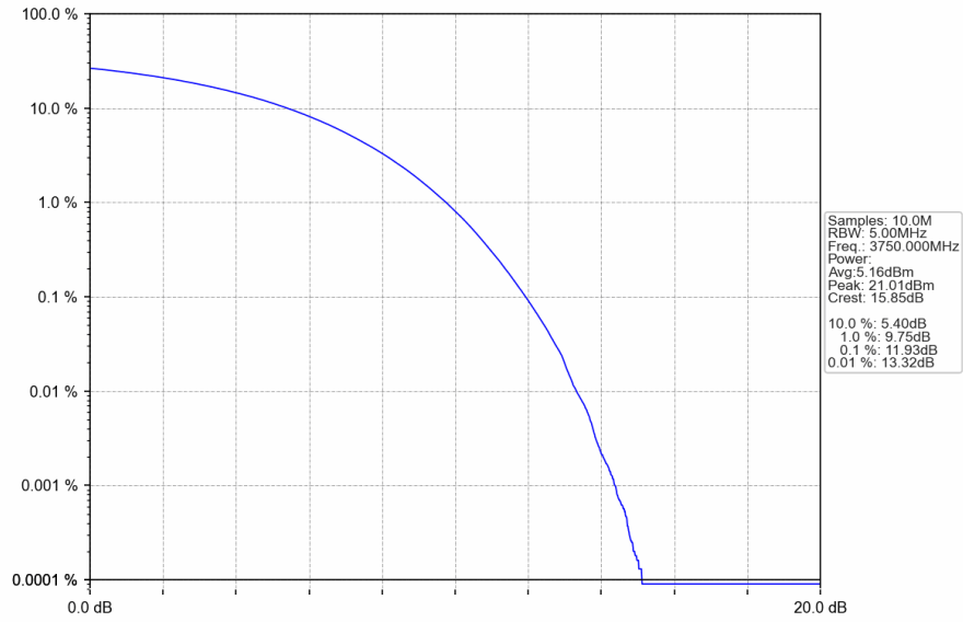
n78a_30kHz_SISO_NTNV_30MHz_CP-OFDM_256_QAM_3750MHz_Outer_Full
