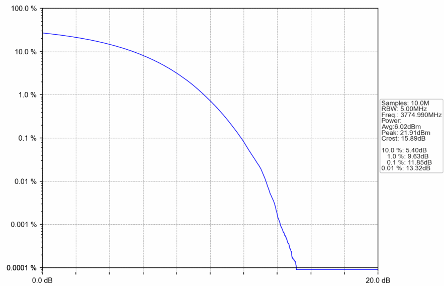
n78a 30kHz SISO NTN 50MHz CP-OFDM QPSK 3774.99MHz Outer Full
