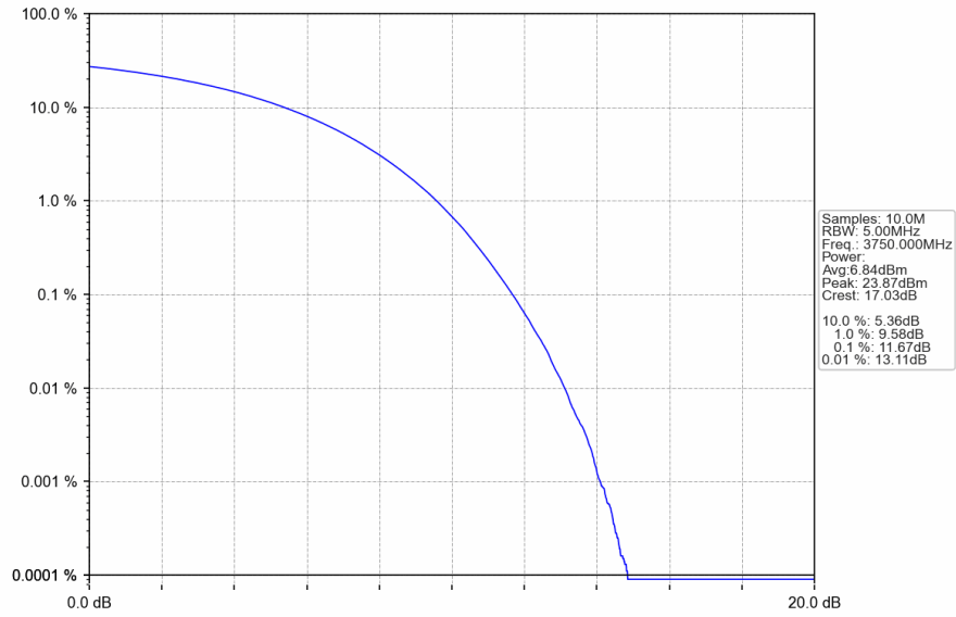
n78a_30kHz_SISO_NTNV_20MHz_CP-OFDM_256_QAM_3750MHz_Outer_Full
