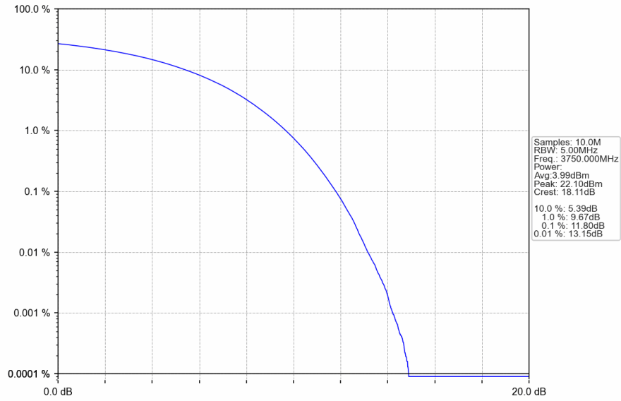
n78a_30kHz_SISO_NTNV_40MHz_CP-OFDM_256_QAM_3750MHz_Outer_Full
