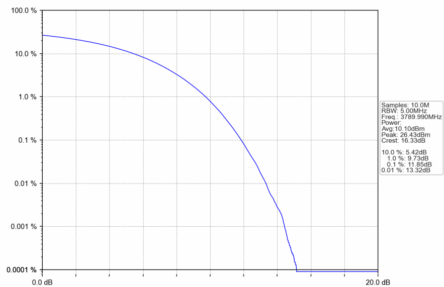
n78a 30kHz SISO_NTNV_20MHz_CP-OFDM QPSK_3789.99MHz_Outer_Full
