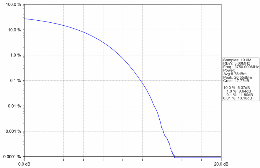
n78a 30kHz SISO NTN 30MHz CP-OFDM QPSK 3750MHz Outer Full
