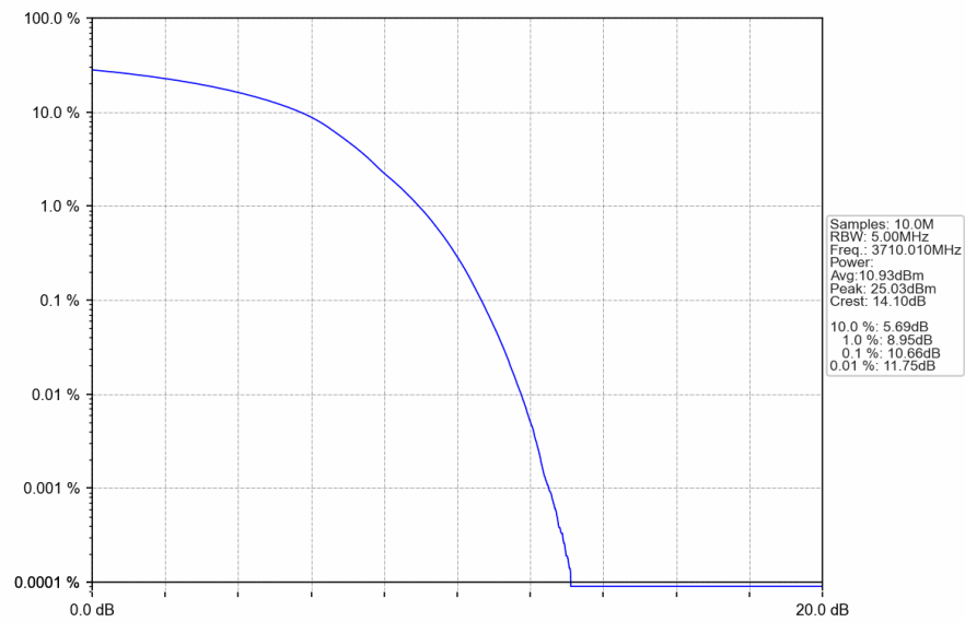
n78a_30kHz_SISO_NTNV_20MHz_DFT-s-OFDM_64_QAM_3710.01MHz_Outer_Full
