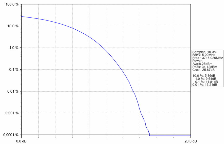
n78a 30kHz SISO NTN 30MHz CP-OFDM 64 QAM 3715.02MHz Outer Full
