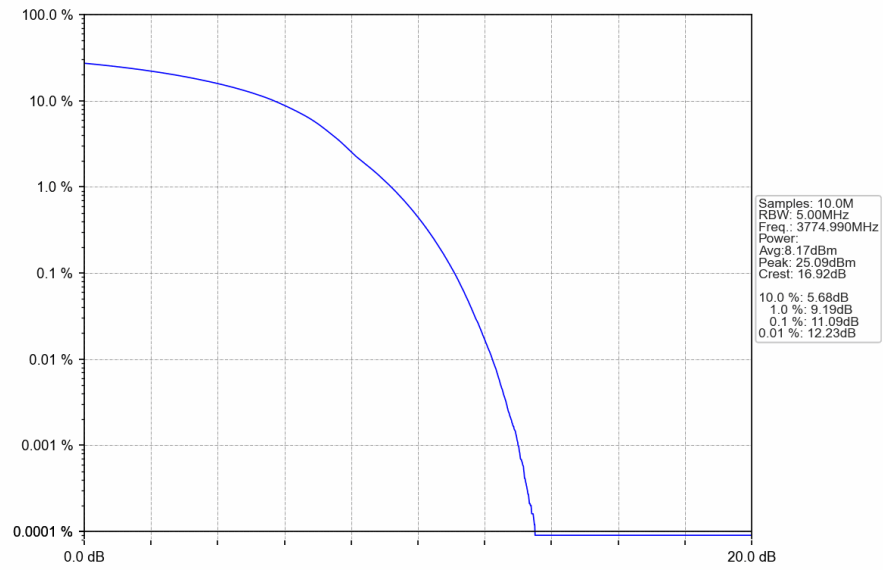
n78a_30kHz_SISO_NTNV_50MHz_DFT-s-OFDM_QPSK_3774.99MHz_Outer_Full
