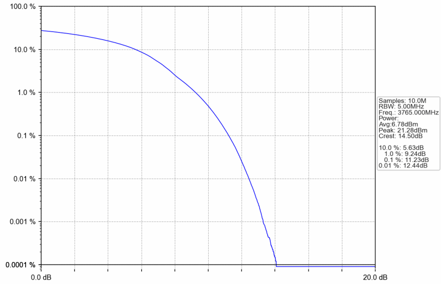
n78a_30kHz_SISO_NTNV_70MHz_DFT-s-OFDM_QPSK_3765MHz_Outer_Full
