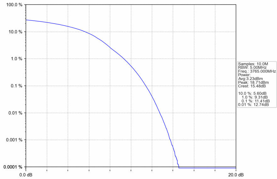
n78a_30kHz_SISO_NTNV_70MHz_DFT-s-OFDM_256_QAM_3765MHz_Outer_Full
