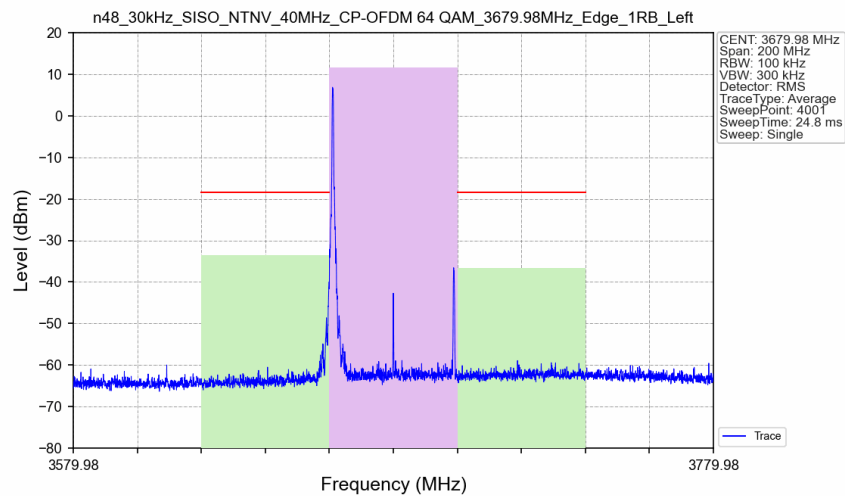
n48_30kHz_SISO_NTNV_40MHz_CP-OFDM 64 QAM_3679.98MHz_Edge_1RB_Left_Ant2
