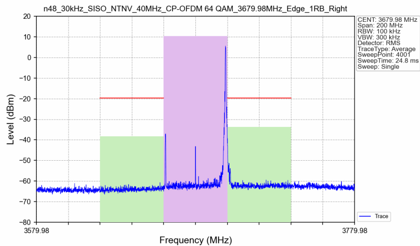
n48_30kHz_SISO_NTNV_40MHz_CP-OFDM 64 QAM_3679.98MHz_Edge_1RB_Right_Ant2
