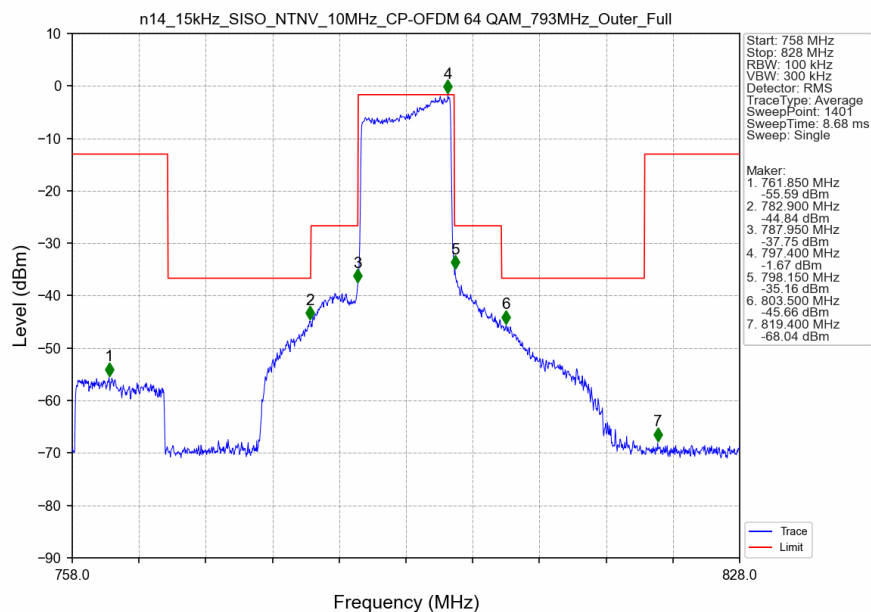
n14_15kHz_SISO_NTNV_10MHz_CP-OFDM 64 QAM_793MHz_Outer_Full_Ant0
