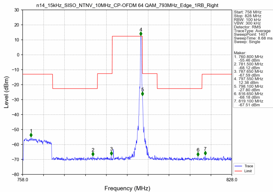
n14_15kHz_SISO_NTNV_10MHz_CP-OFDM 64 QAM_793MHz_Edge_1RB_Right_Ant0
