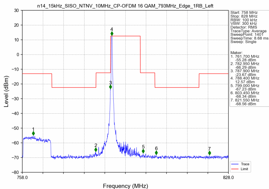
n14_15kHz_SISO_NTNV_10MHz_CP-OFDM 16 QAM_793MHz_Edge_1RB_Left_Ant0
