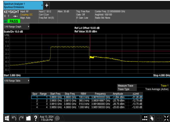
N77(50M)_CP- OFDM_QPSK_Outer_Full_High_CH
