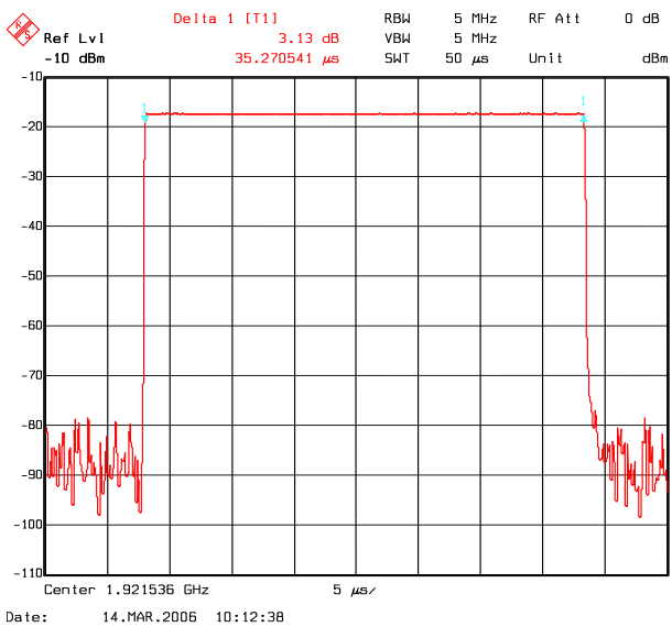
35 \mu s pulse
