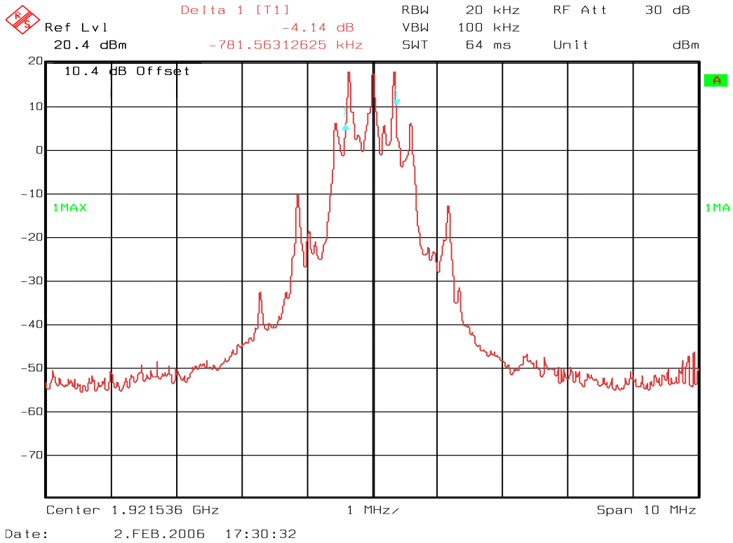
Conducted 6dB Bandwidth, ch 04
