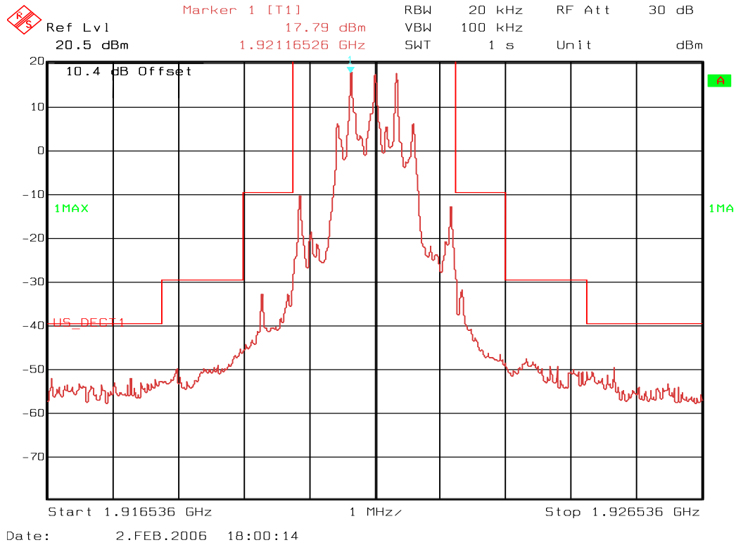
Conducted In-Band Emissions, Lower Channel
