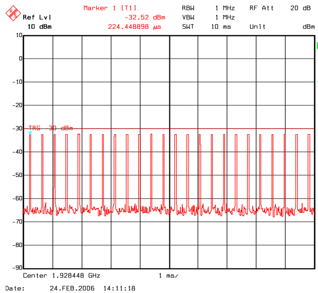
50 µs pulses synced to DECT frame
