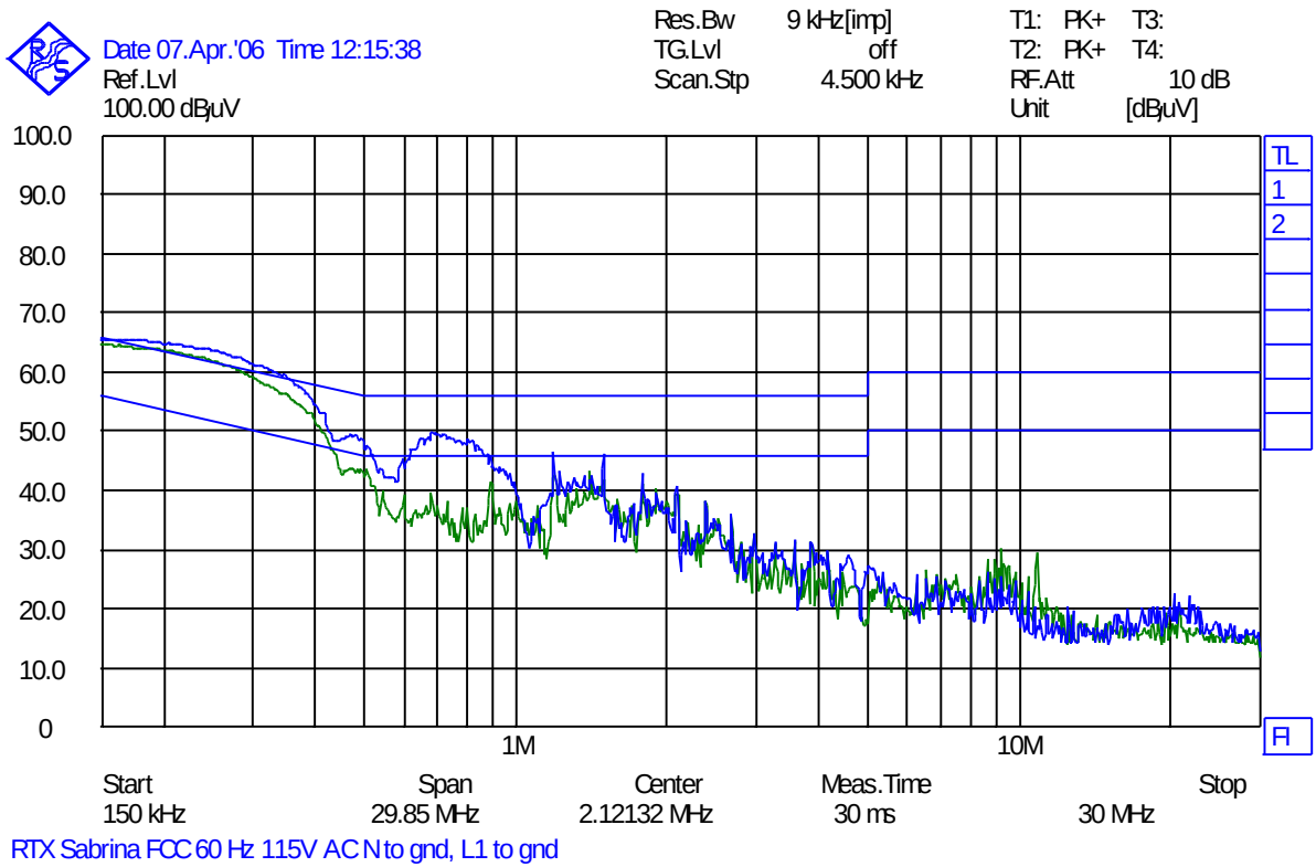
Conducted Emissions, Peak, N and L1
