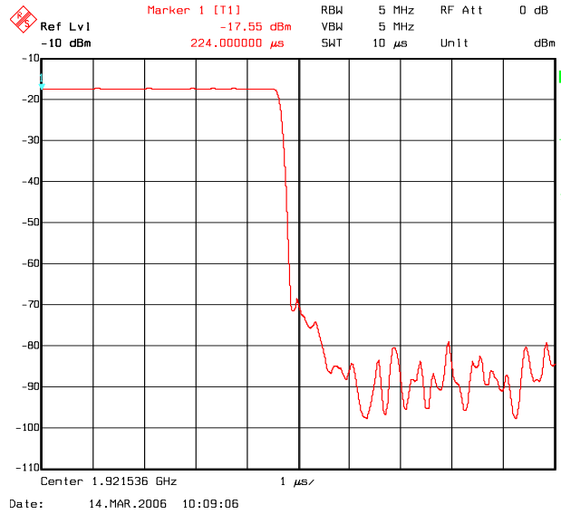
50 µs pulse, Fall Time
