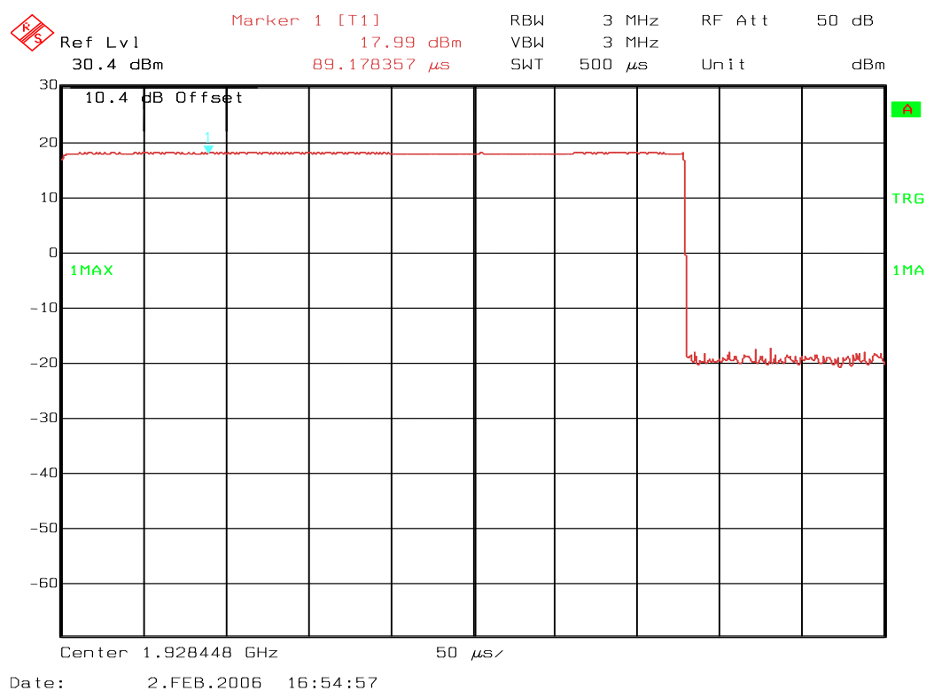
Conducted Peak Transmit Power, ch 00
