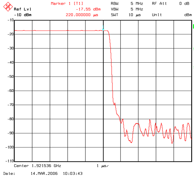
35 \mu s pulse, Fall Time
