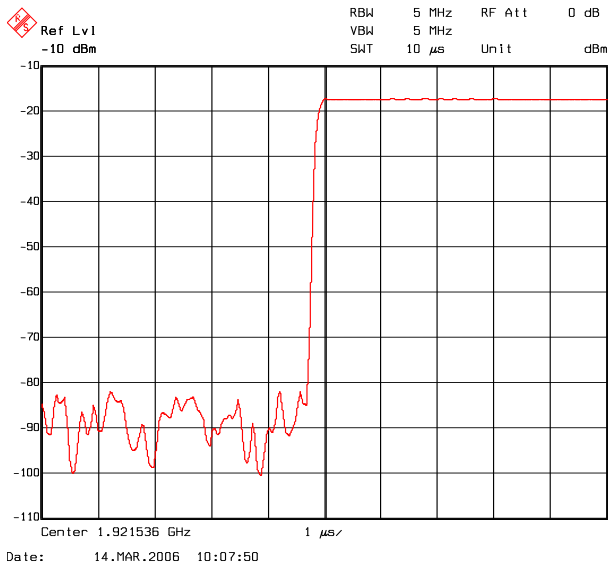
50 µs pulse, Rise Time
