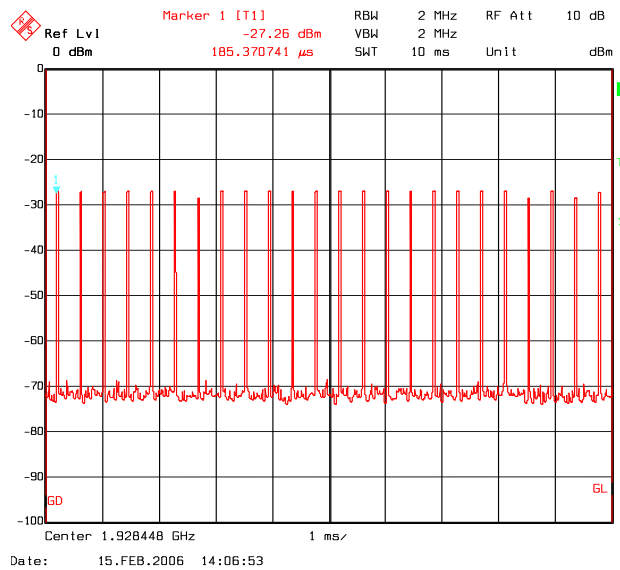
35 \mu s pulses synced to DECT frame
