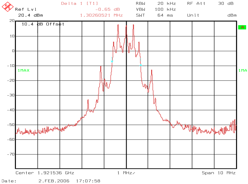
Conducted Emission Bandwidth B 26 dB, ch 04
