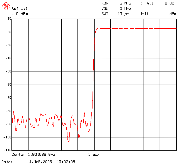
35 \mu s pulse, Rise Time
