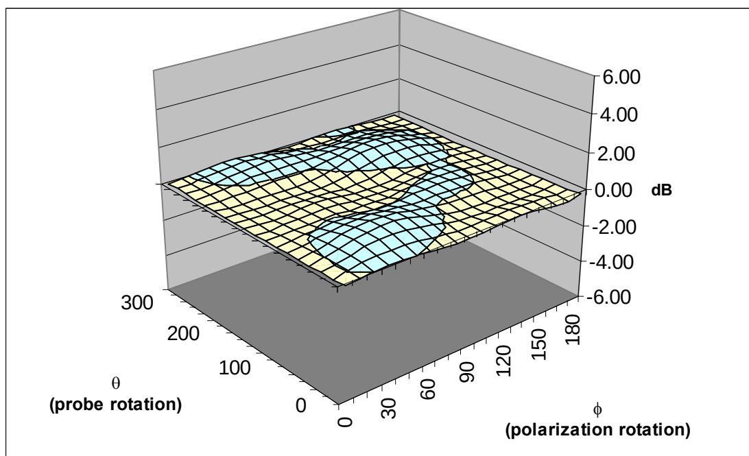
Surface Isotropy diagram of IXP-050 Probe S/N 0170 at 900MHz after VPM (rotational isotropy at side \pm 0.09 dB, spherical isotropy \pm 0.44 dB)
