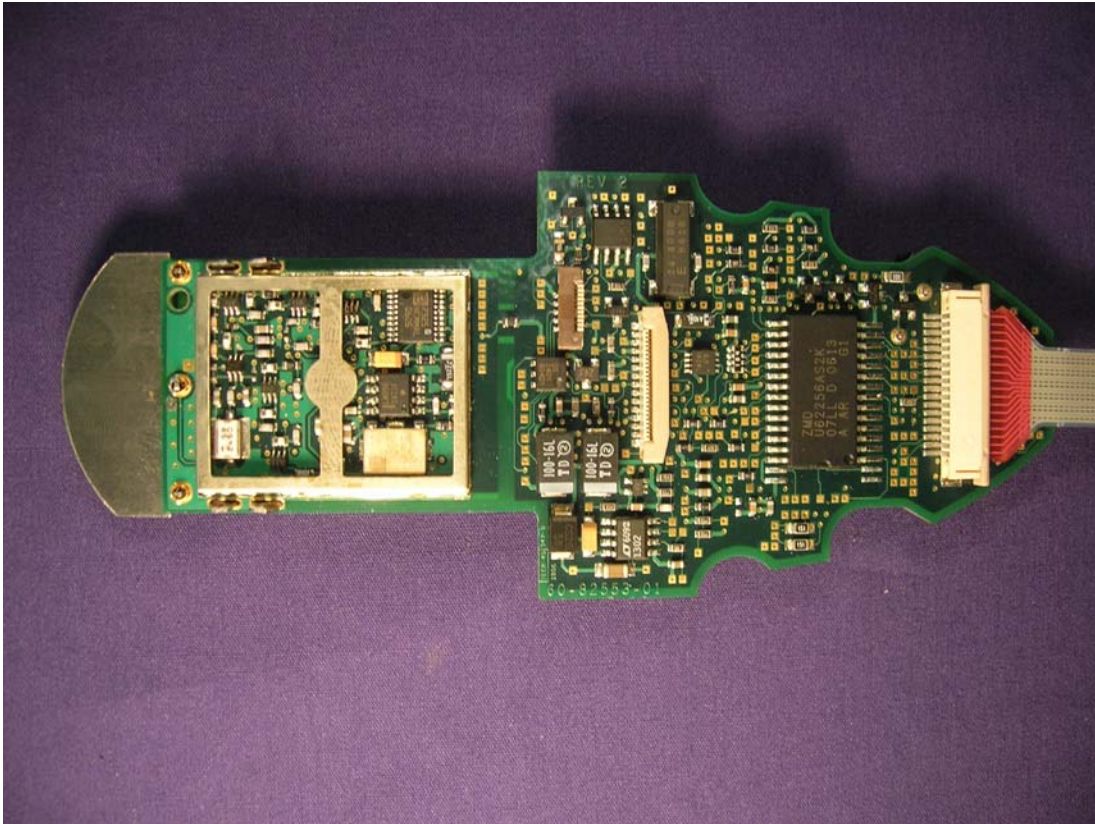
Top w/ RF Shield Removed
