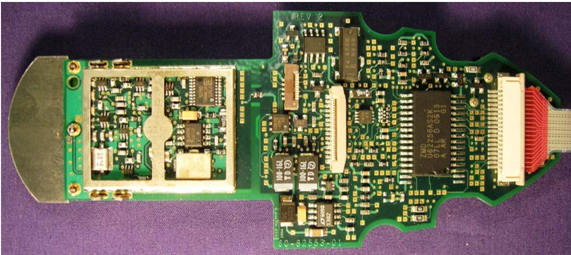
Top w/ RF Shield Removed
