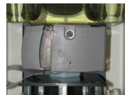
Figure 14.1 Body SAR Test Setup
