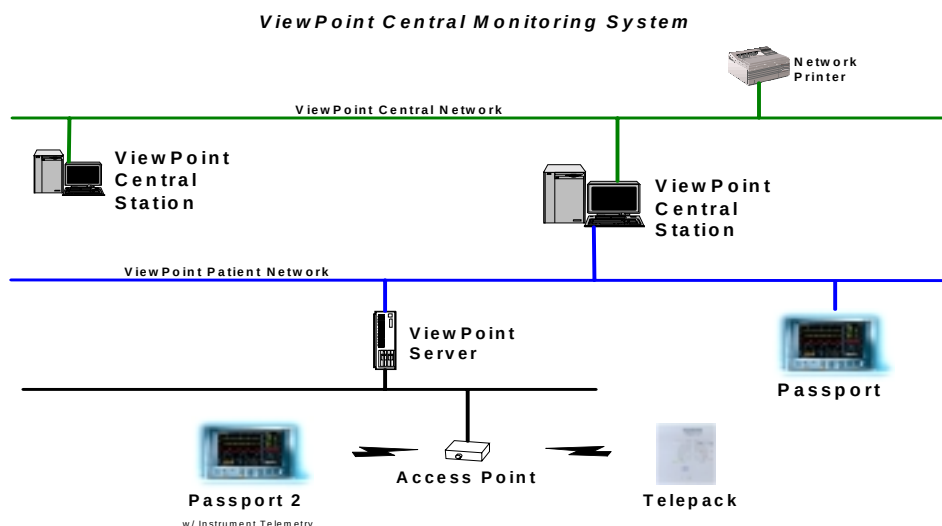
FIGURE 1-1 ViewPoint Central Monitoring System
