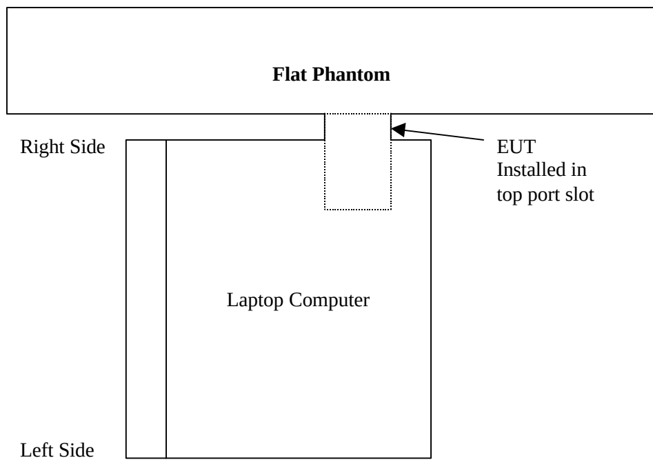
Figure 3: laptop in vertical position
