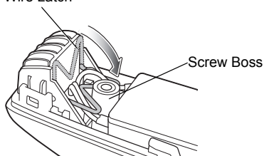
Wire Latch
