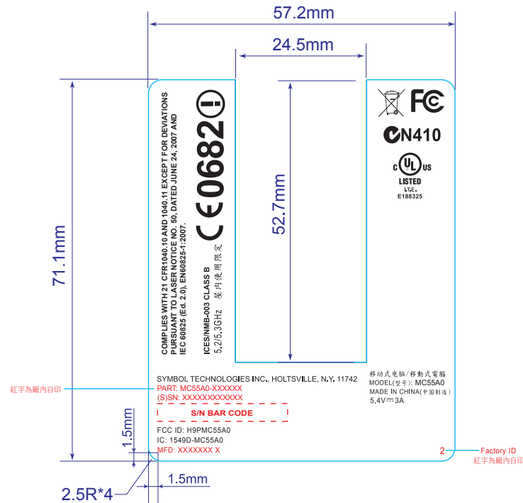
Joint-Regulatory Manufacturing Label (55A0)
