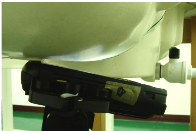
Right Tilted - DUT with Battery 2 + Scanner 2 + Keypad 1
