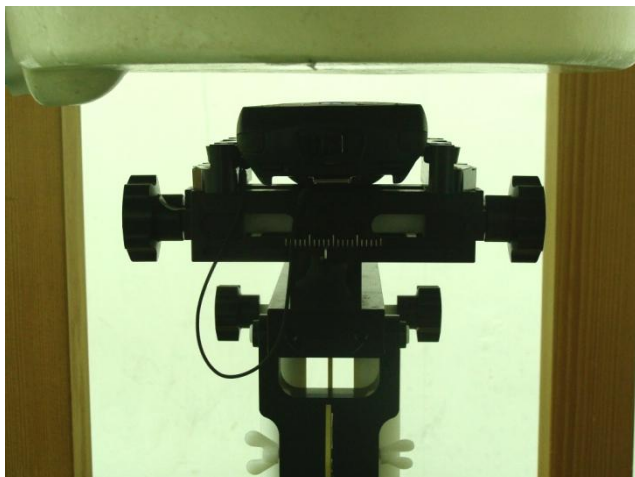
Face of the DUT with Battery 1 + Scanner 2 + Keypad 2 (with Phantom 1.5 cm Gap)
