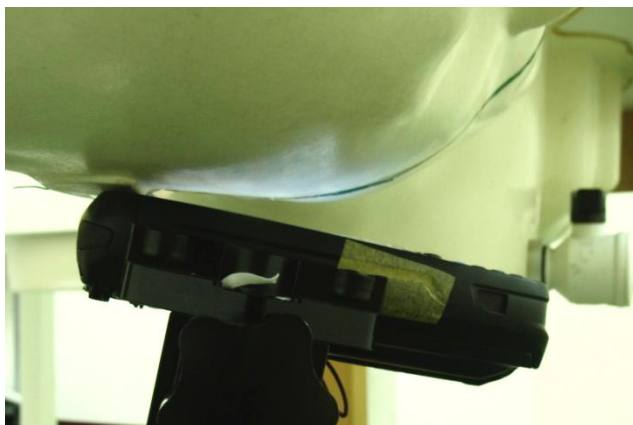
Right Tilted - DUT with Battery 2 + Scanner 2 + Keypad 3
