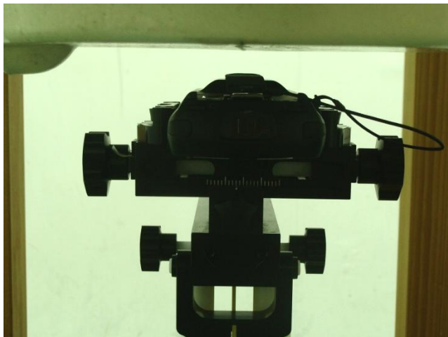
Bottom of the DUT with Battery 2 + Scanner 1 + Keypad 3 (with Phantom 1.5 cm Gap)
