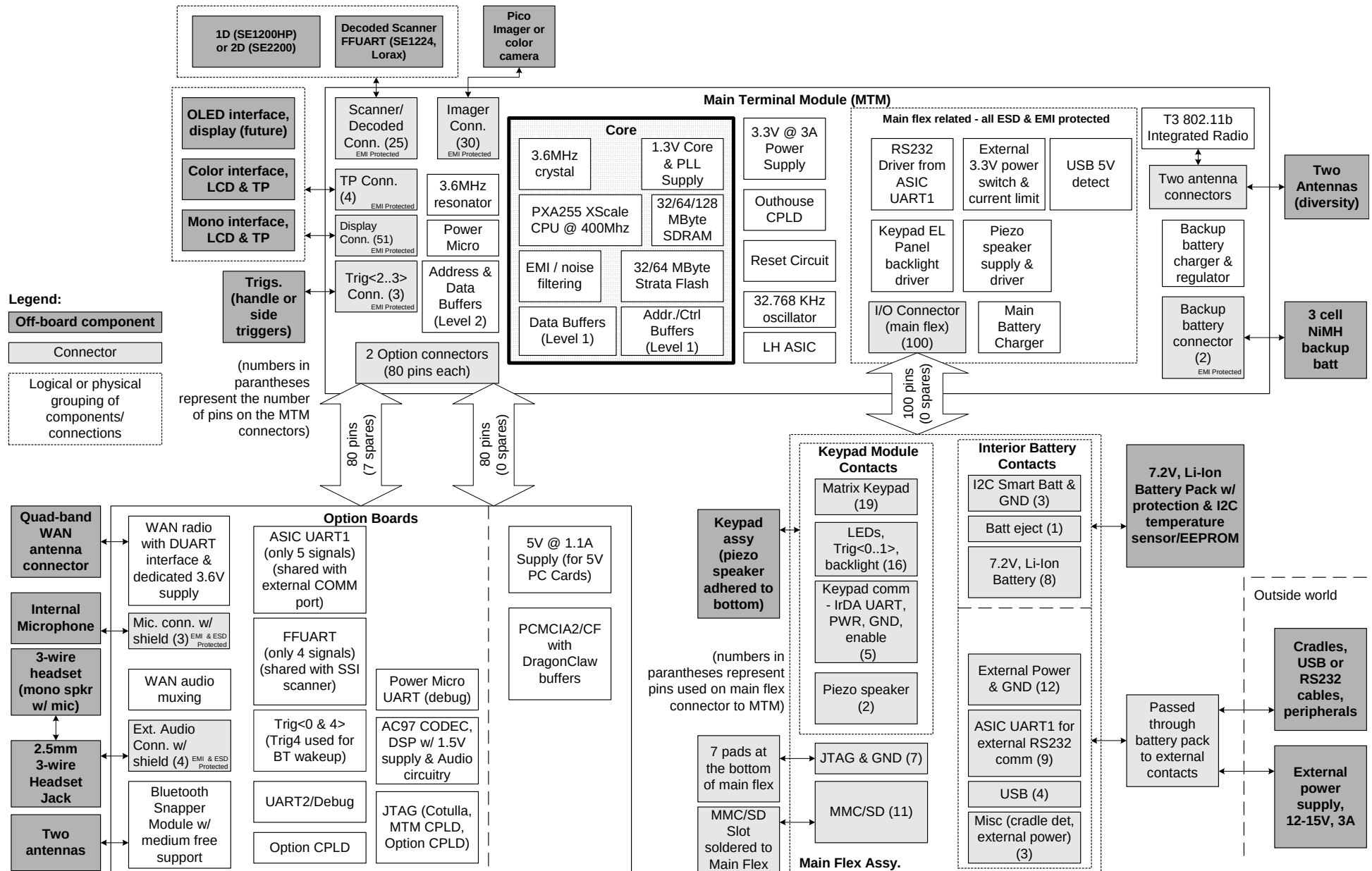
Figure 2.1: High Level MTM Block Diagram (Rev 15 from Visio)
