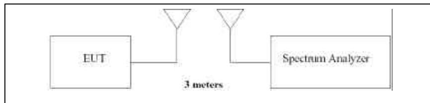
Figure A-3. Test Instrument & Measurement Setup
