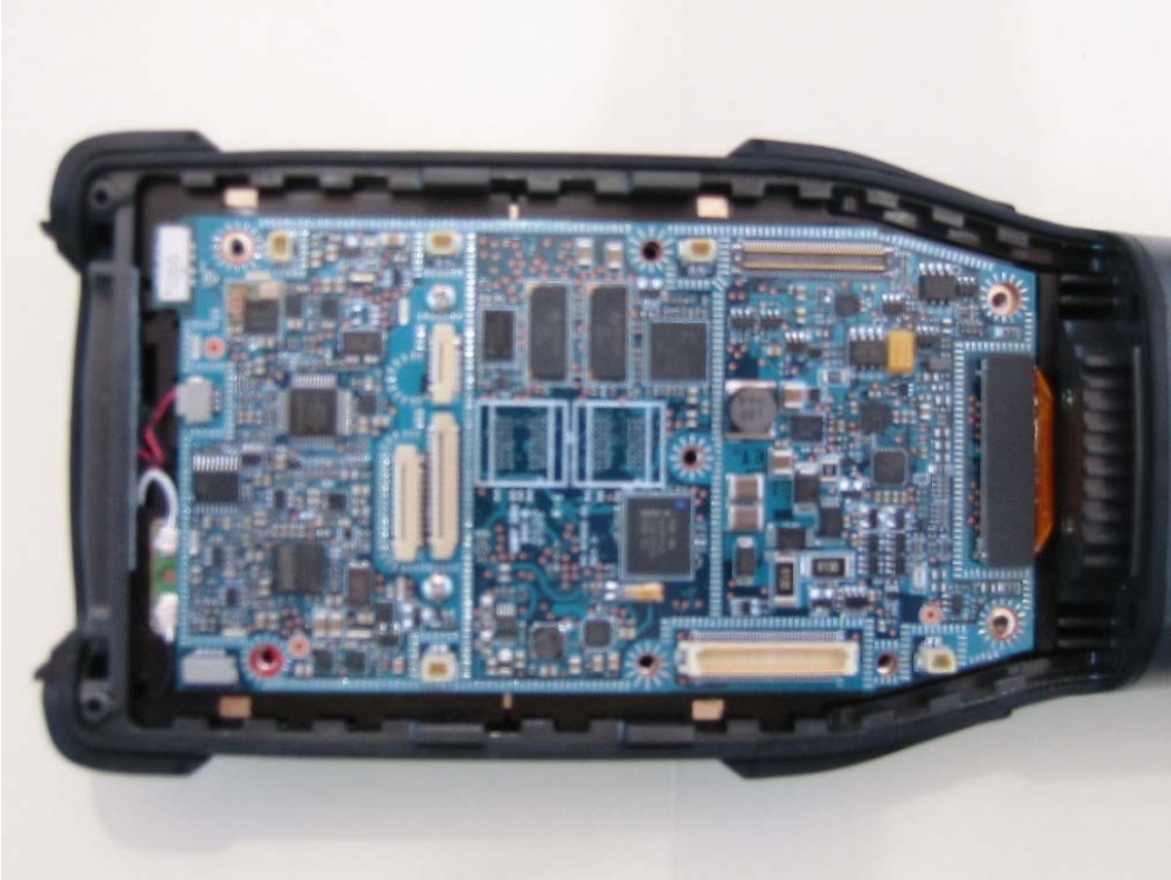
Main PCB board under iDEN carrier board assy
