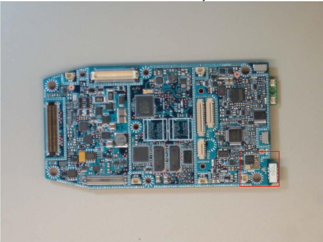
Bluetooth chip radio and antenna shown in red square
