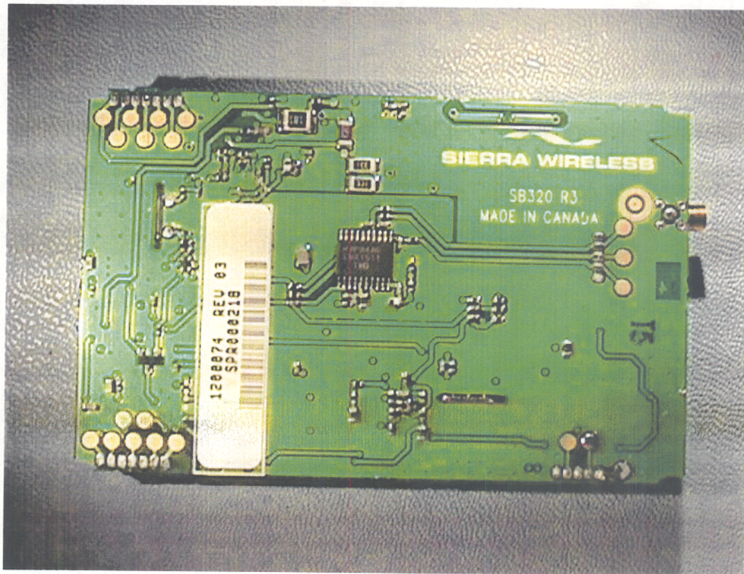
Figure4:ModemInternalView–RadioBoardBottomSide
